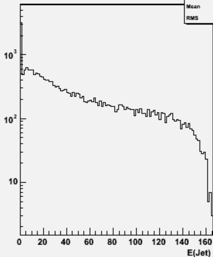
Jet energies(All jets)w102219 n2n2e1e1e3e3_o
