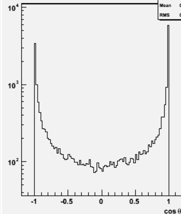
Jet cos \theta (All jets)w102219 n2n2e1e1e3e3_o
