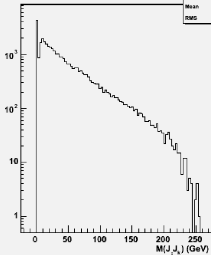
2jets mass(All comb)w102219 n2n2e1e1e3e3_o
