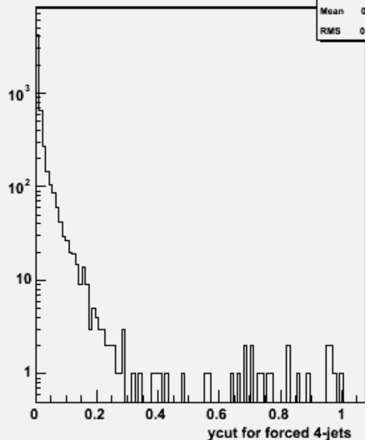
Ycut for 4-jets :w102219 n2n2e1e1e3e3_o
