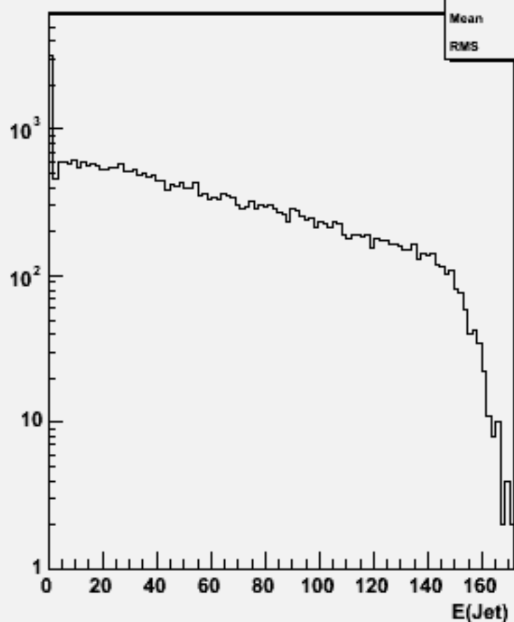
Jet energies(All jets)w102217 n2n2e1e1e1e1_o
