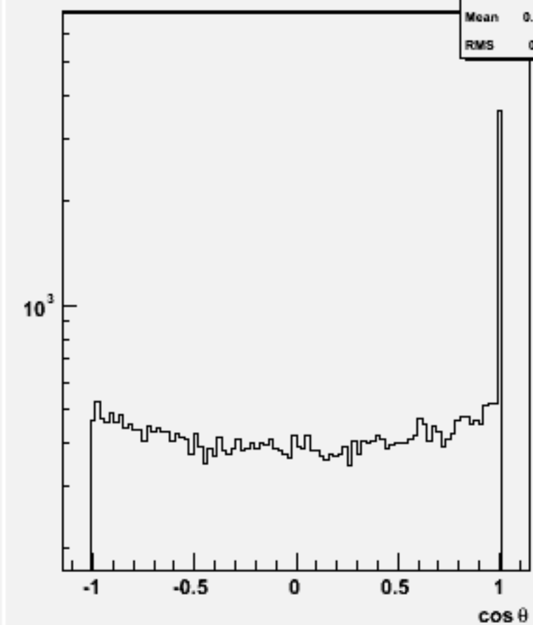
Jet cos \theta (All jets)w102209 n1n1ssbb_o
