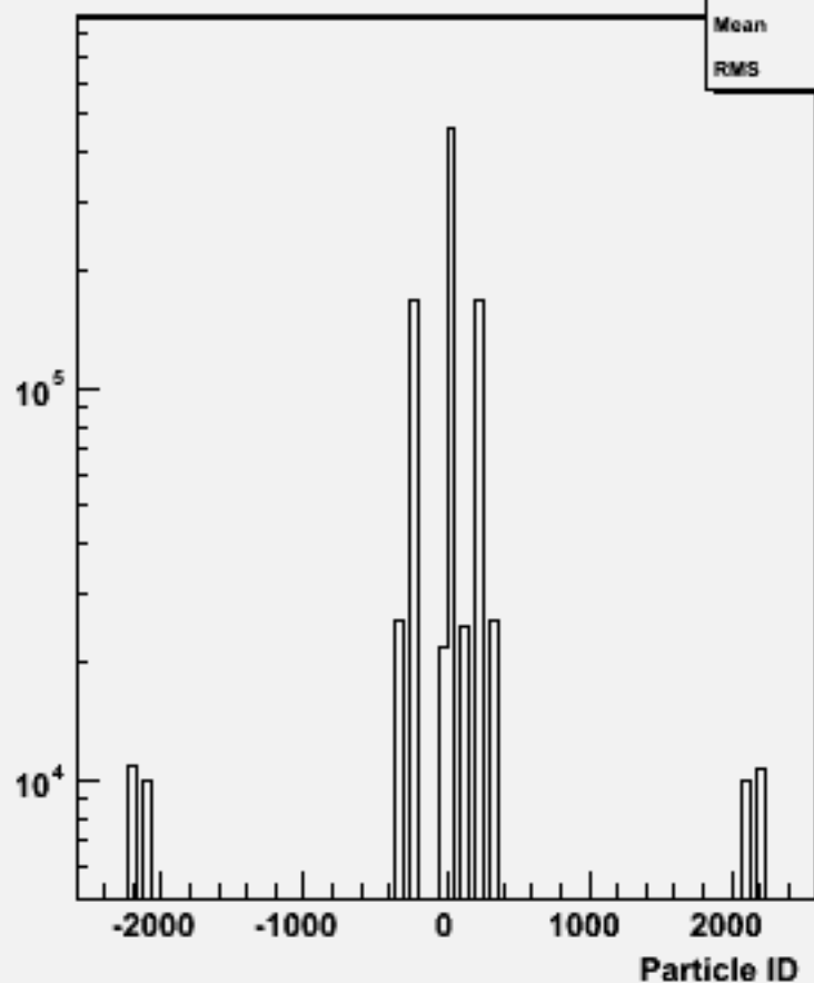
Particle ID : w102209 n1n1ssbb_o
