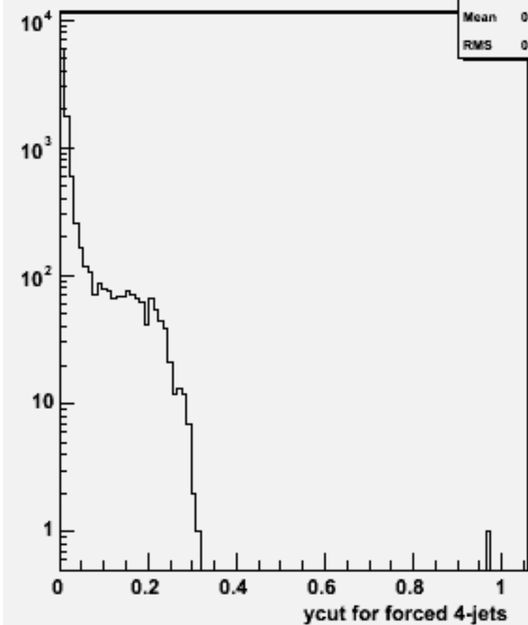
Ycut for 4-jets :w102209 n1n1ssbb_o
