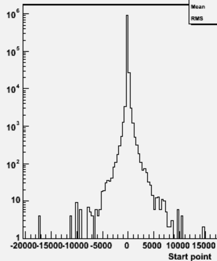
Start point Z : w102209 n1n1ssbb_o
