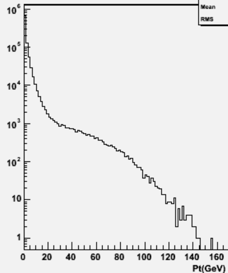
Particle Pt : w102209 n1n1ssbb_o
