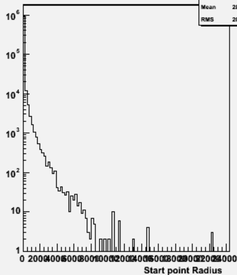
Start point R : w102209 n1n1ssbb_o
