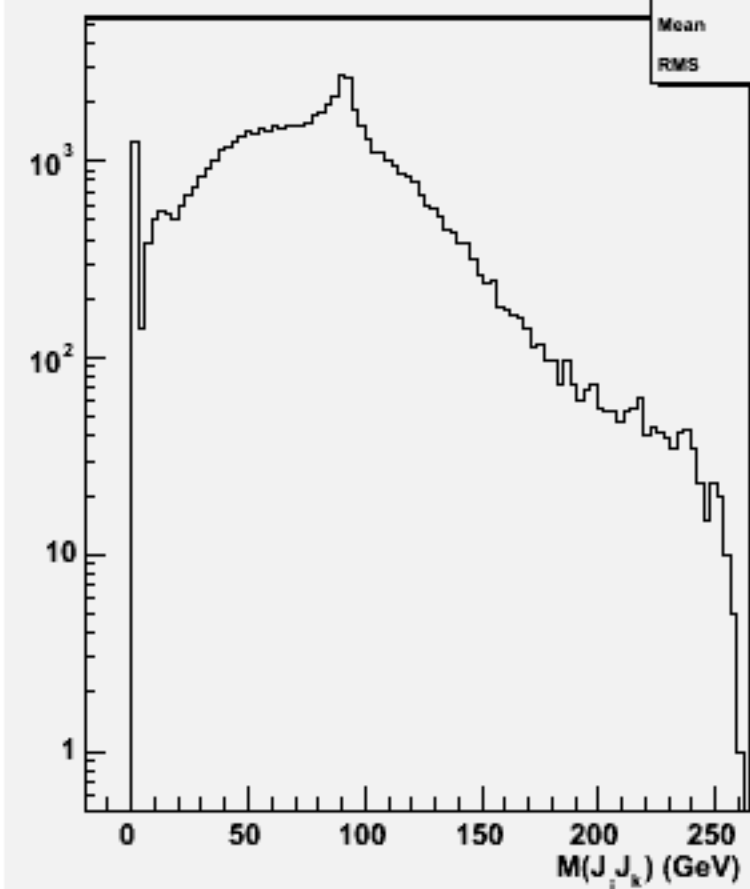
2jets mass(All comb)w102209 n1n1ssbb_o
