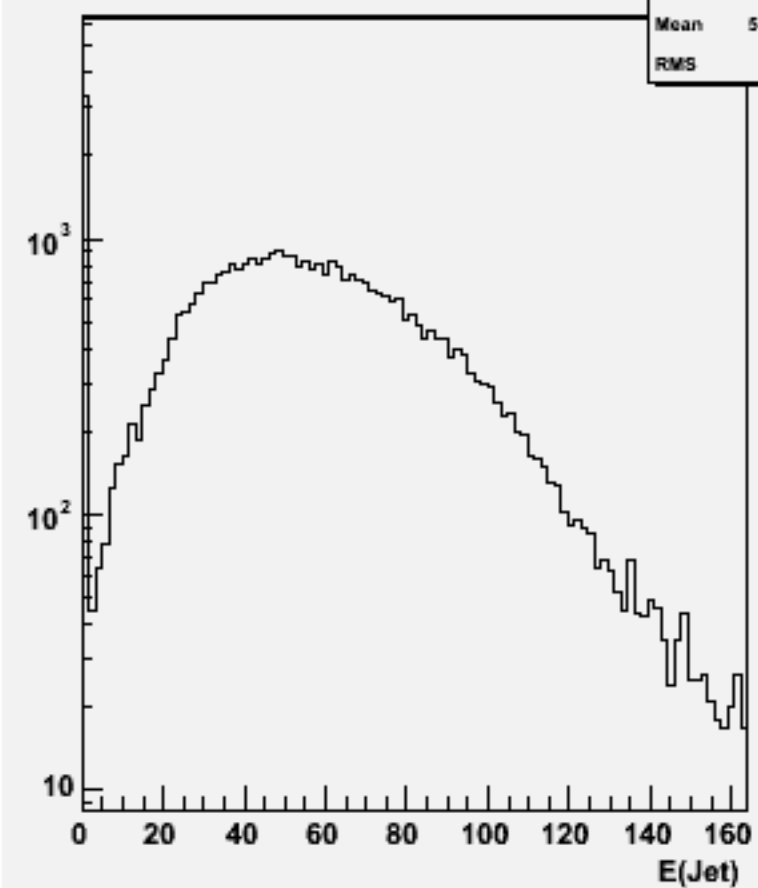
Jet energies(All jets)w102209 n1n1ssbb_o
