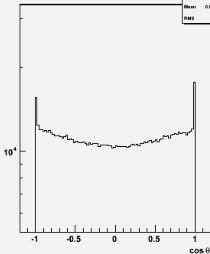
Particle cos \theta : w102209 n1n1ssbb_o
