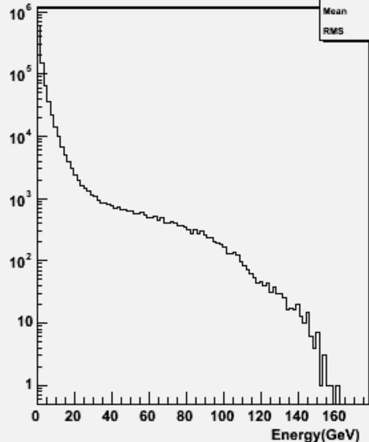
Particle Energy : w102209 n1n1ssbb_o
