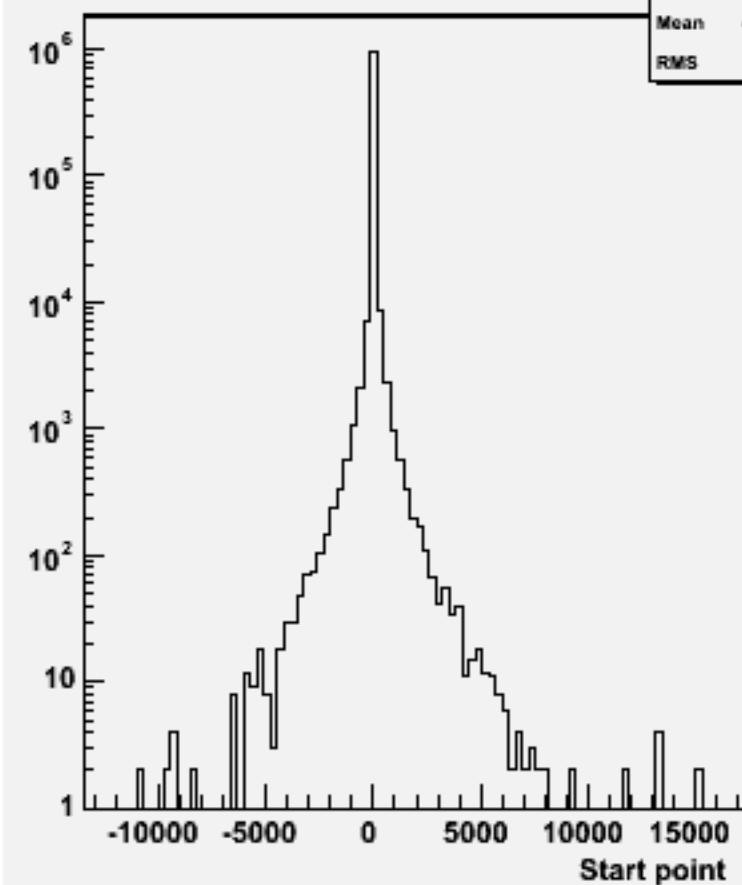
Start point Z : w102208 n1n1ssbb_o
