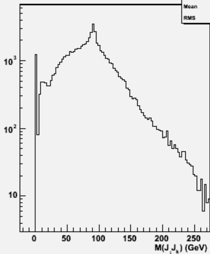
2jets mass(All comb)w102208 n1n1ssbb_o
