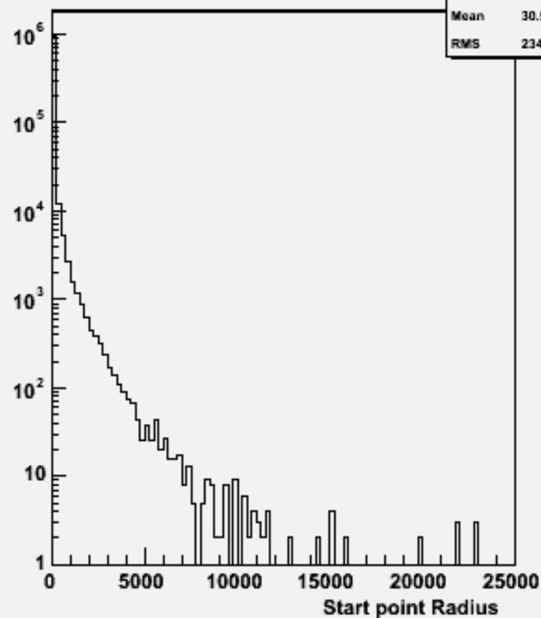
Start point R : w102208 n1n1ssbb_o
