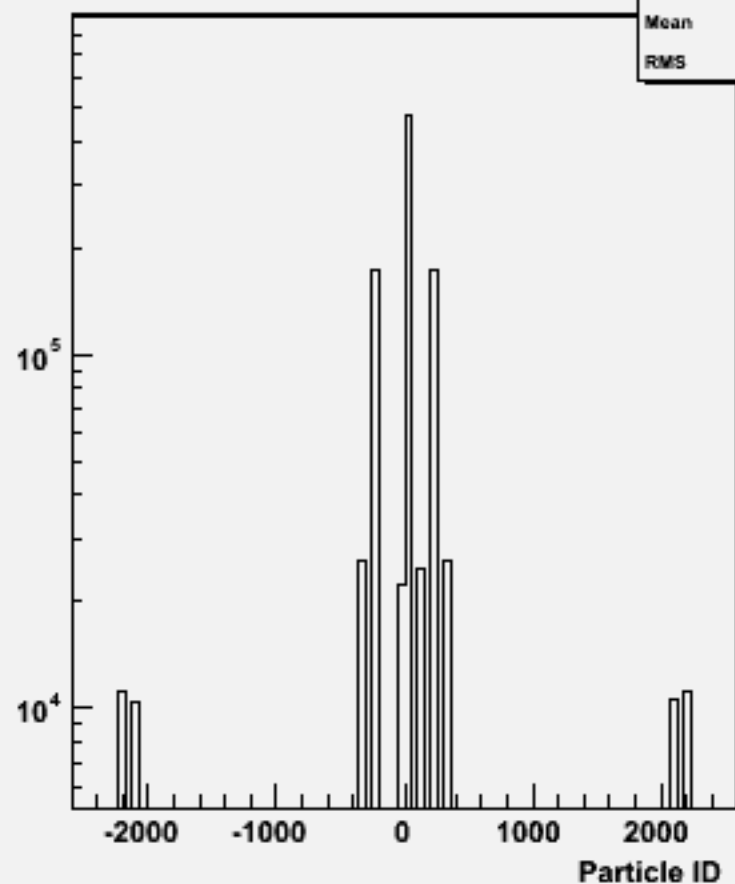
Particle ID : w102208 n1n1ssbb_o
