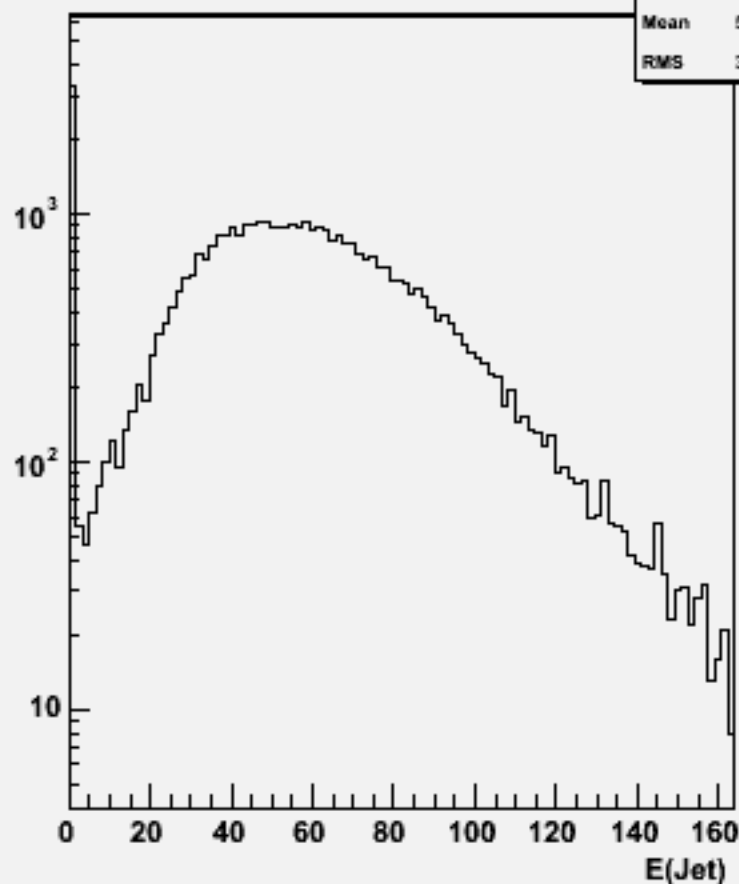
Jet energies(All jets)w102208 n1n1ssbb_o
