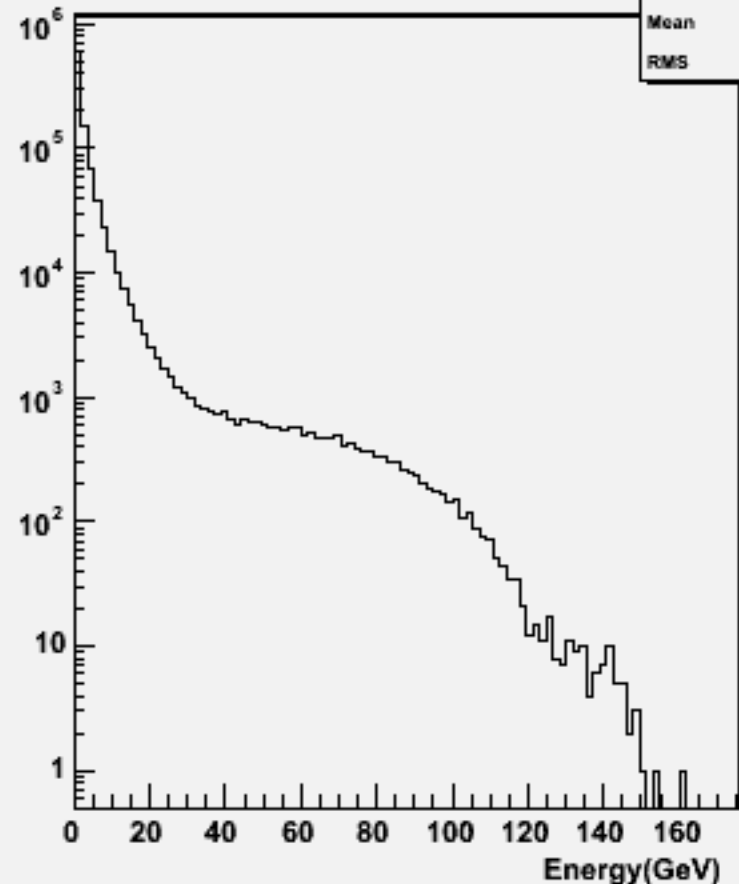
Particle Energy : w102208 n1n1ssbb_o
