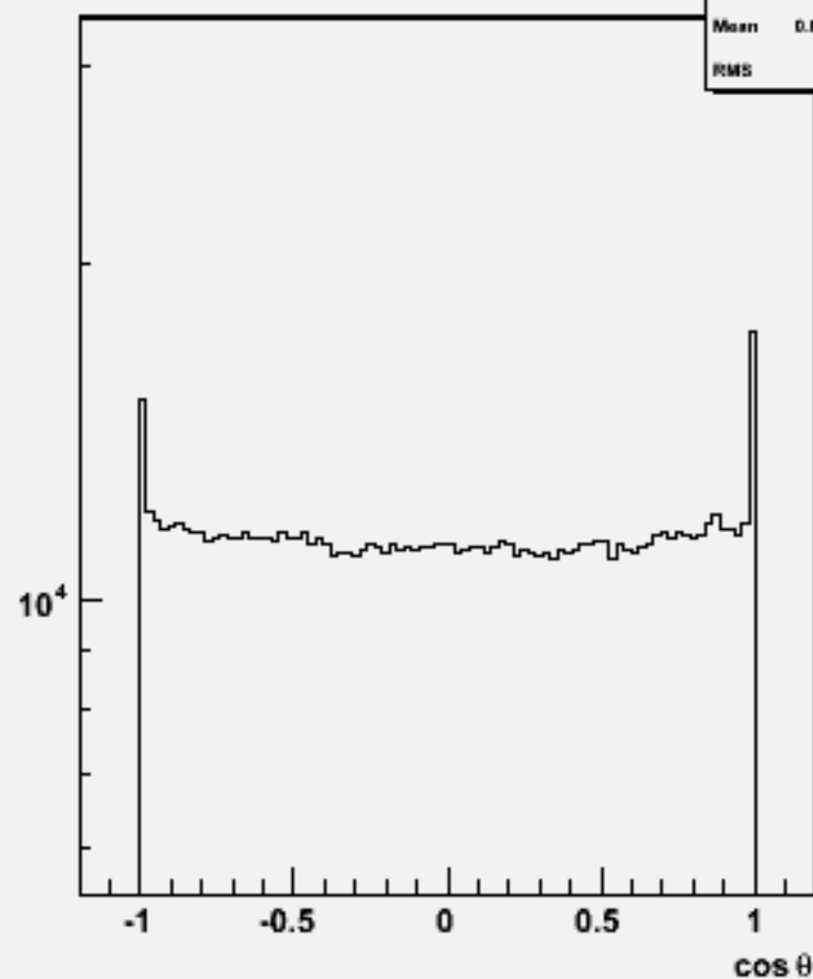
Particle cos \theta : w102208 n1n1ssbb_o
