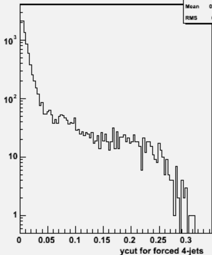
Ycut for 4-jets :w102208 n1n1ssbb_o
