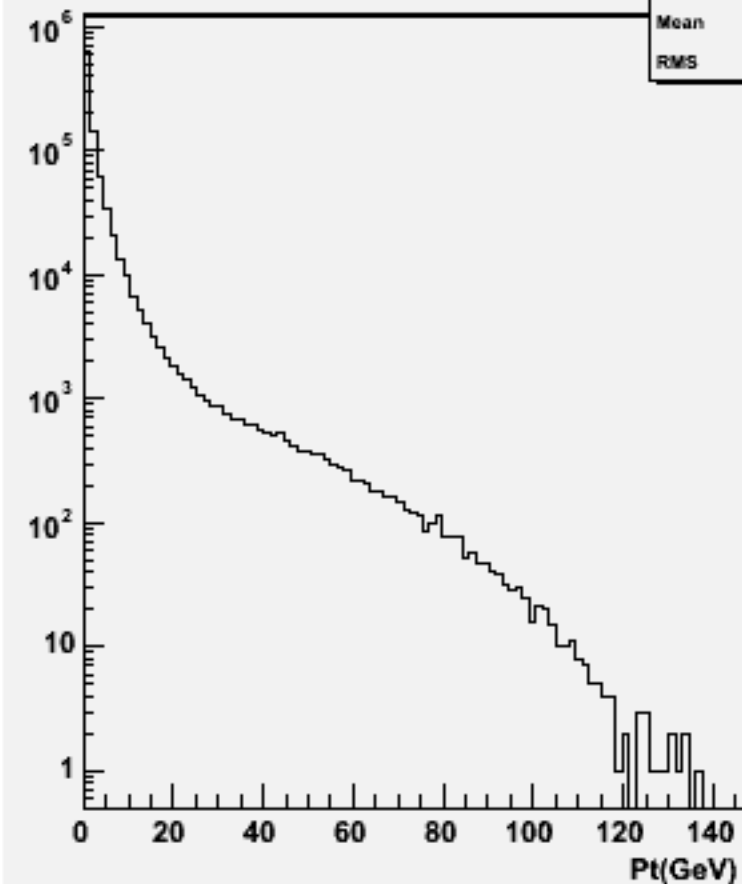
Particle Pt : w102208 n1n1ssbb_o
