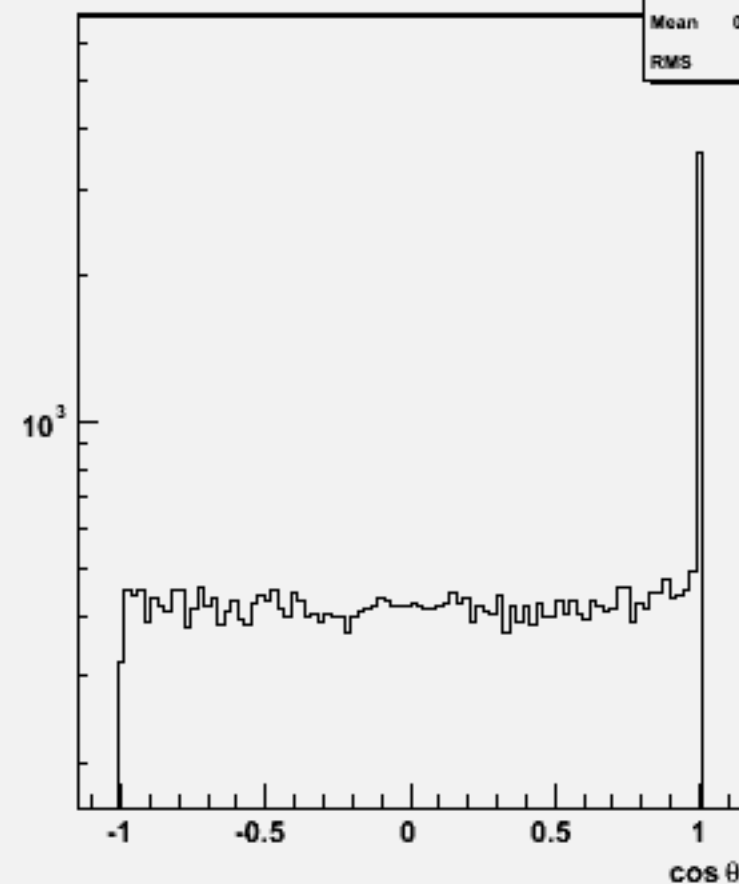
Jet cos \theta (All jets)w102208 n1n1ssbb_o
