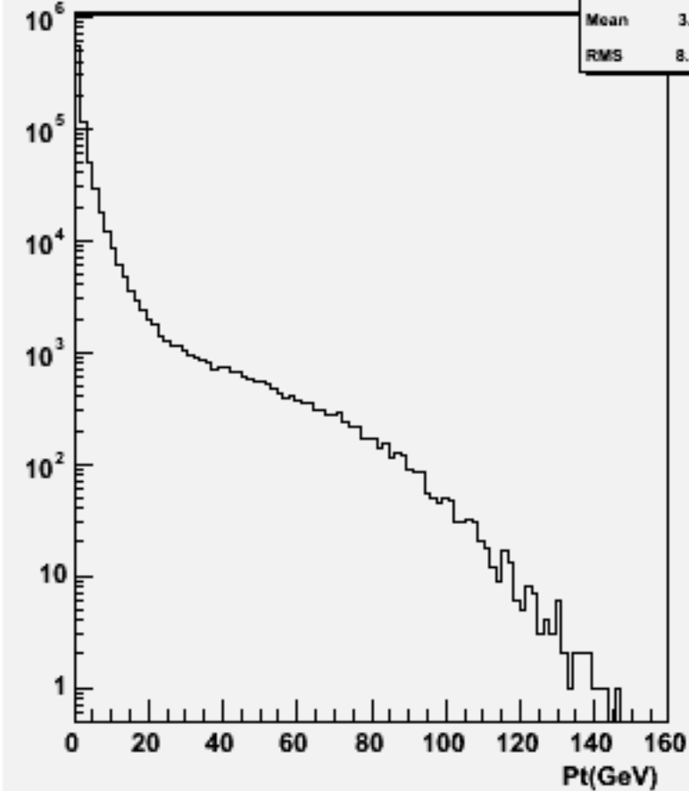
Particle Pt : w102205 n1n1ssss_o
