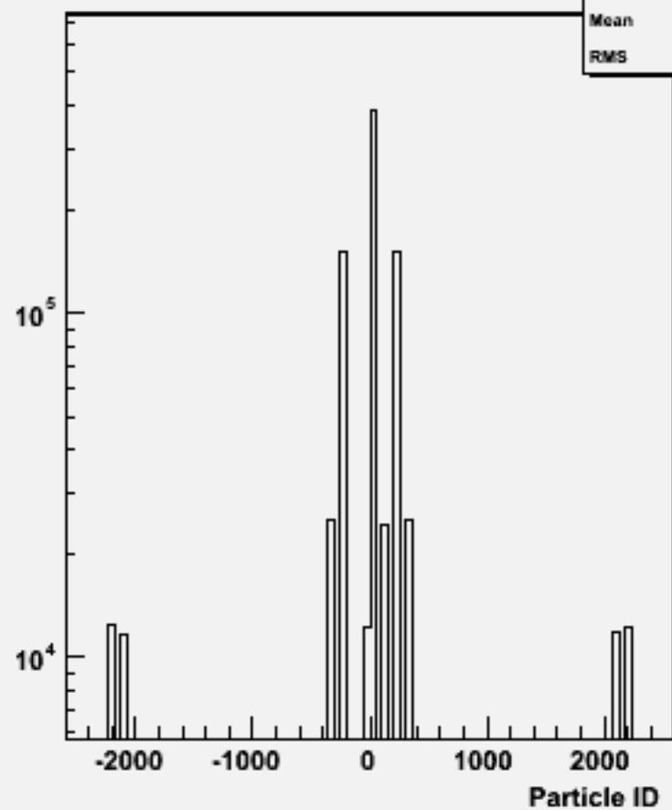
Particle ID : w102205 n1n1ssss_o
