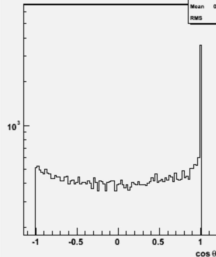
Jet cosθ (All jets)w102205 n1n1ssss_o
