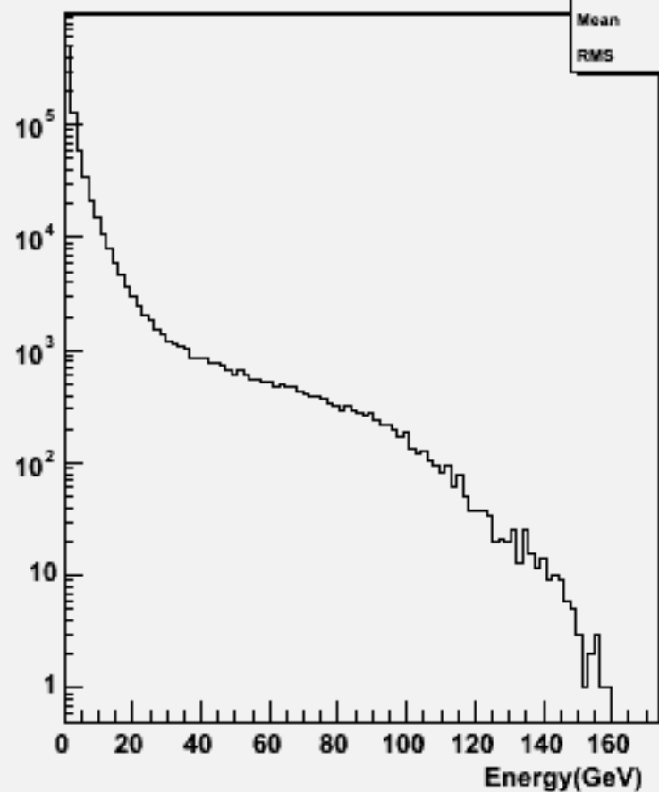
Particle Energy : w102205 n1n1ssss_o
