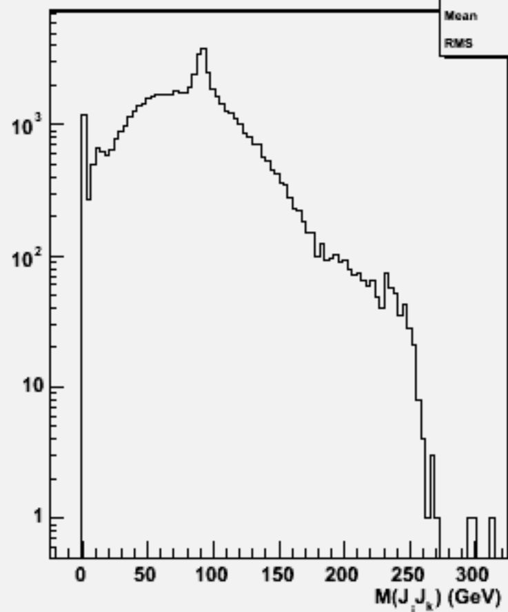
2jets mass(All comb)w102205 n1n1ssss_o
