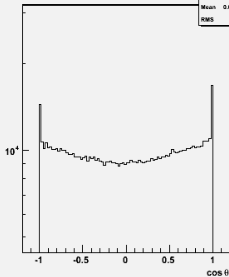
Particle cos \theta : w102205 n1n1ssss_o
