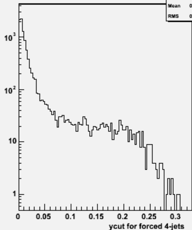
Ycut for 4-jets :w102205 n1n1ssss_o
