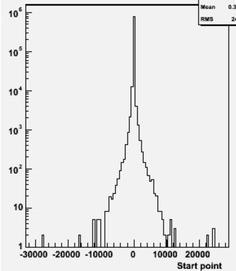
Start point Z : w102205 n1n1ssss_o
