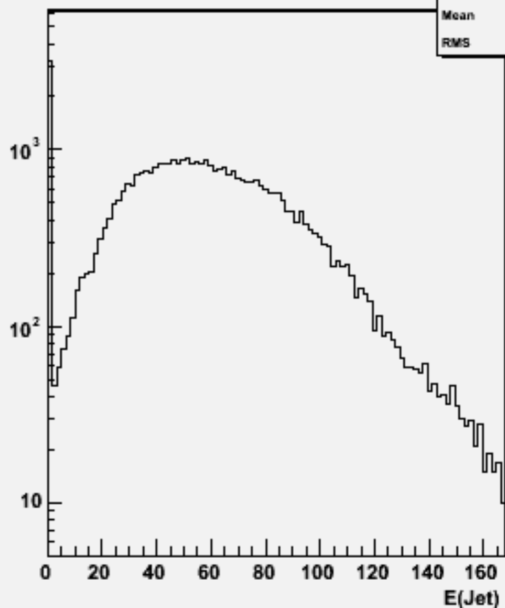
Jet energies(All jets)w102205 n1n1ssss_o
