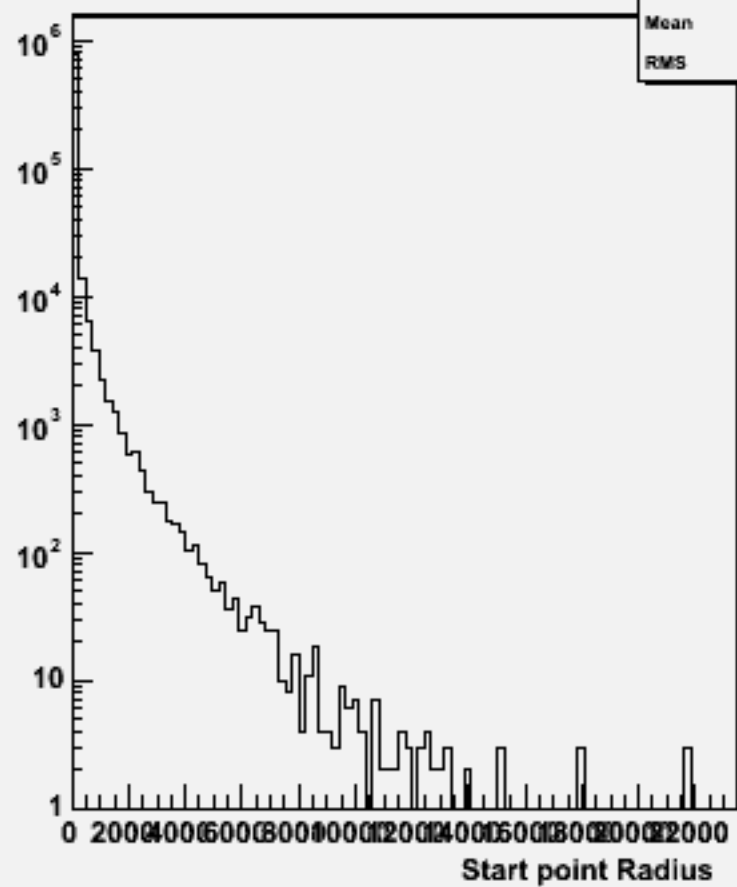
Start point R : w102205 n1n1ssss_o
