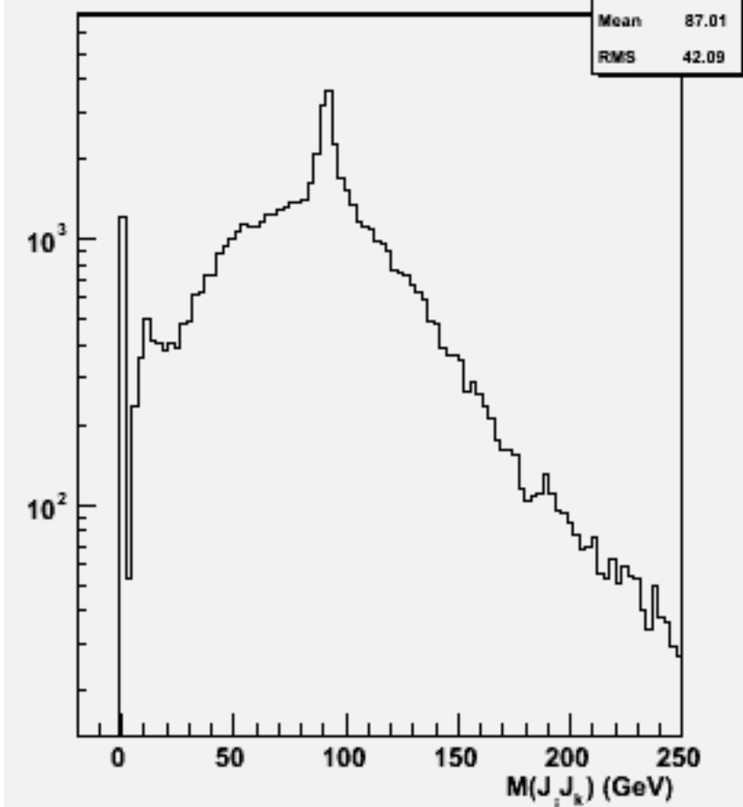
2jets mass(All comb)w102204 n1n1ssss_o
