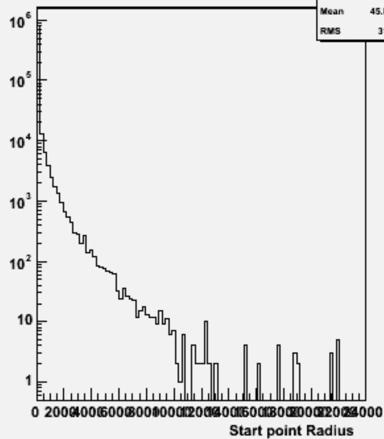
Start point R : w102204 n1n1ssss_o
