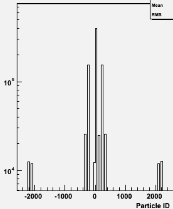
Particle ID : w102204 n1n1ssss_o
