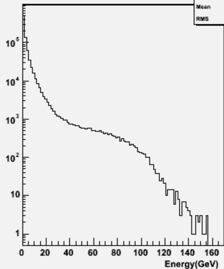
Particle Energy : w102204 n1n1ssss_o
