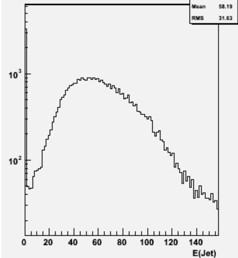
Jet energies(All jets)w102204 n1n1ssss_o
