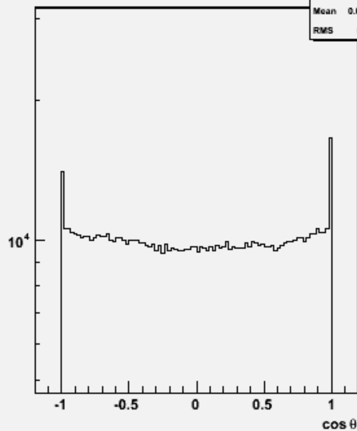
Particle cos \theta : w102204 n1n1ssss_o
