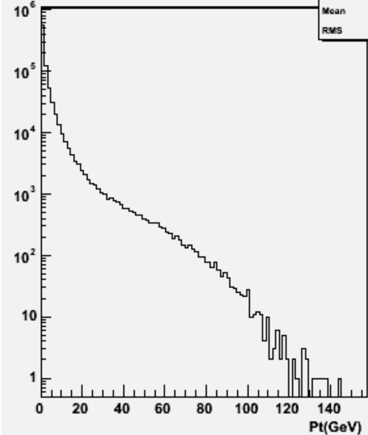
Particle Pt : w102204 n1n1ssss_o
