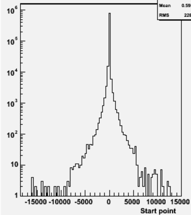
Start point Z : w102204 n1n1ssss_o
