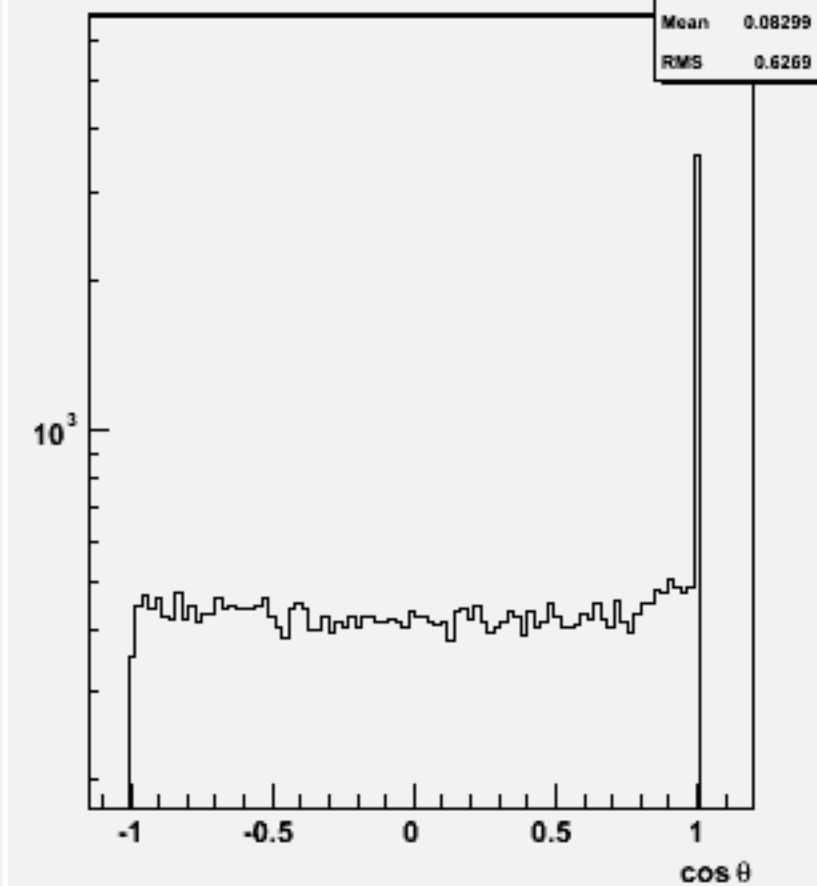
Jet cos \theta (All jets)w102204 n1n1ssss_o
