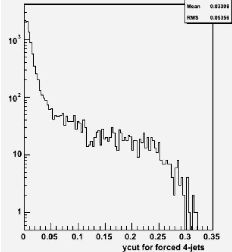
Ycut for 4-jets :w102204 n1n1ssss_o
