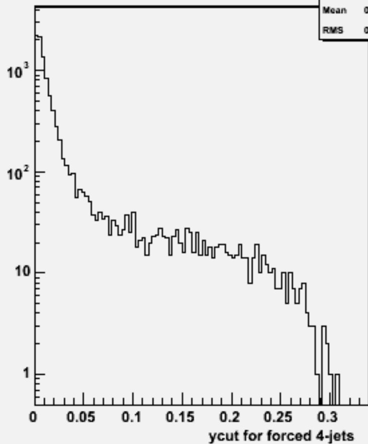
Ycut for 4-jets :w102201 n1n1ddb_o
