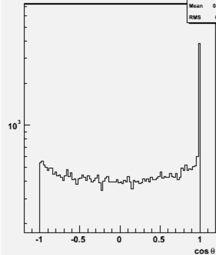
Jet cosθ (All jets)w102201 n1n1ddb_o
