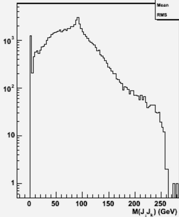
2jets mass(All comb)w102201 n1n1ddb_o
