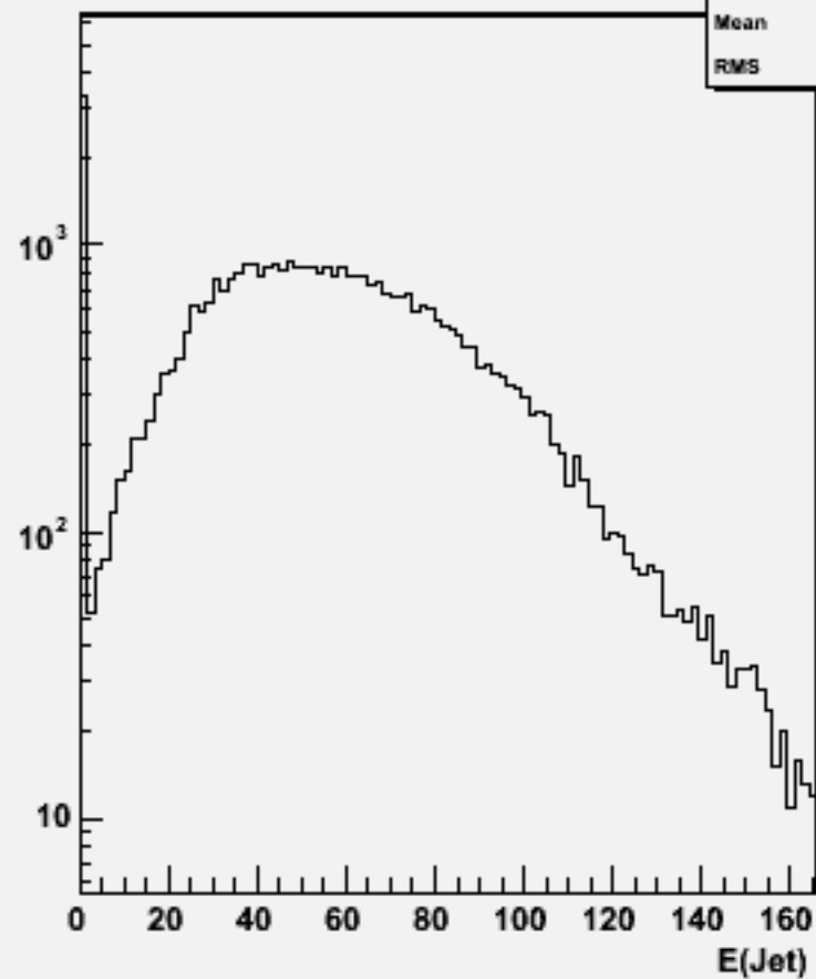
Jet energies(All jets)w102201 n1n1ddb_o
