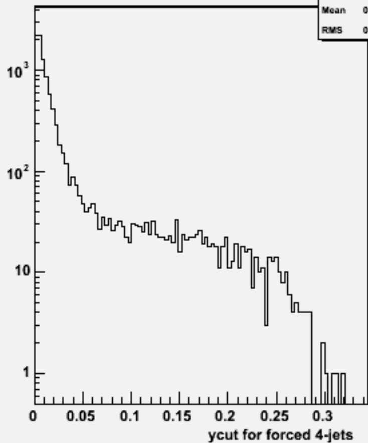
Ycut for 4-jets :w102197 n1n1ddss_o
