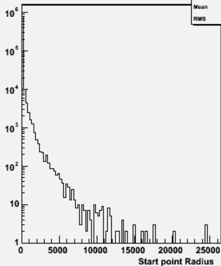
Start point R : w102197 n1n1ddss_o
