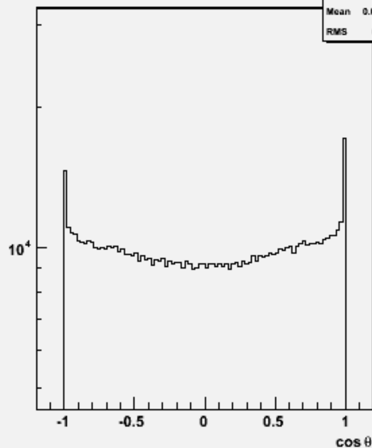
Particle cos \theta : w102197 n1n1ddss_o
