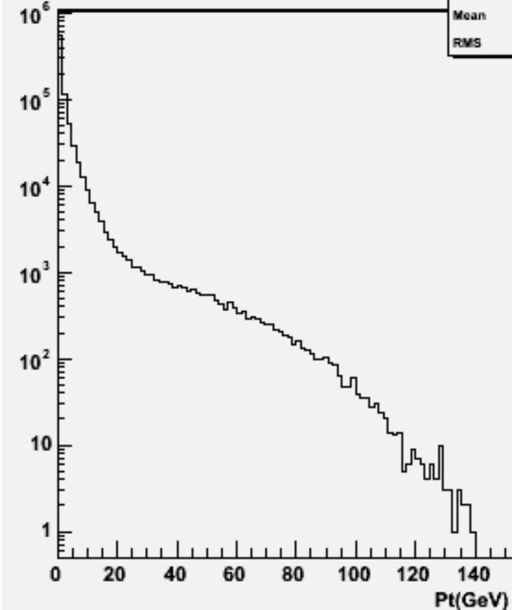
Particle Pt : w102197 n1n1ddss_o
