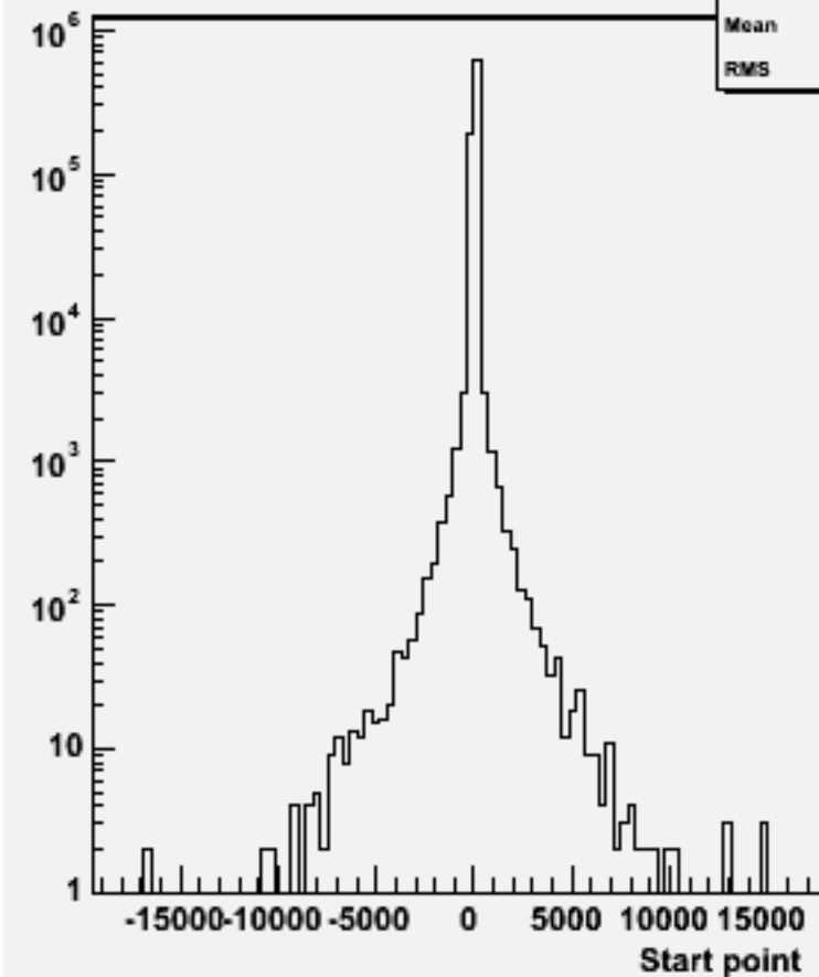
Start point Z : w102197 n1n1ddss_o
