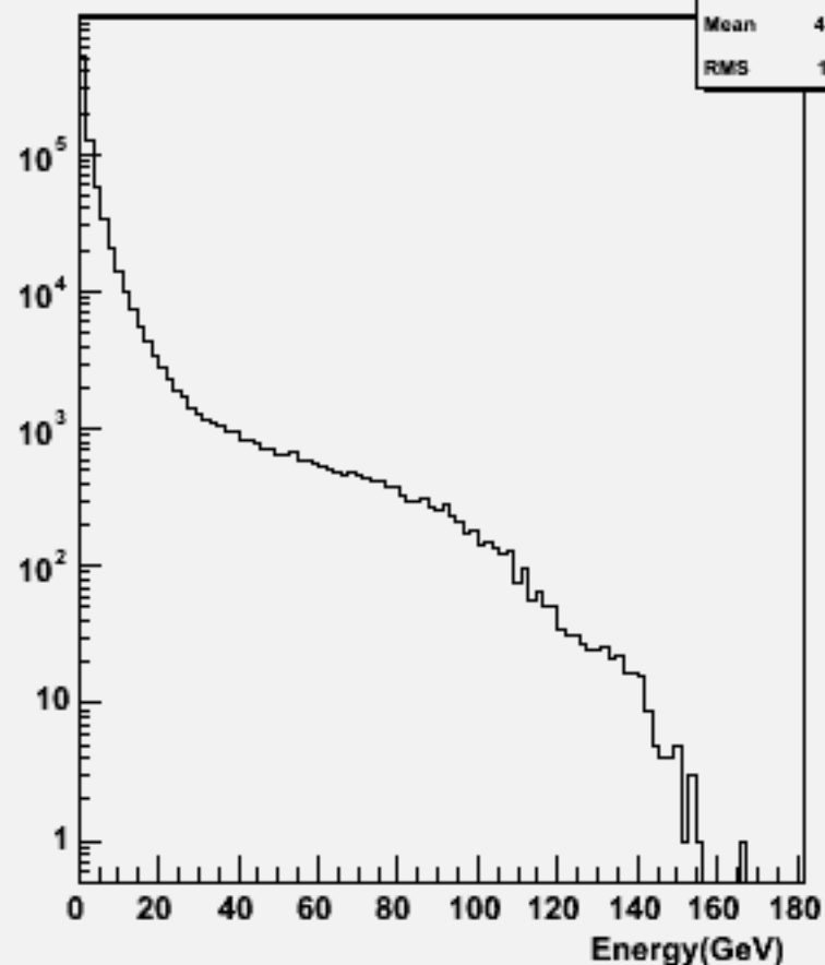
Particle Energy : w102197 n1n1ddss_o
