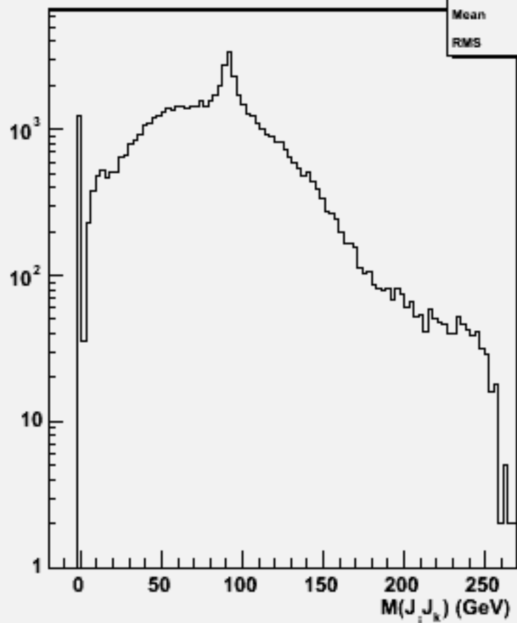
2jets mass(All comb)w102197 n1n1ddss_o
