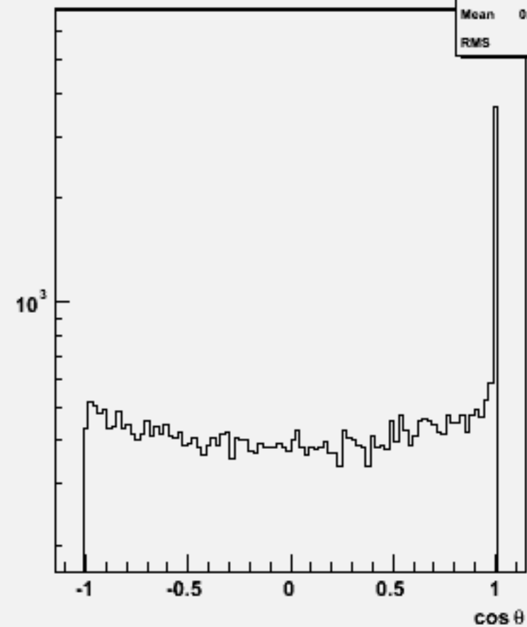
Jet cos \theta (All jets)w102197 n1n1ddss_o
