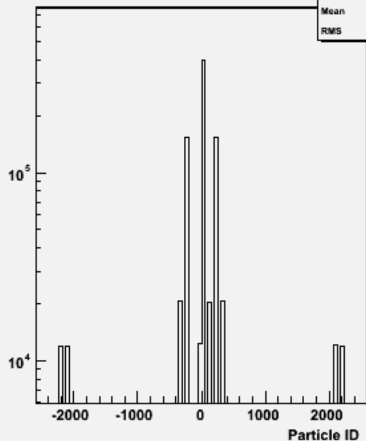
Particle ID : w102197 n1n1ddss_o
