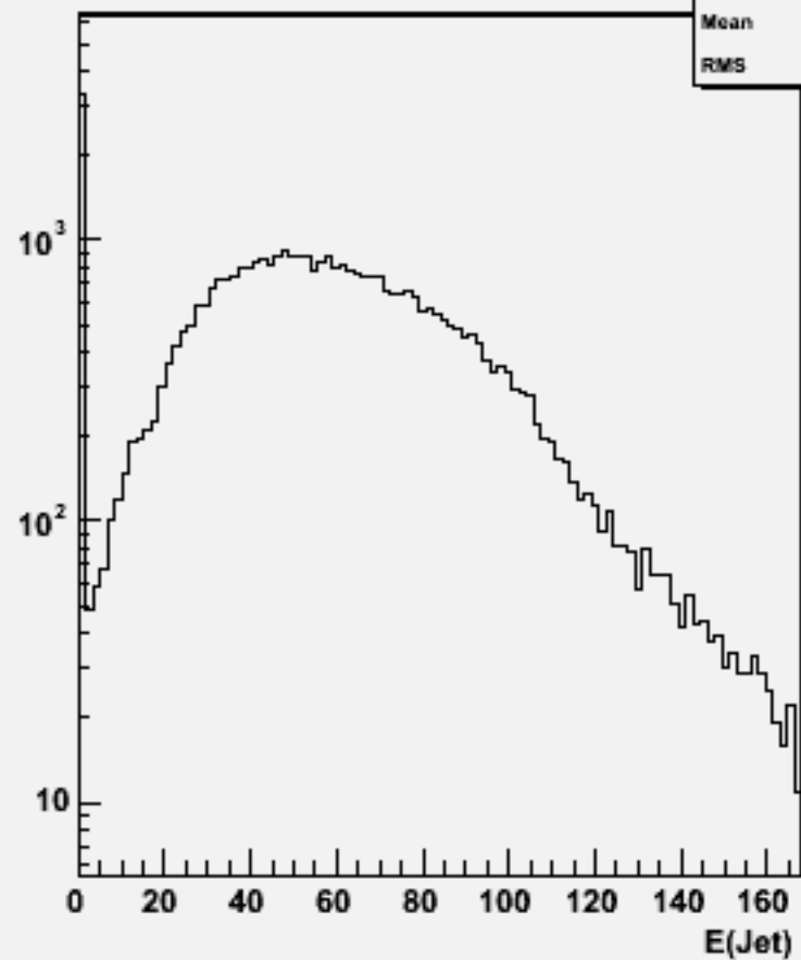
Jet energies(All jets)w102197 n1n1ddss_o
