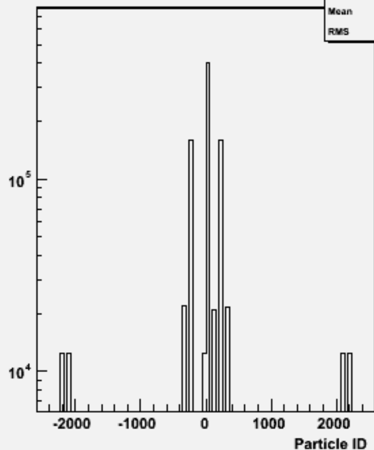
Particle ID : w102196 n1n1ddss_o
