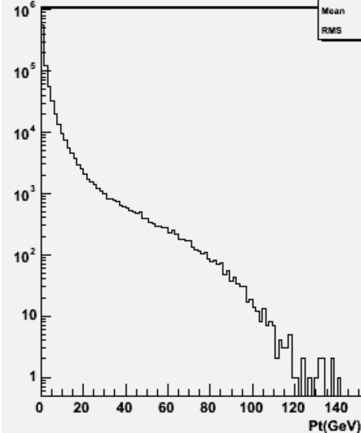
Particle Pt : w102196 n1n1ddss_o
