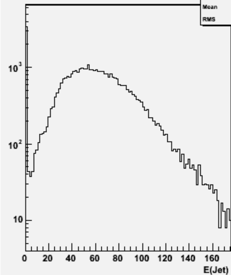
Jet energies(All jets)w102196 n1n1ddss_o
