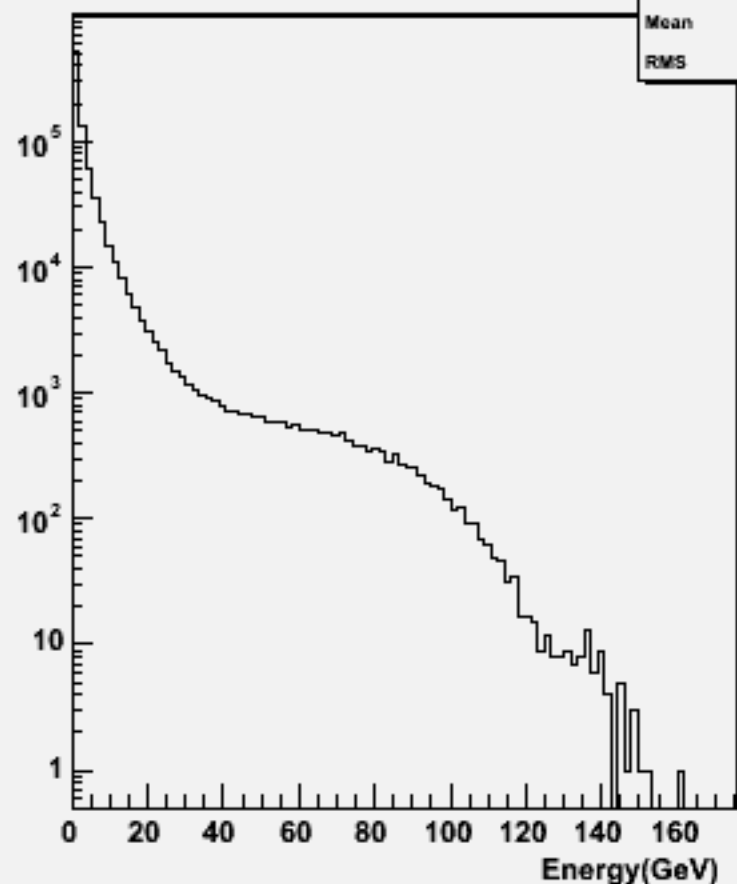
Particle Energy : w102196 n1n1ddss_o
