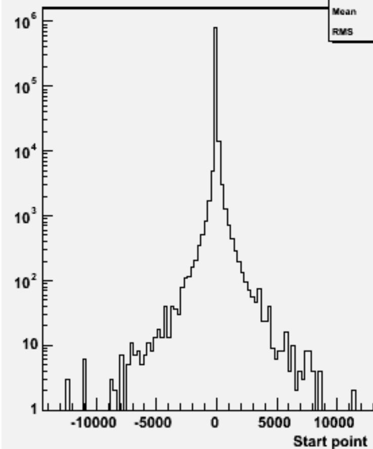
Start point Z : w102196 n1n1ddss_o
