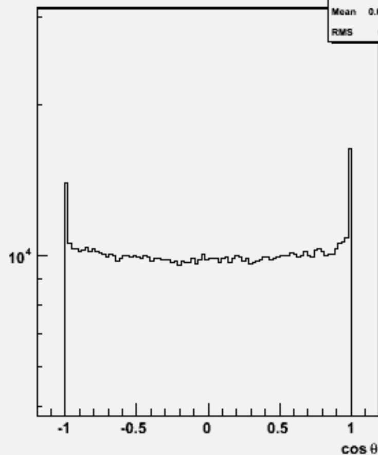
Particle cos \theta : w102196 n1n1ddss_o
