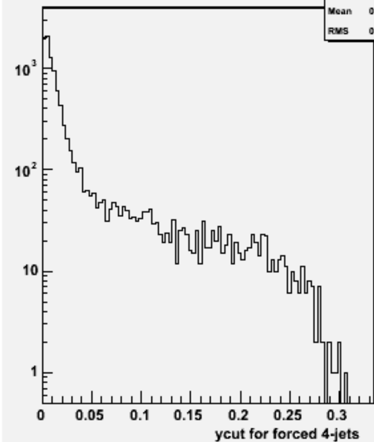
Ycut for 4-jets :w102196 n1n1ddss_o
