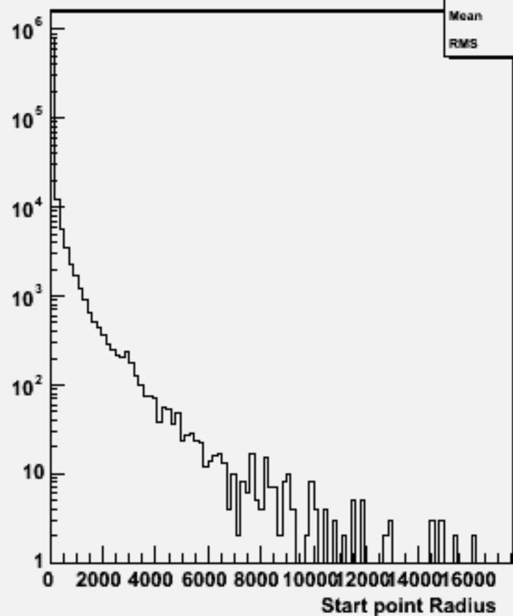
Start point R : w102196 n1n1ddss_o
