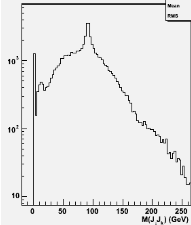
2jets mass(All comb)w102196 n1n1ddss_o
