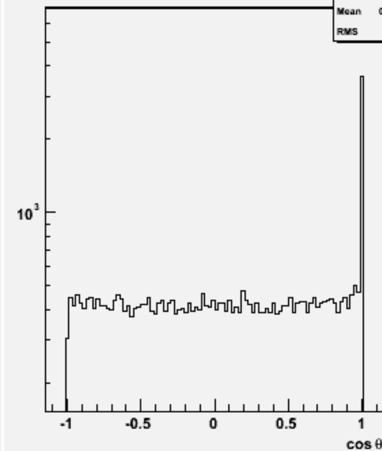
Jet cos \theta (All jets)w102196 n1n1ddss_o
