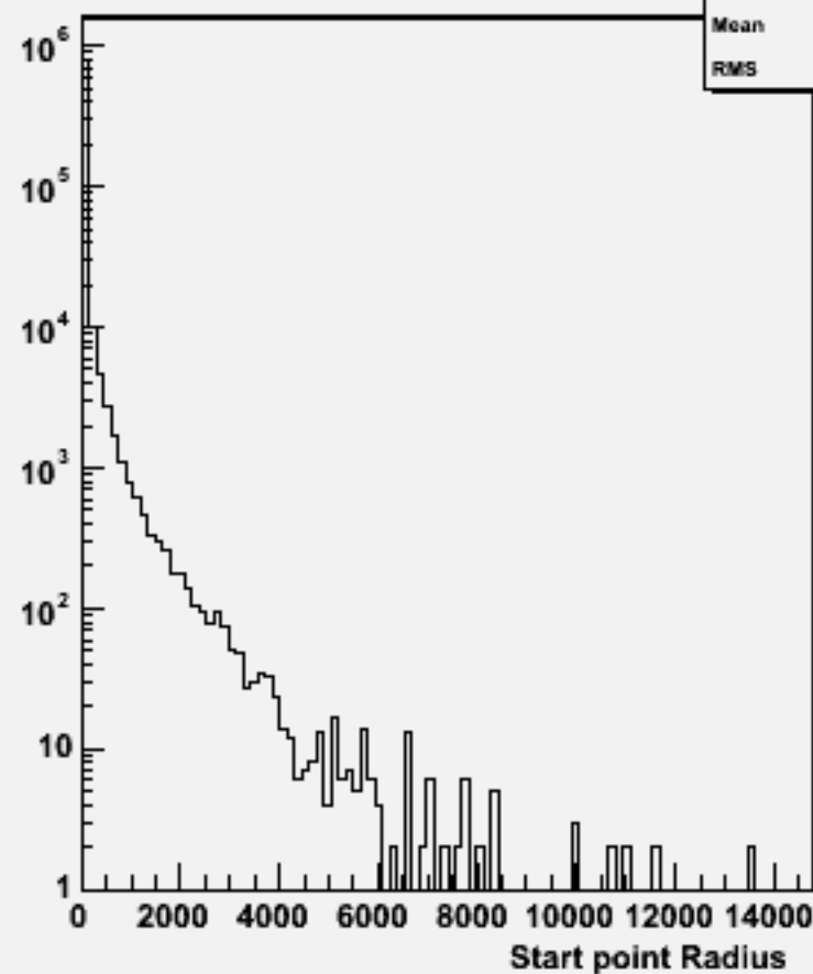
Start point R : w102193 n1n1dddd_o
