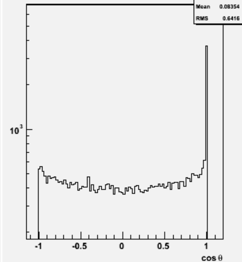
Jet cos \theta (All jets)w102193 n1n1dddd_o
