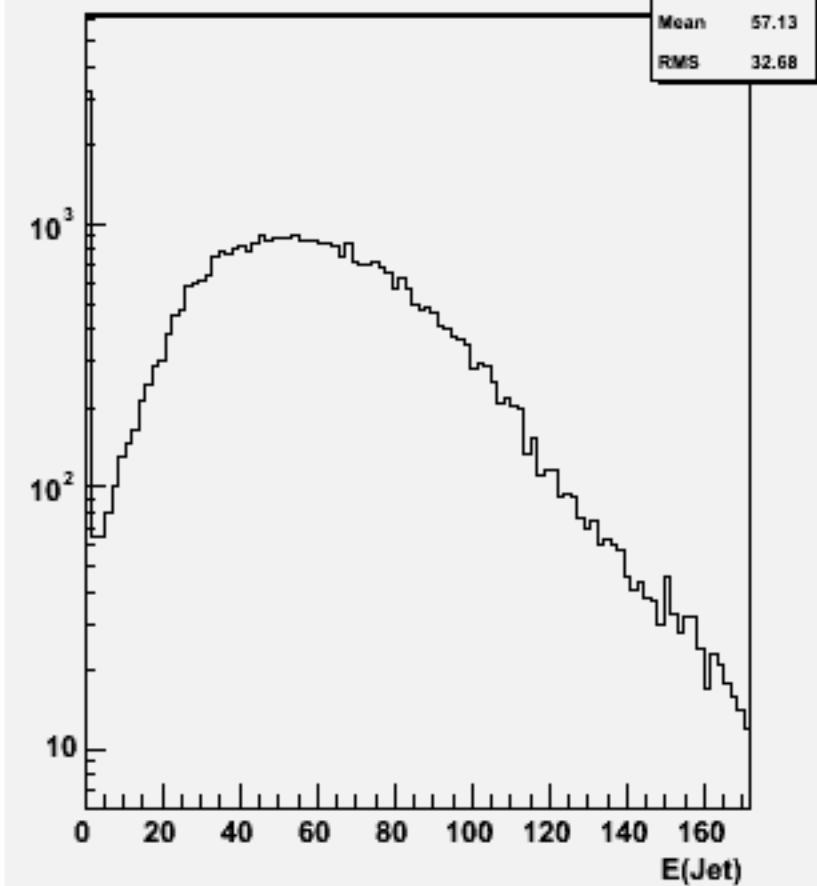
Jet energies(All jets)w102193 n1n1dddd_o
