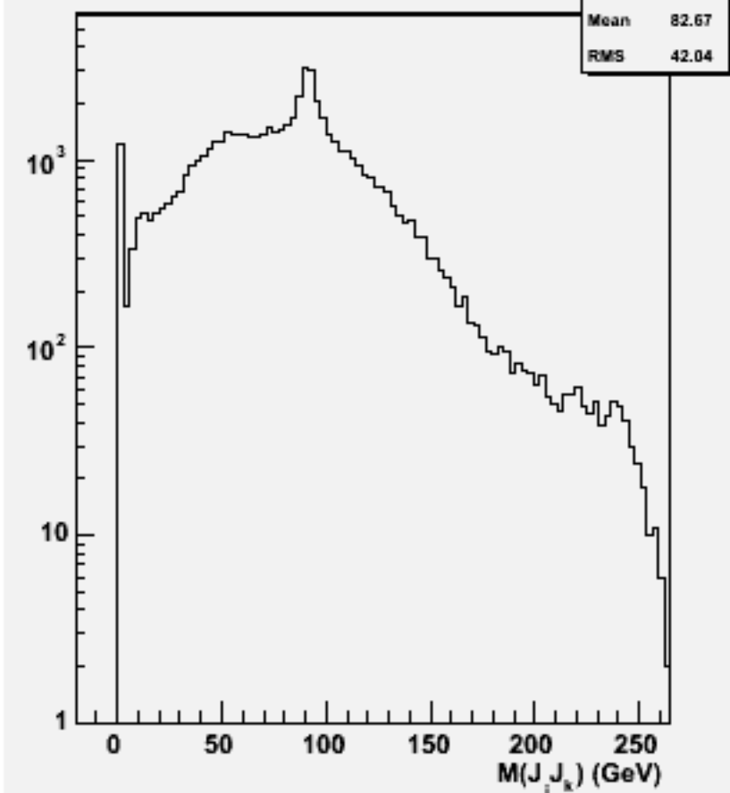
2jets mass(All comb)w102193 n1n1dddd_o
