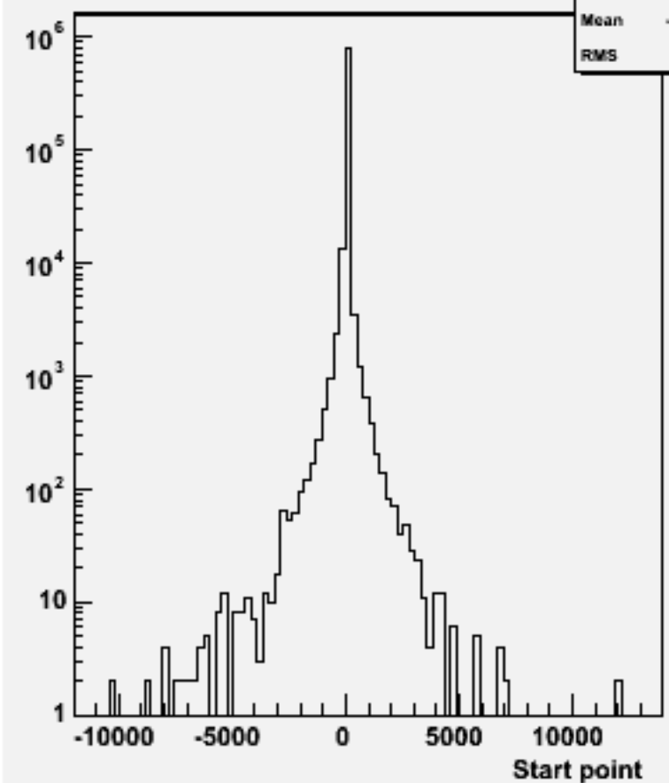
Start point Z : w102193 n1n1dddd_o
