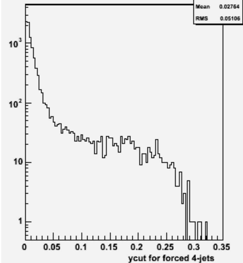
Ycut for 4-jets :w102193 n1n1dddd_o
