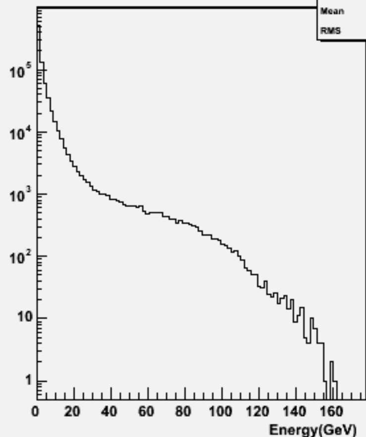
Particle Energy : w102193 n1n1dddd_o
