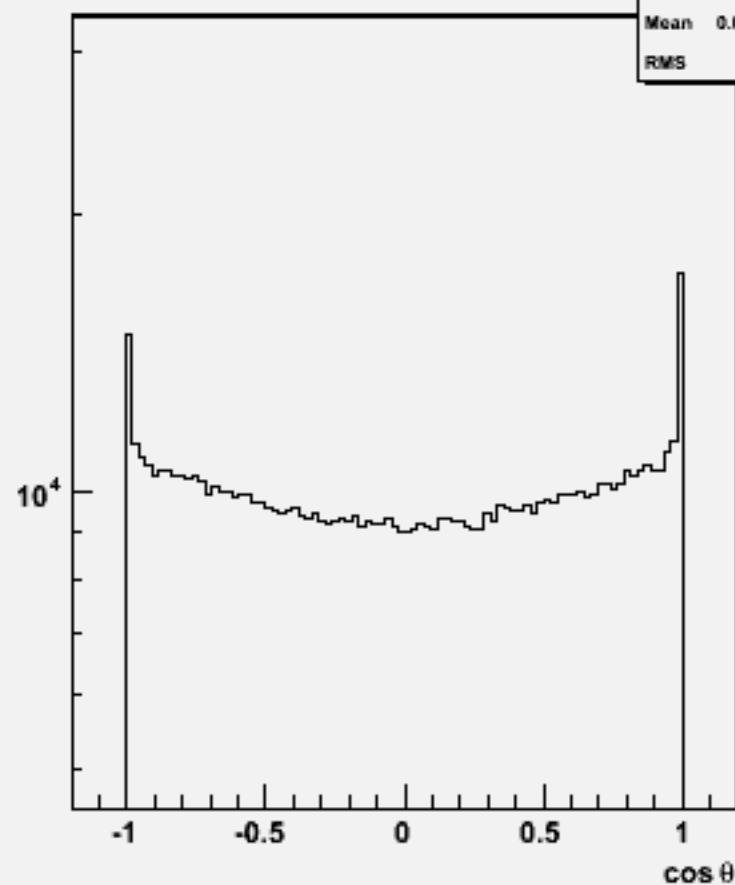
Particle cos \theta : w102193 n1n1dddd_o
