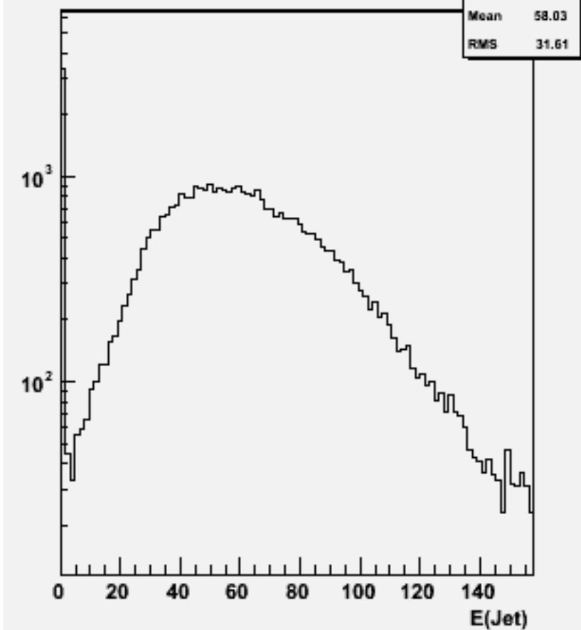
Jet energies(All jets)w102192 n1n1dddd_o
