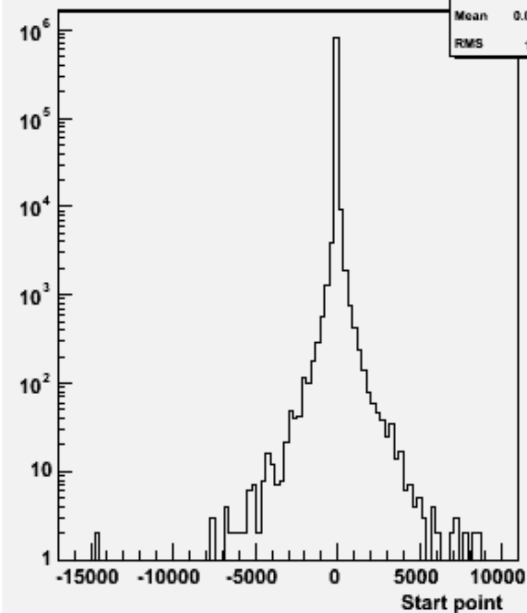
Start point Z : w102192 n1n1dddd_o
