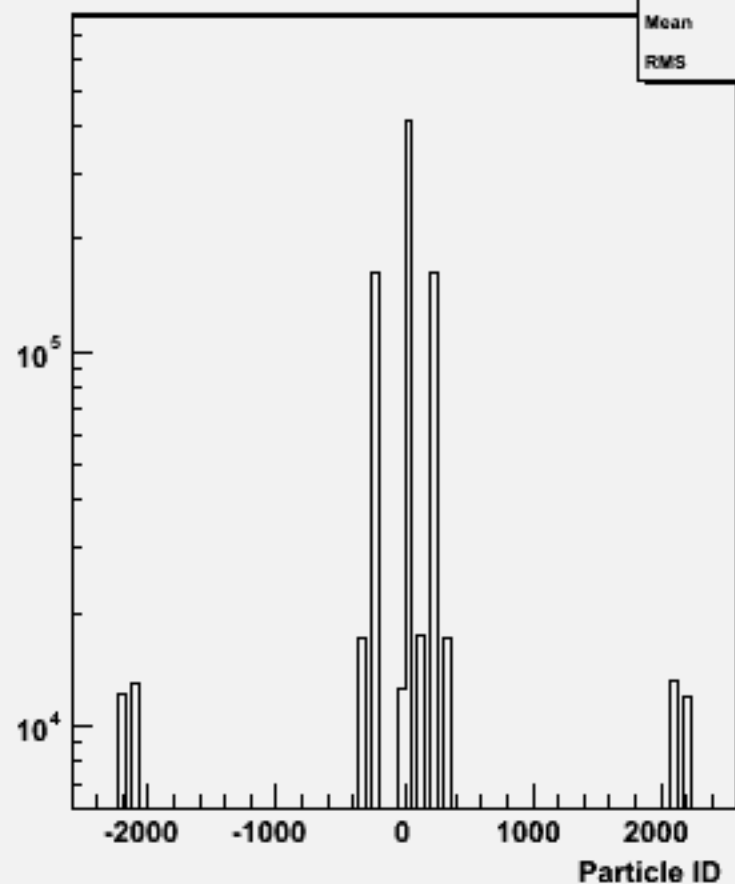
Particle ID : w102192 n1n1dddd_o
