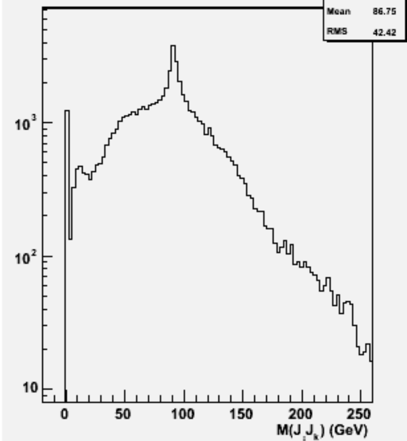
2jets mass(All comb)w102192 n1n1dddd_o
