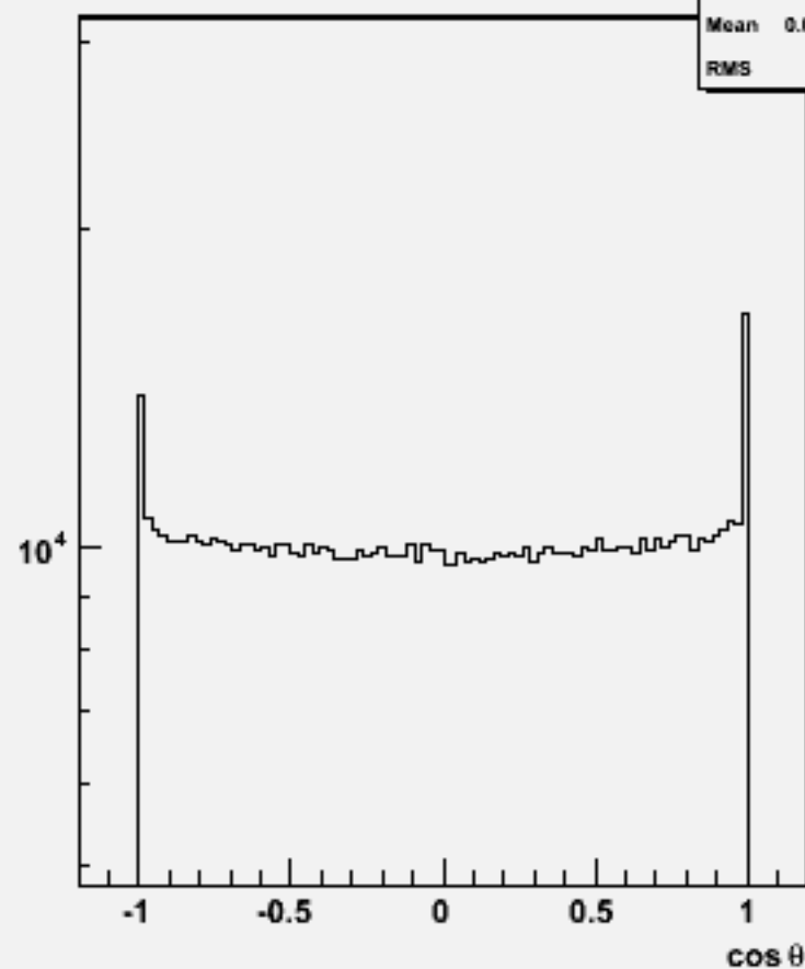
Particle cos \theta : w102192 n1n1dddd_o
