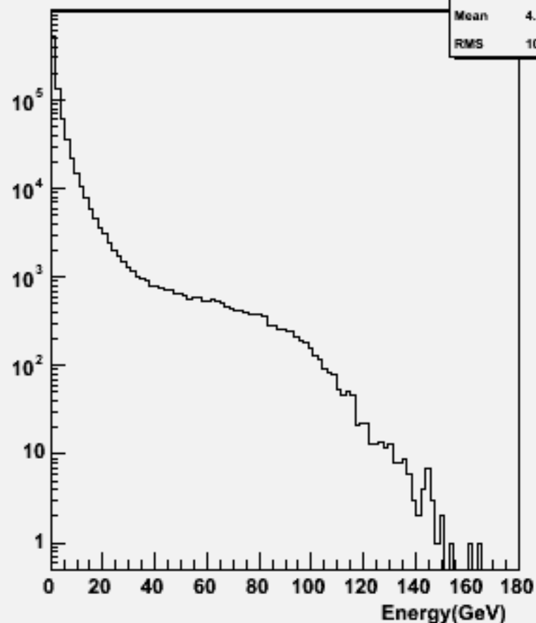
Particle Energy : w102192 n1n1dddd_o
