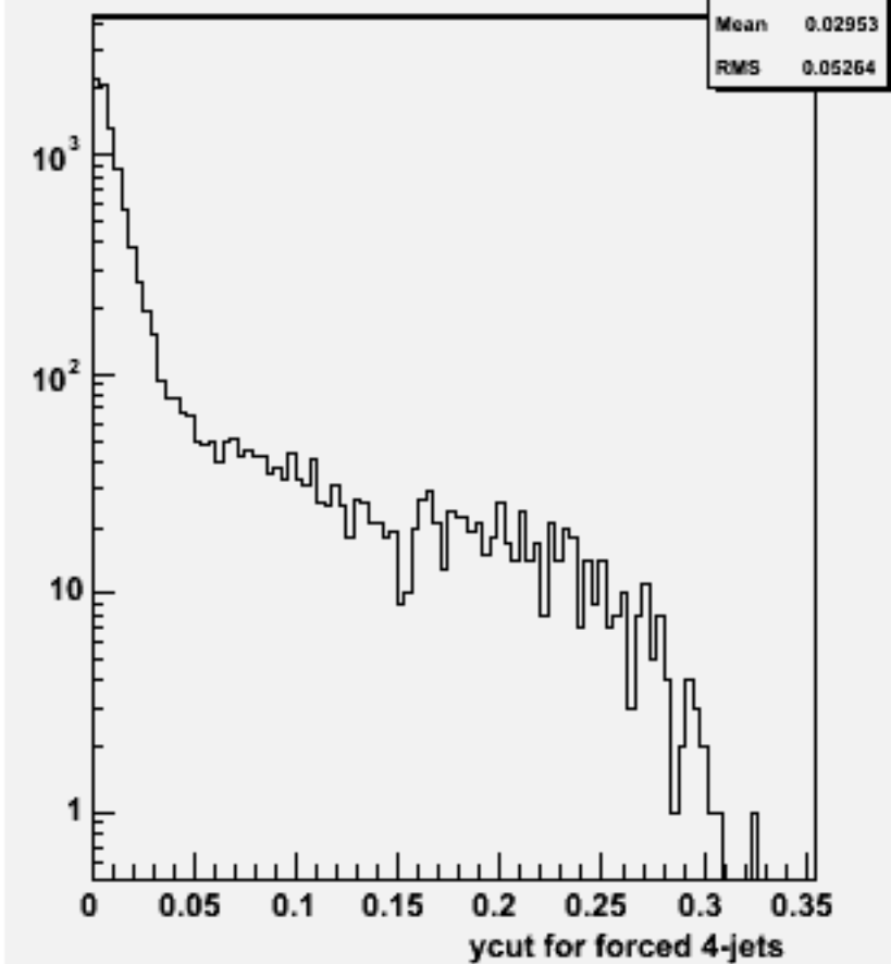
Ycut for 4-jets :w102192 n1n1dddd_o
