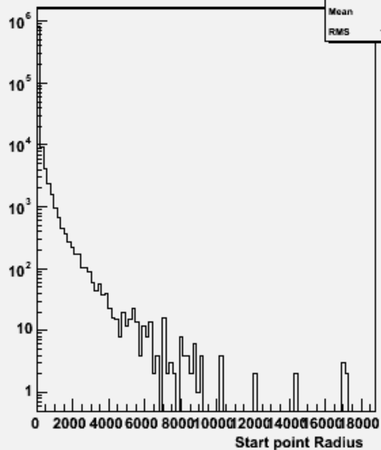
Start point R : w102192 n1n1dddd_o
