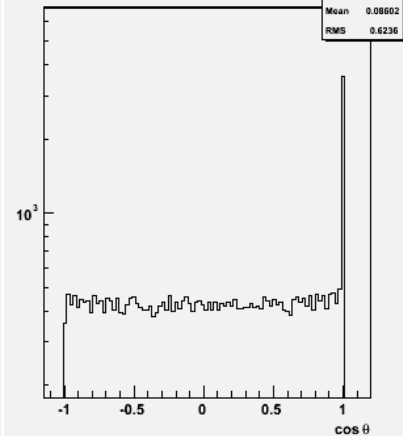
Jet cos \theta (All jets)w102192 n1n1dddd_o
