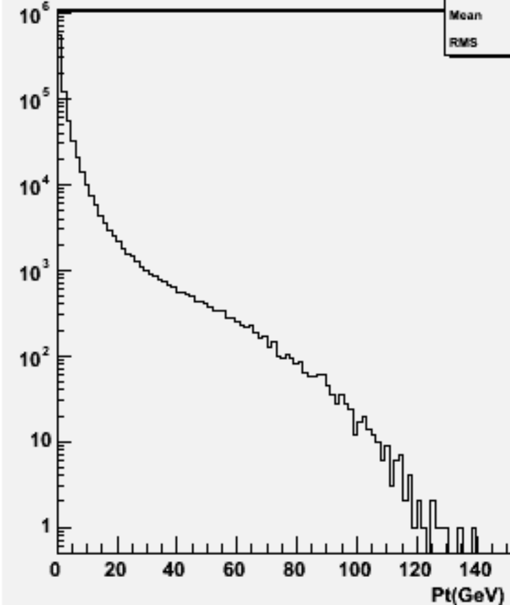
Particle Pt : w102192 n1n1dddd_o
