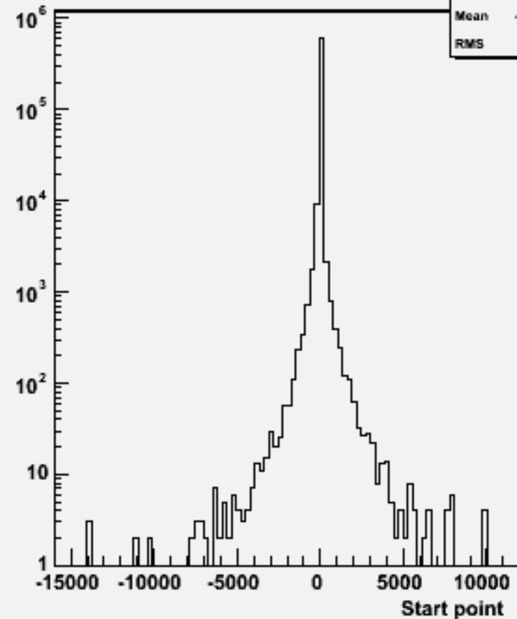
Start point Z : w102189 n1n1e3e3bb_o
