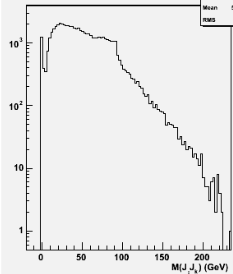
2jets mass(All comb)w102189 n1n1e3e3bb_o
