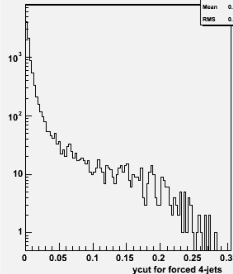
Ycut for 4-jets :w102189 n1n1e3e3bb_o
