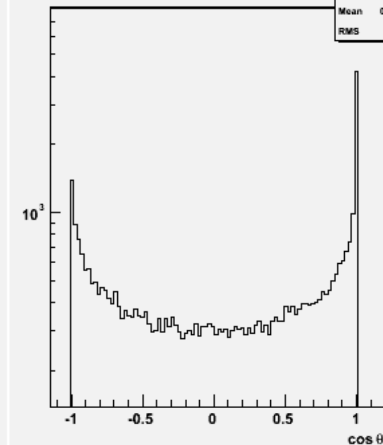
Jet cos \theta (All jets)w102189 n1n1e3e3bb_o
