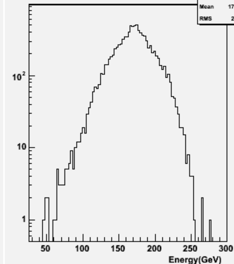
Thrust w102189 n1n1e3e3bb_o
