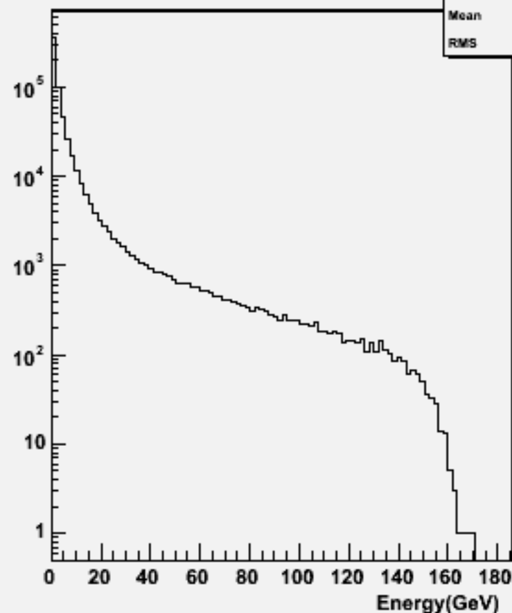
Particle Energy : w102189 n1n1e3e3bb_o
