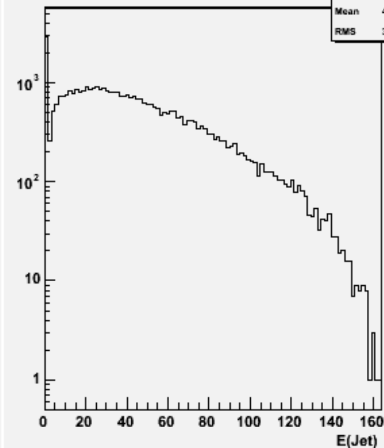
Jet energies(All jets)w102189 n1n1e3e3bb_o
