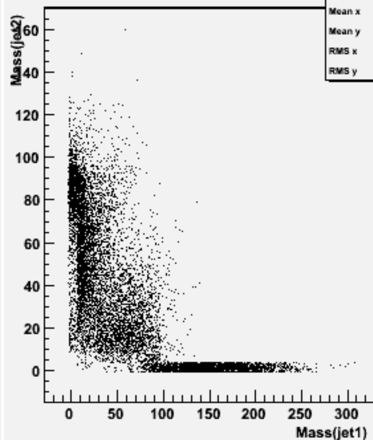
Jet mass for forced 2-jets : w102188 n1n1e3e3bb_o
