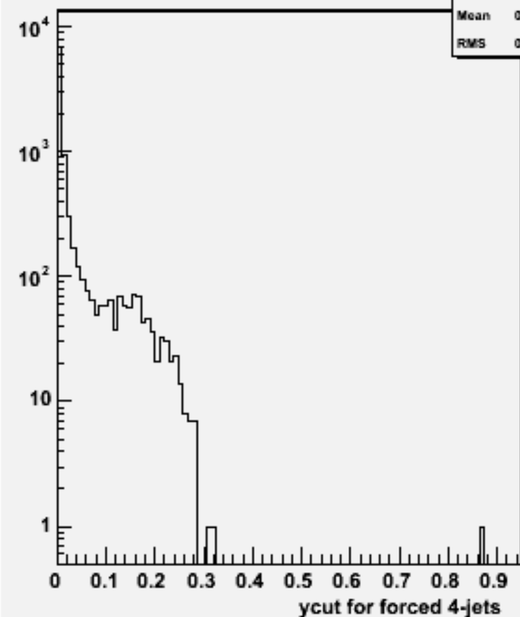
Ycut for 4-jets :w102188 n1n1e3e3bb_o
