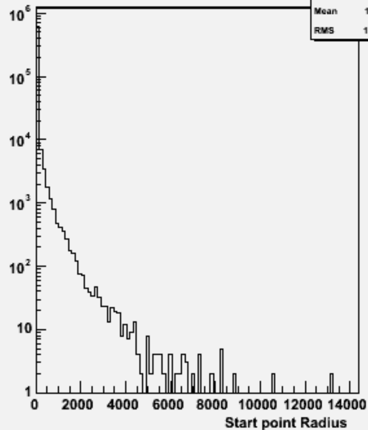
Start point R : w102188 n1n1e3e3bb_o
