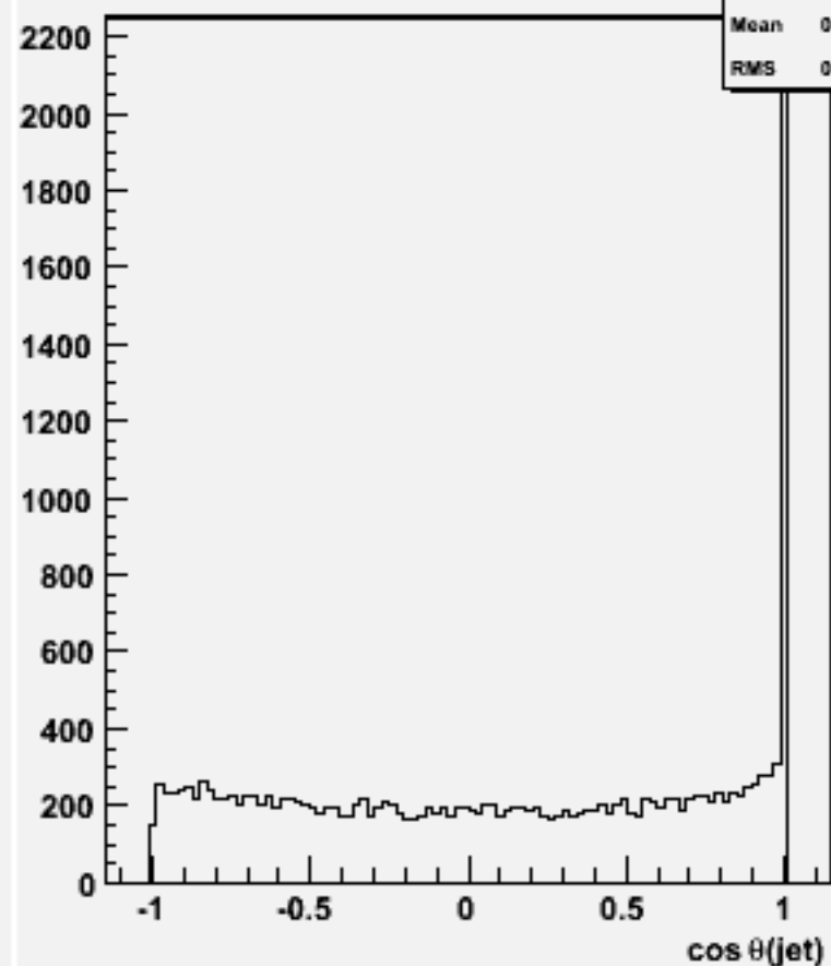
cos \theta for 2-jets :w102188 n1n1e3e3bb_o
