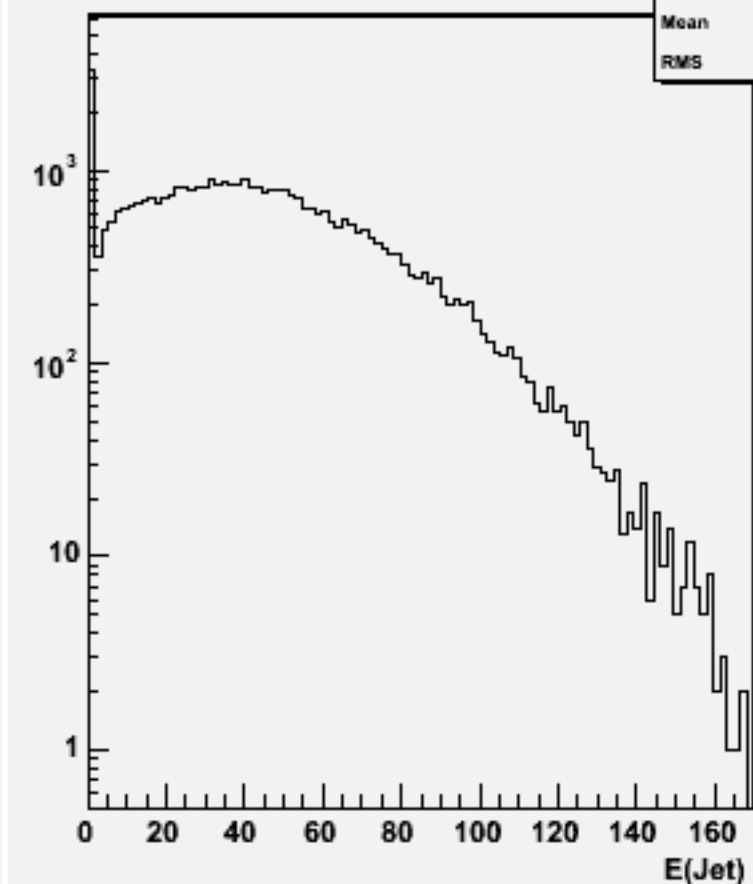
Jet energies(All jets)w102188 n1n1e3e3bb_o
