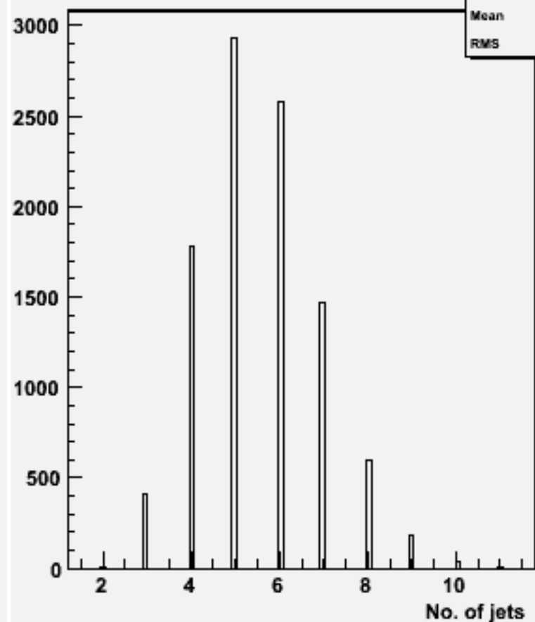
No. jets (ycut=0.001) : w102188 n1n1e3e3bb_o
