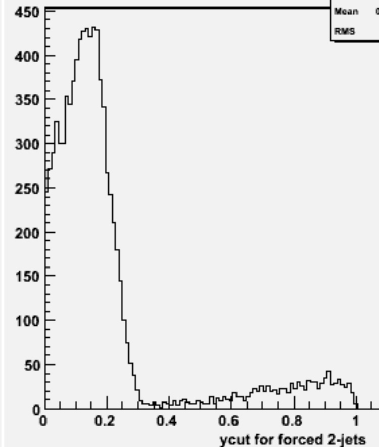
Ycut for 2-jets :w102188 n1n1e3e3bb_o
