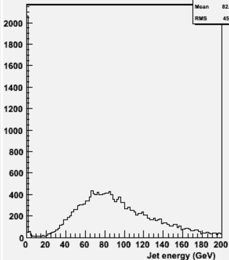
energy for 2-jets :w102188 n1n1e3e3bb_o
