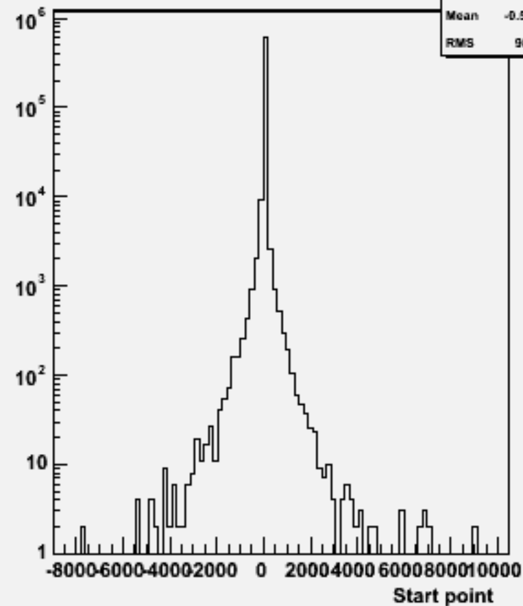
Start point Z : w102188 n1n1e3e3bb_o
