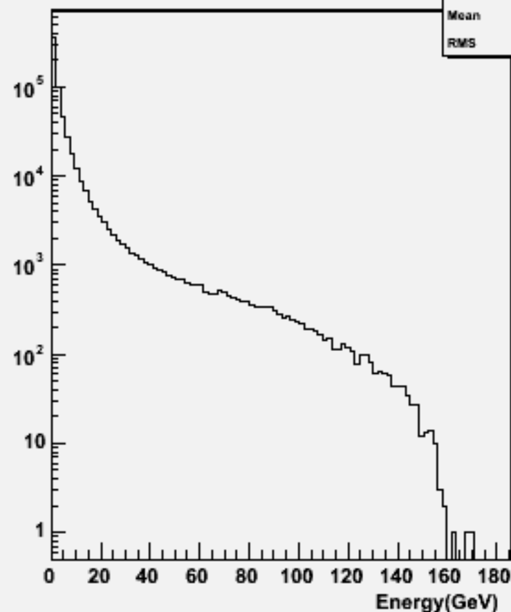
Particle Energy : w102188 n1n1e3e3bb_o
