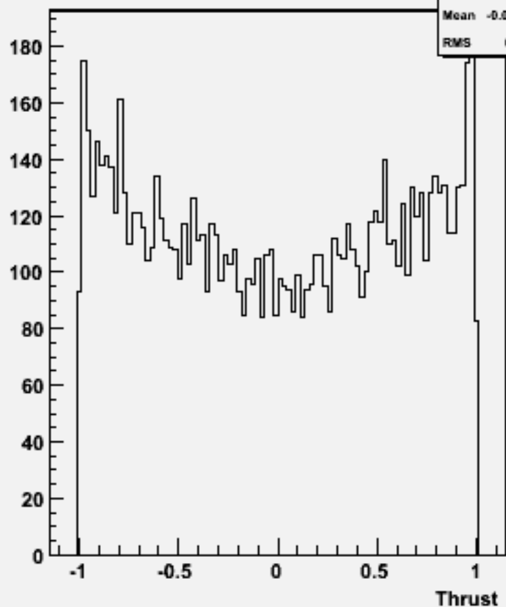
cos \Theta (thrust) w102188 n1n1e3e3bb_o
