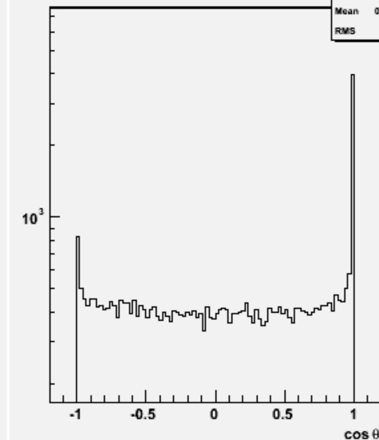
Jet cos \theta (All jets)w102188 n1n1e3e3bb_o
