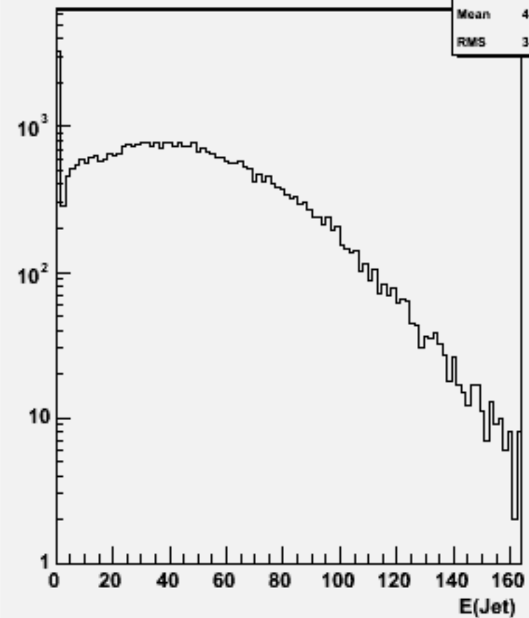
Jet energies(All jets)w102184 n1n1e3e3ss_o
