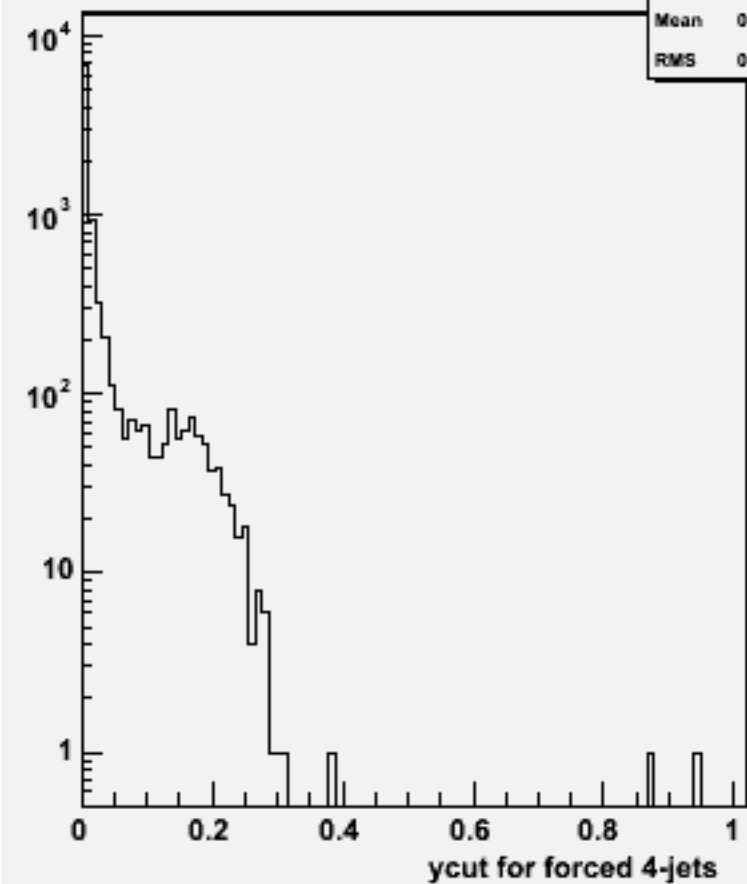
Ycut for 4-jets :w102184 n1n1e3e3ss_o
