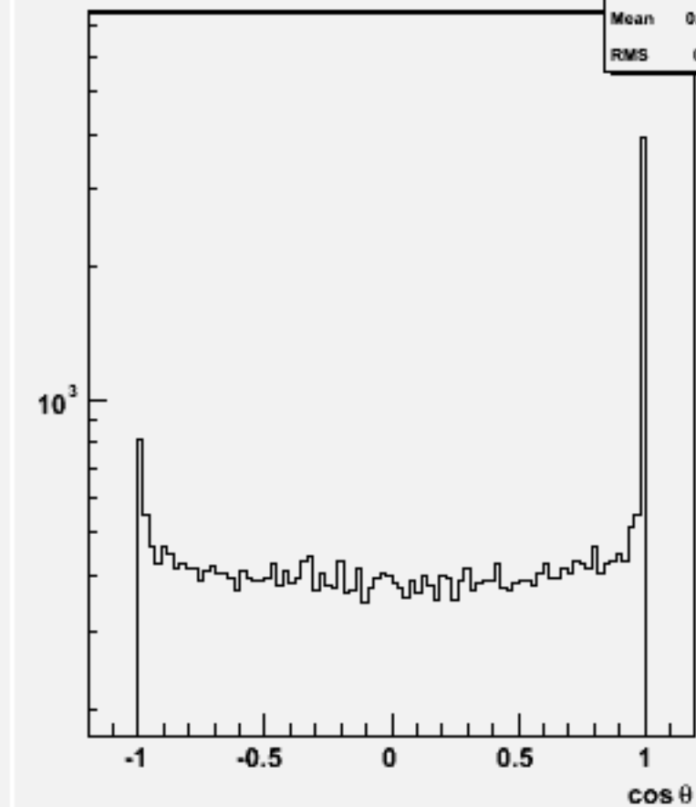
Jet cos \theta (All jets)w102184 n1n1e3e3ss_o
