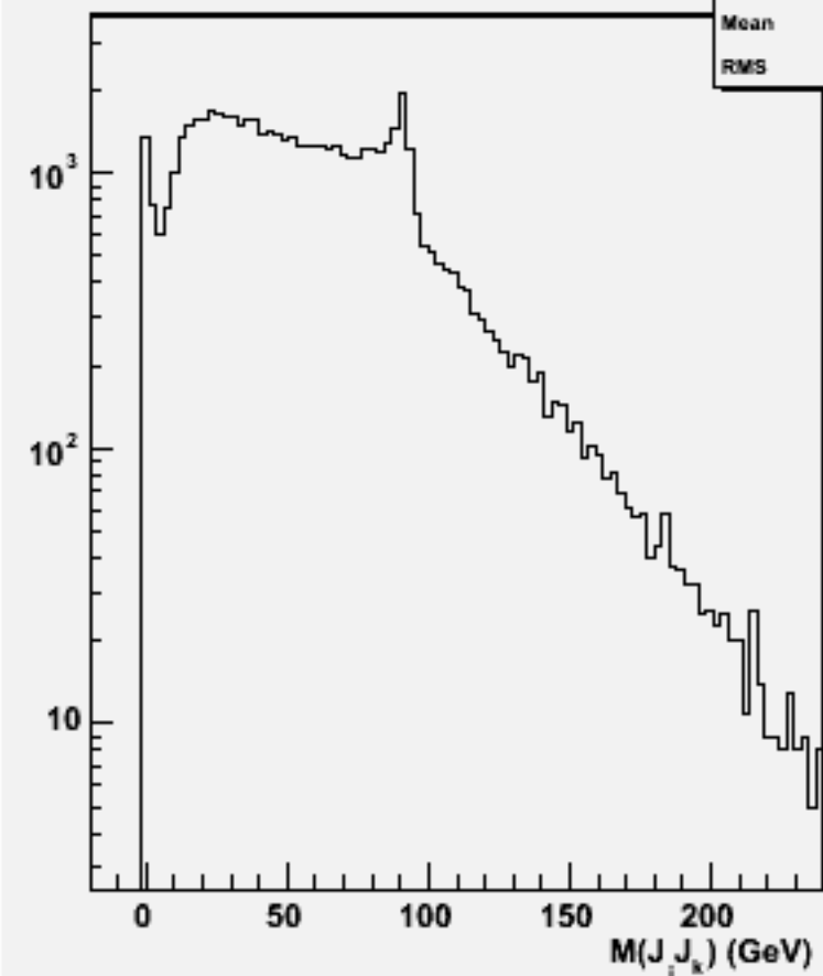
2jets mass(All comb)w102184 n1n1e3e3ss_o
