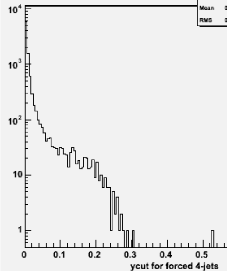
Ycut for 4-jets :w102181 n1n1e3e3dd_o
