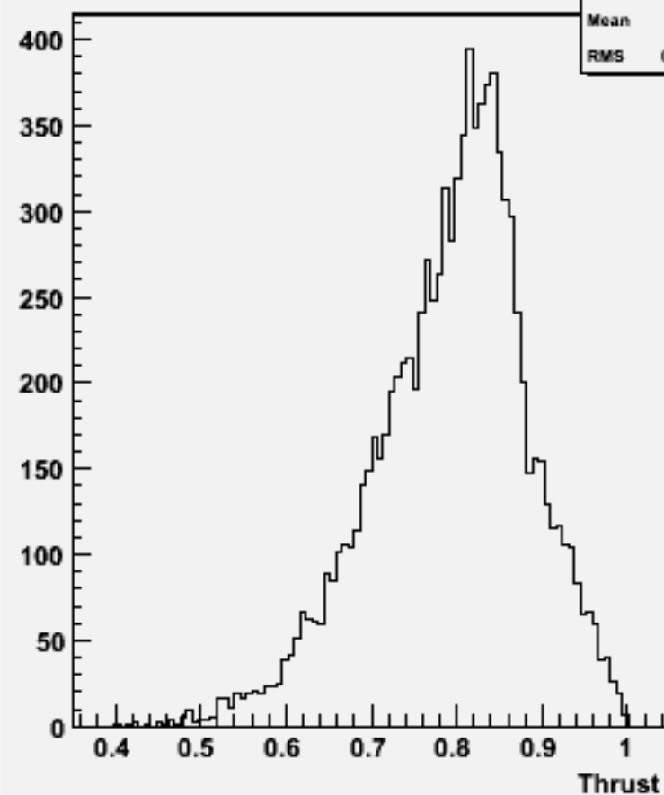
Thrust w102181 n1n1e3e3dd_o
