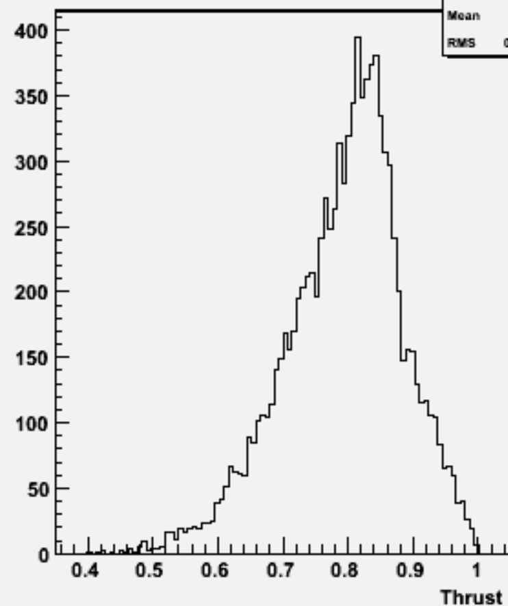
Thrust w102181 n1n1e3e3dd_o
