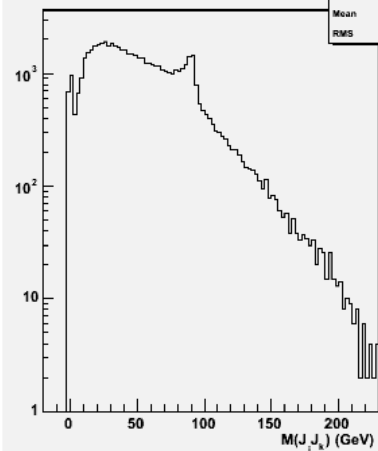
2jets mass(All comb)w102181 n1n1e3e3dd_o
