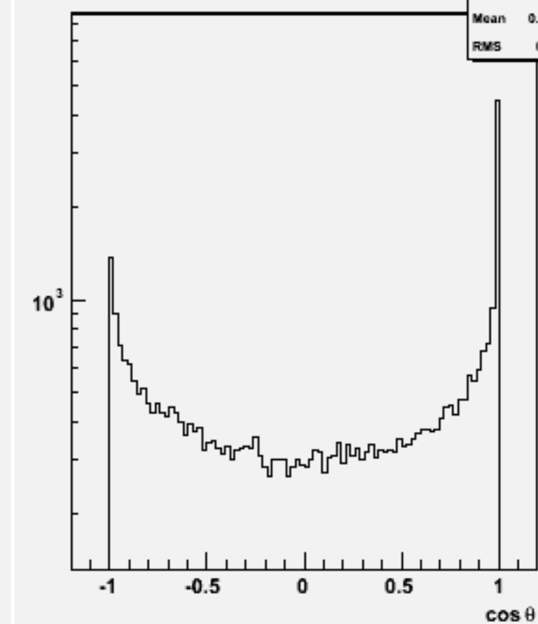
Jet cos \theta (All jets)w102181 n1n1e3e3dd_o
