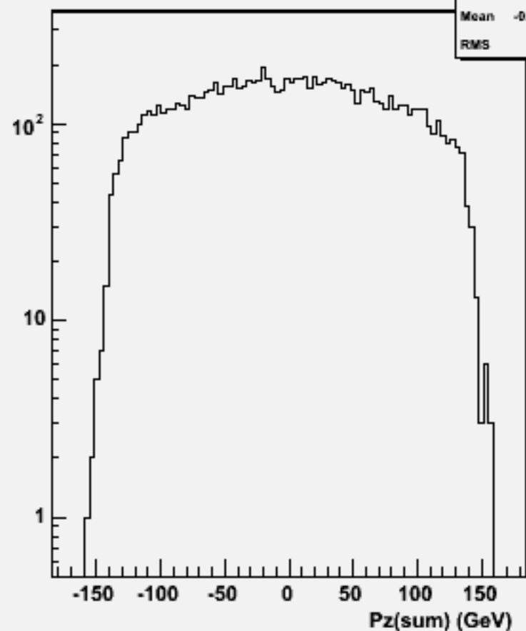
Pz Sum: w102181 n1n1e3e3dd_o
