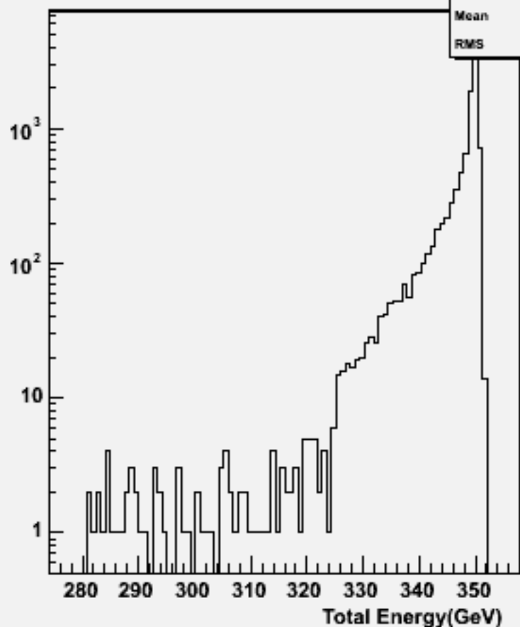
Pt Sum: w102181 n1n1e3e3dd_o
