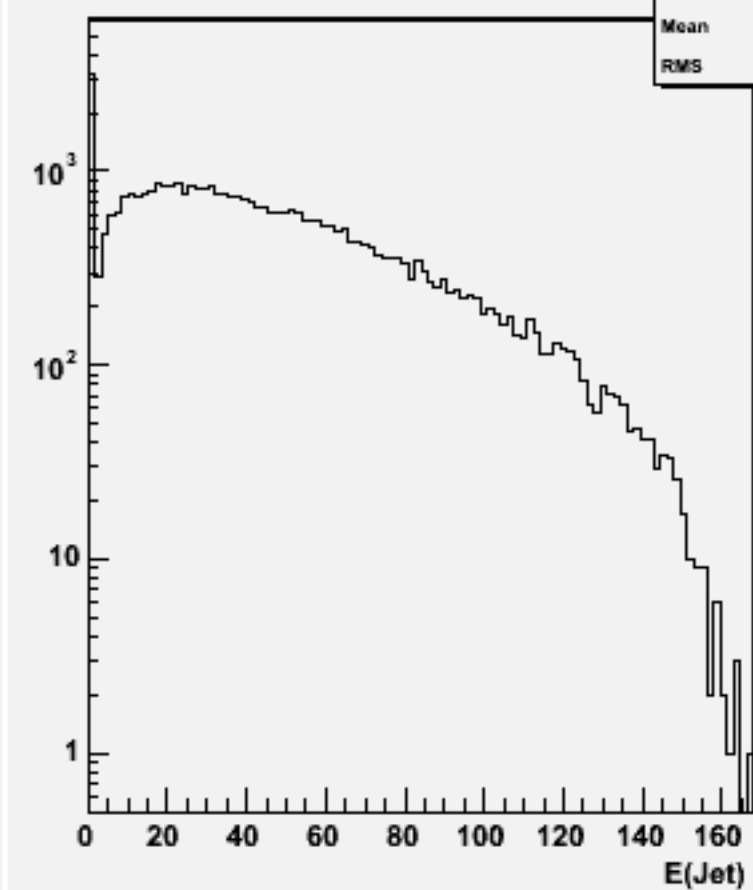
Jet energies(All jets)w102181 n1n1e3e3dd_o
