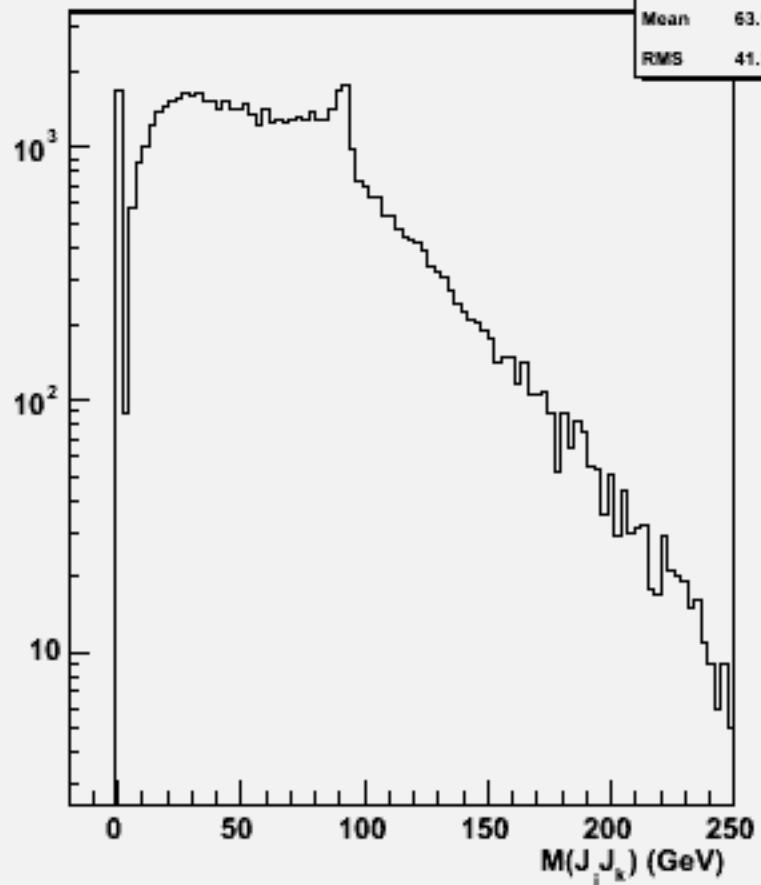
2jets mass(All comb)w102173 n1n1e2e2bb_o
