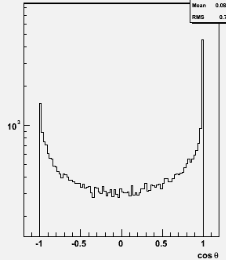
Jet cos \theta (All jets)w102173 n1n1e2e2bb_o
