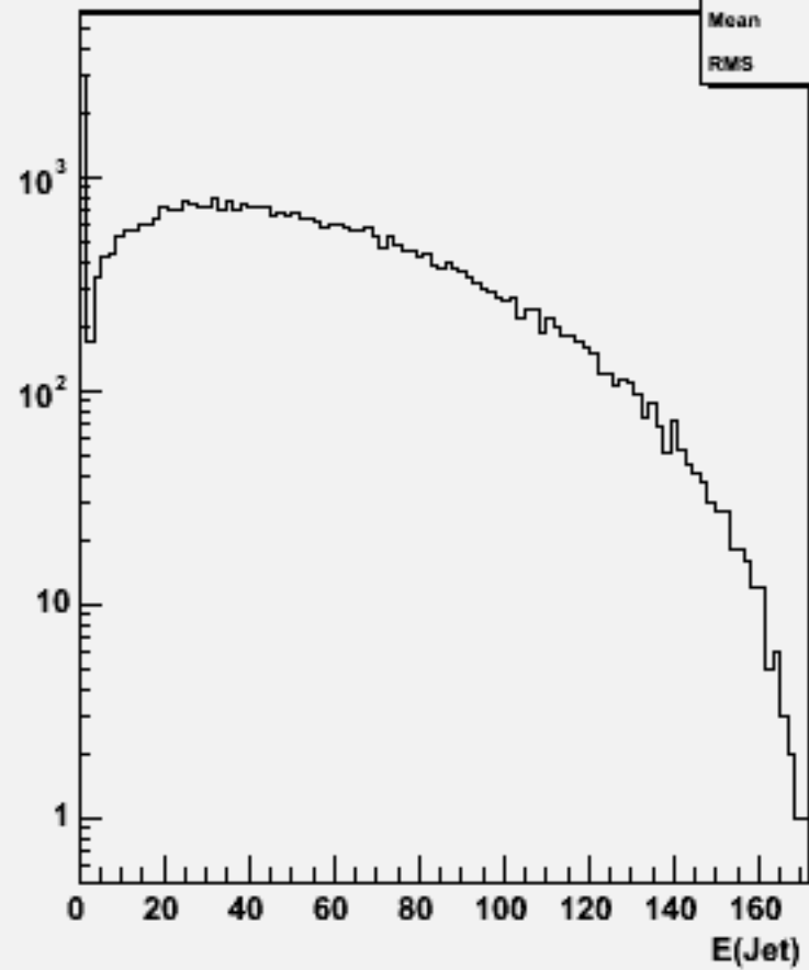
Jet energies(All jets)w102173 n1n1e2e2bb_o
