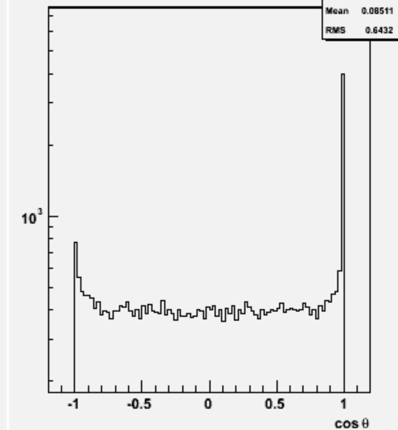
Jet cos \theta (All jets)w102172 n1n1e2e2bb_o
