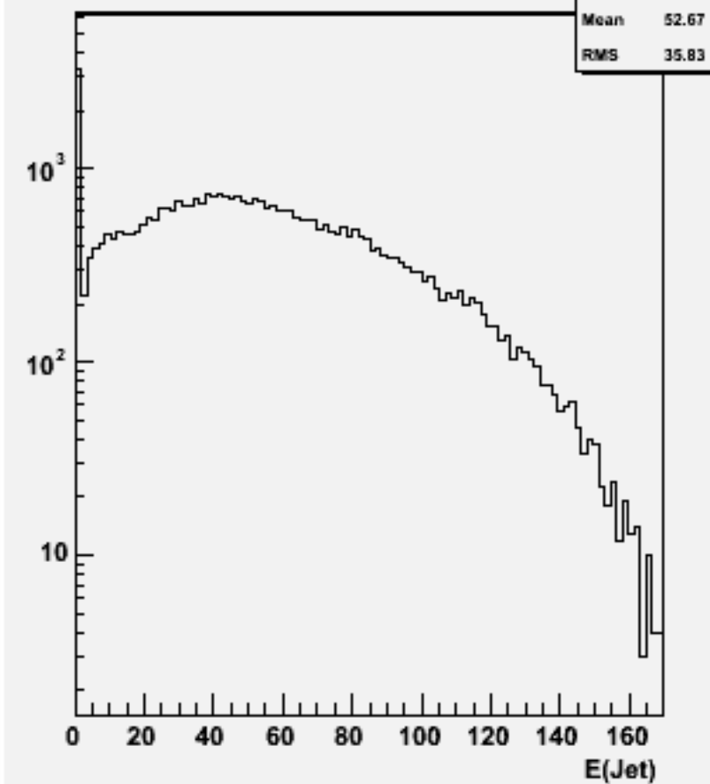
Jet energies(All jets)w102172 n1n1e2e2bb_o
