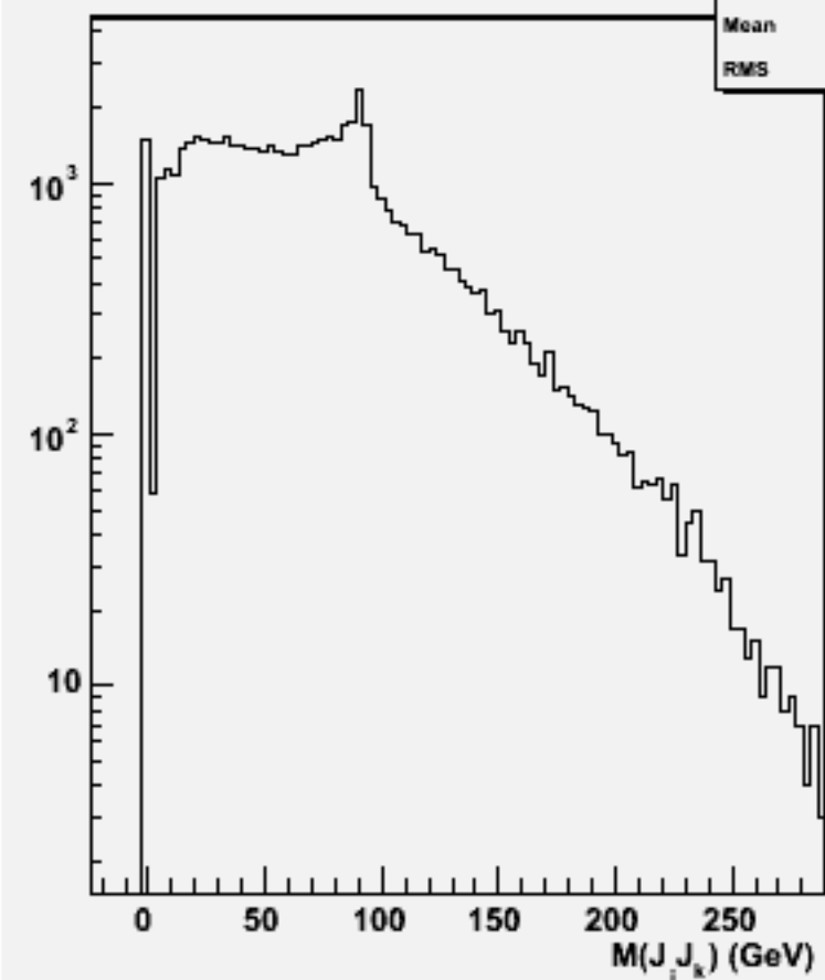
2jets mass(All comb)w102172 n1n1e2e2bb_o
