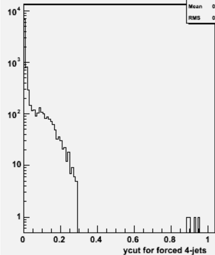
Ycut for 4-jets :w102172 n1n1e2e2bb_o
