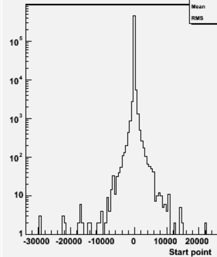
Start point Z : w102169 n1n1e2e2ss_o
