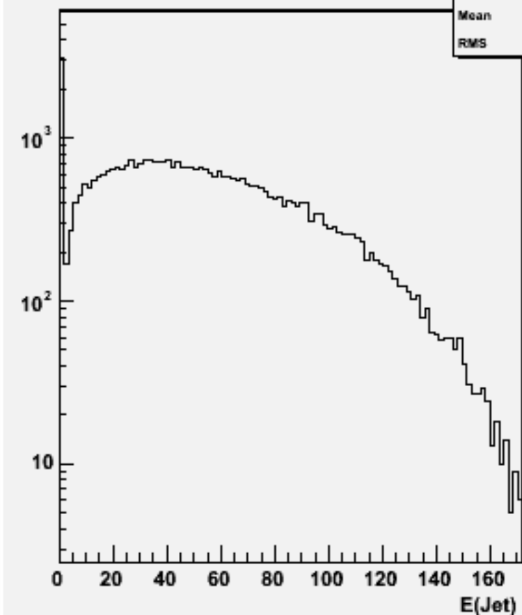
Jet energies(All jets)w102169 n1n1e2e2ss_o
