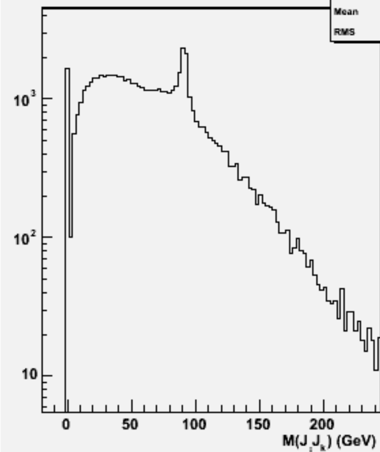
2jets mass(All comb)w102169 n1n1e2e2ss_o
