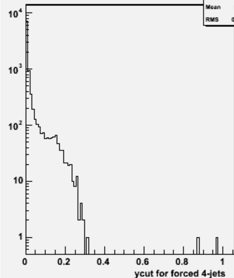
Ycut for 4-jets :w102169 n1n1e2e2ss_o
