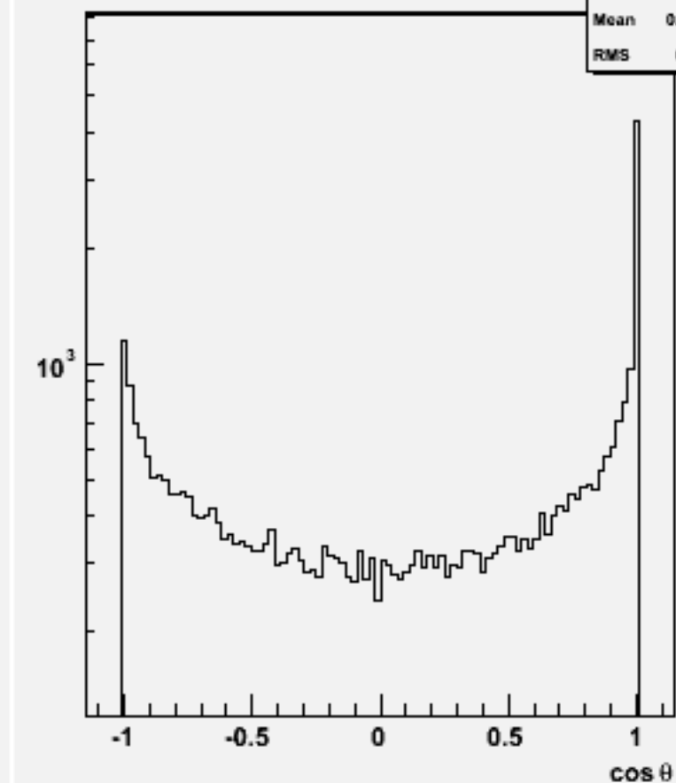
Jet cos \theta (All jets)w102169 n1n1e2e2ss_o
