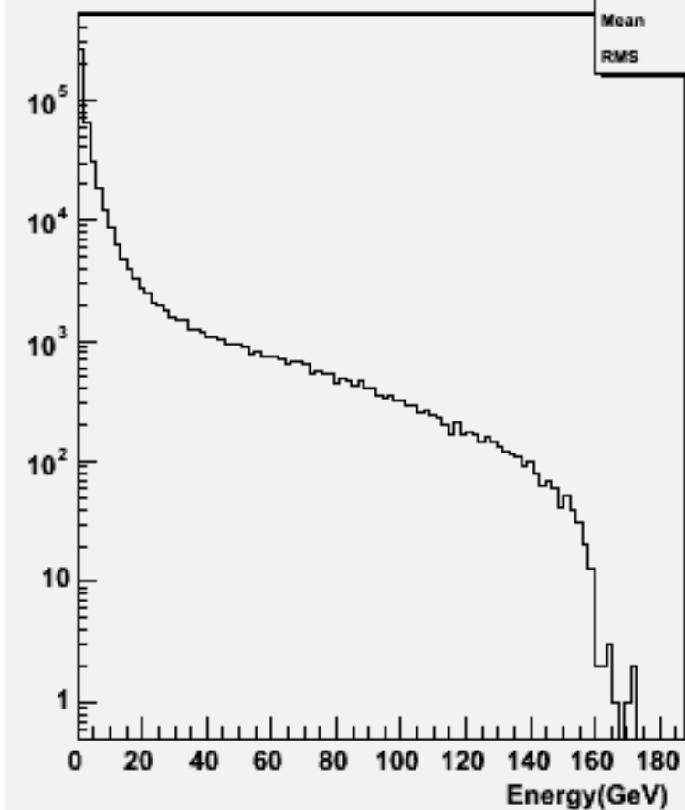
Particle Energy : w102169 n1n1e2e2ss_o
