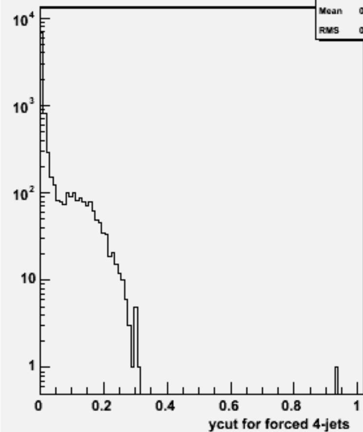
Ycut for 4-jets :w102168 n1n1e2e2ss_o
