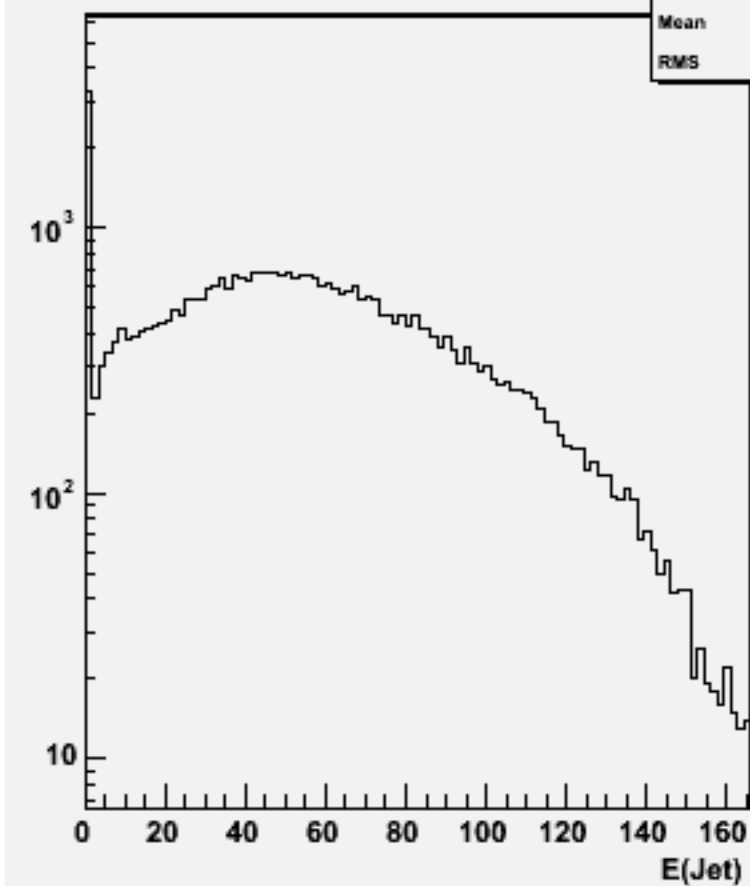
Jet energies(All jets)w102168 n1n1e2e2ss_o
