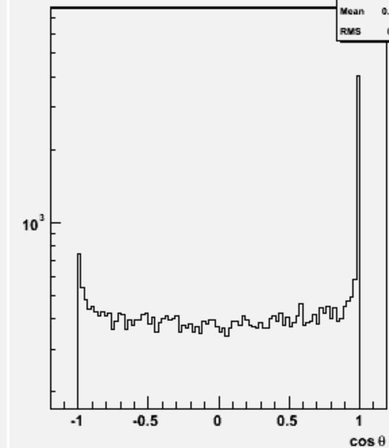
Jet cos \theta (All jets)w102168 n1n1e2e2ss_o
