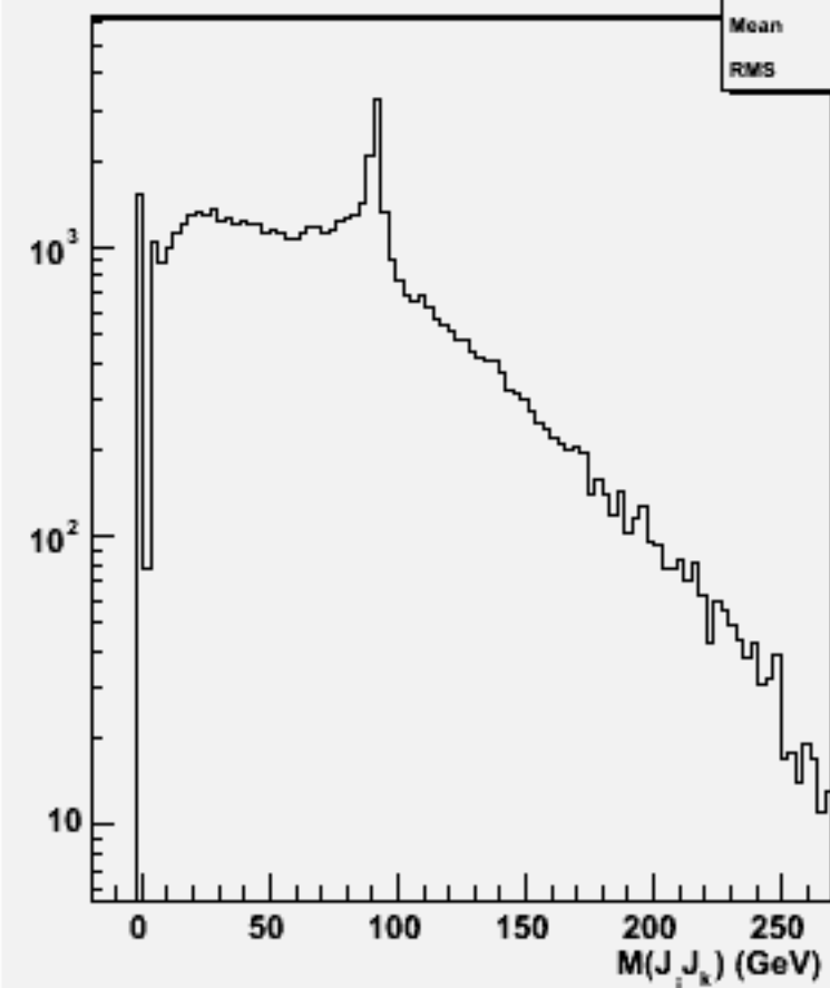
2jets mass(All comb)w102168 n1n1e2e2ss_o
