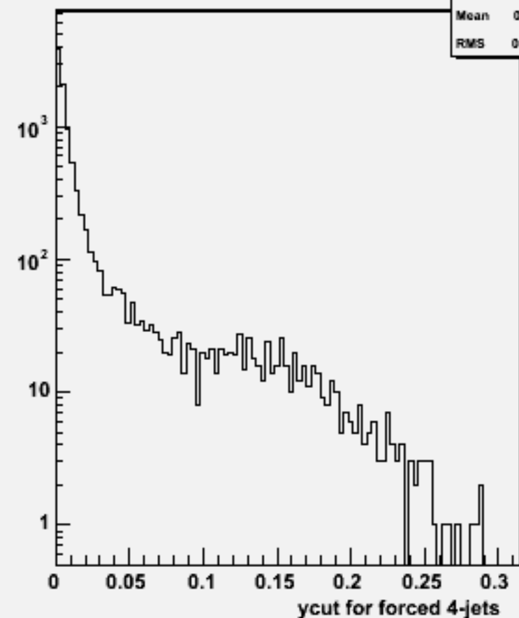
Ycut for 4-jets :w102165 n1n1e2e2dd_o
