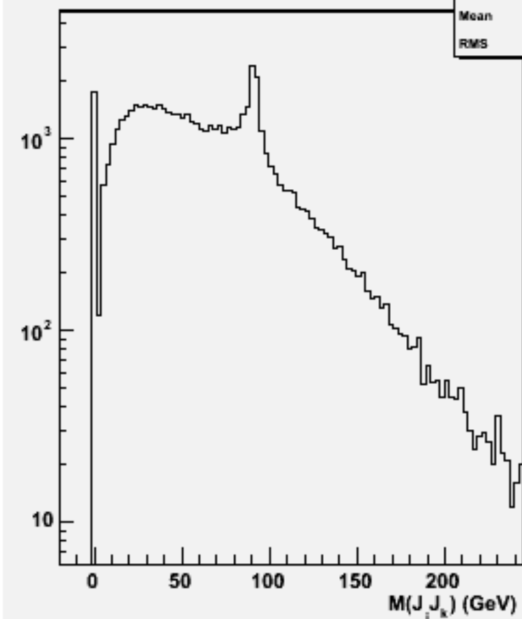
2jets mass(All comb)w102165 n1n1e2e2dd_o
