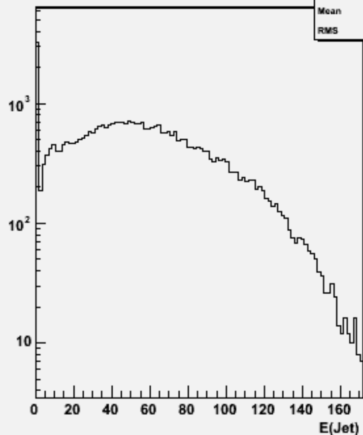
Jet energies(All jets)w102164 n1n1e2e2dd_o
