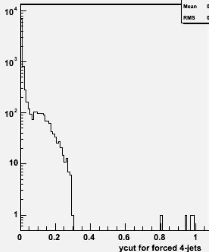
Ycut for 4-jets :w102164 n1n1e2e2dd_o
