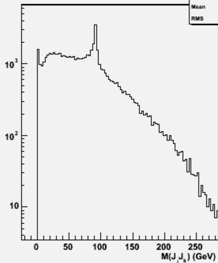
2jets mass(All comb)w102164 n1n1e2e2dd_o
