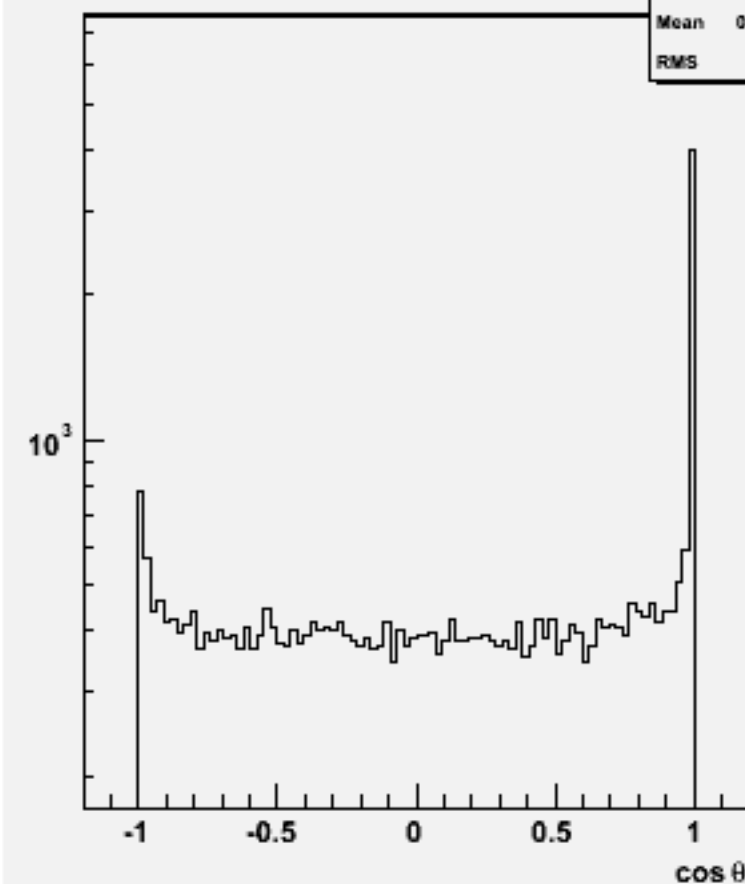
Jet cos \theta (All jets)w102164 n1n1e2e2dd_o
