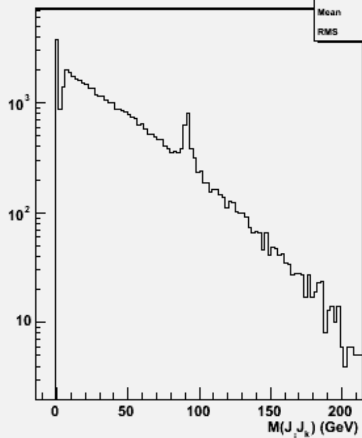
2jets mass(All comb)w102161 n1n1e2e2e3e3_o
