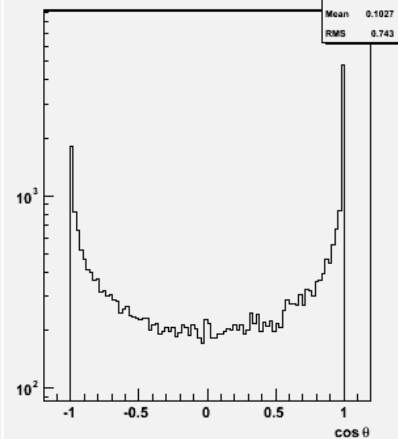
Jet cos theta (All jets)w102161 n1n1e2e2e3e3_o
