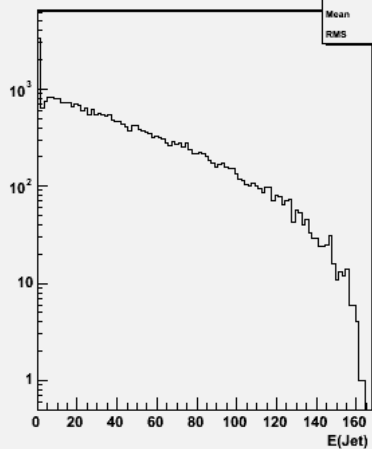
Jet energies(All jets)w102161 n1n1e2e2e3e3_o
