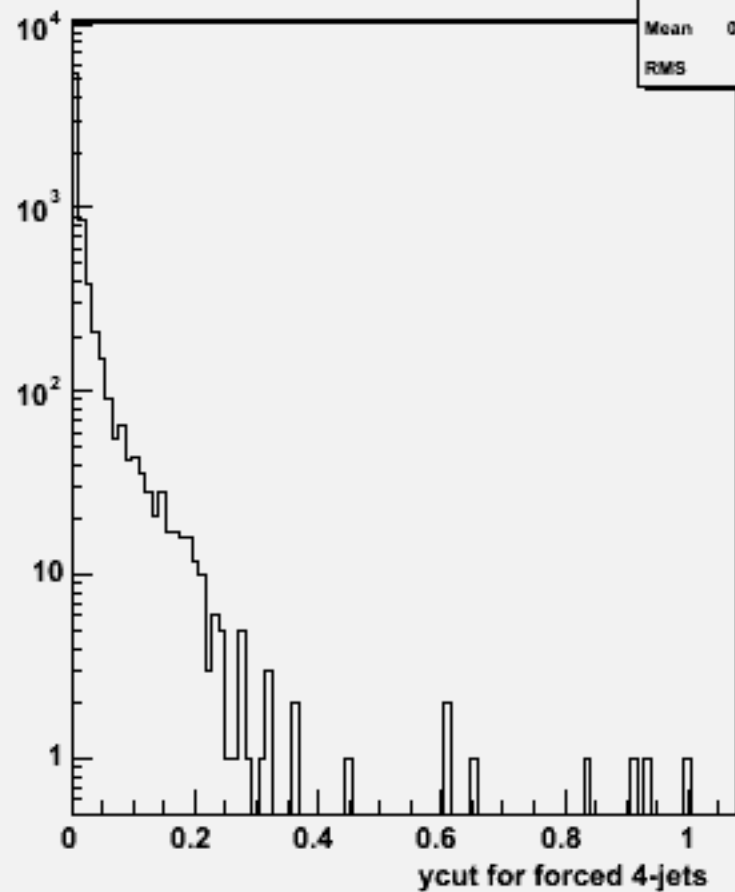
Ycut for 4-jets :w102161 n1n1e2e2e3e3_o
