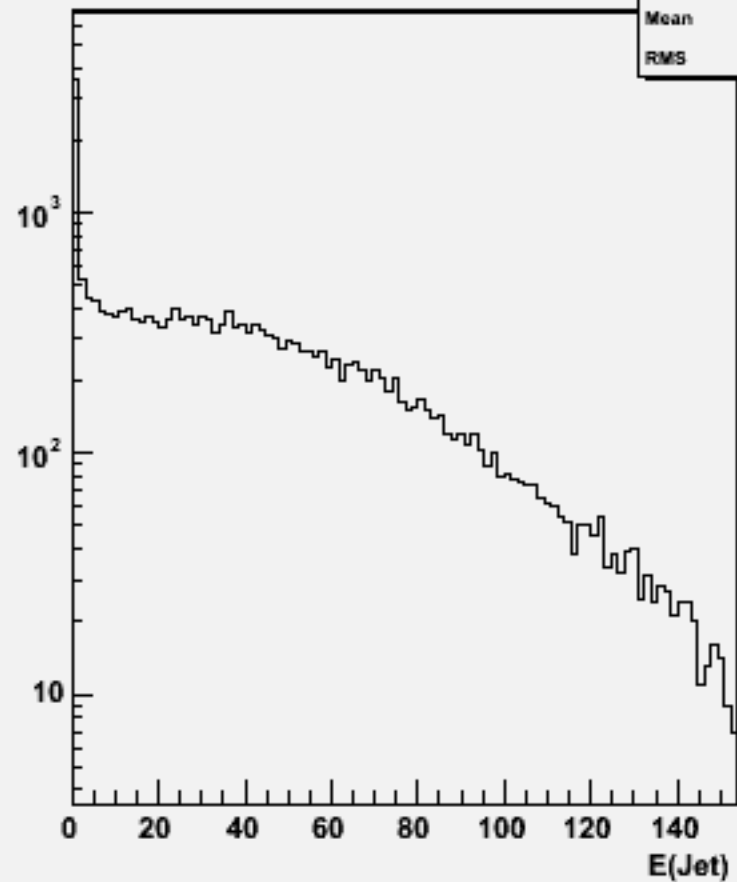
Jet energies(All jets)w102160 n1n1e2e2e3e3_o
