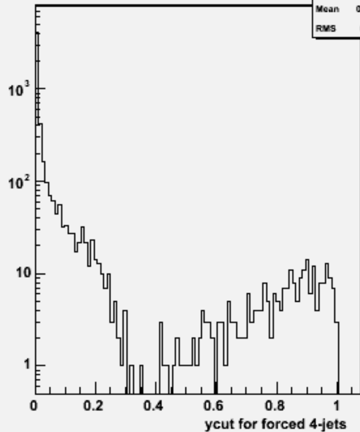
Ycut for 4-jets :w102160 n1n1e2e2e3e3_o
