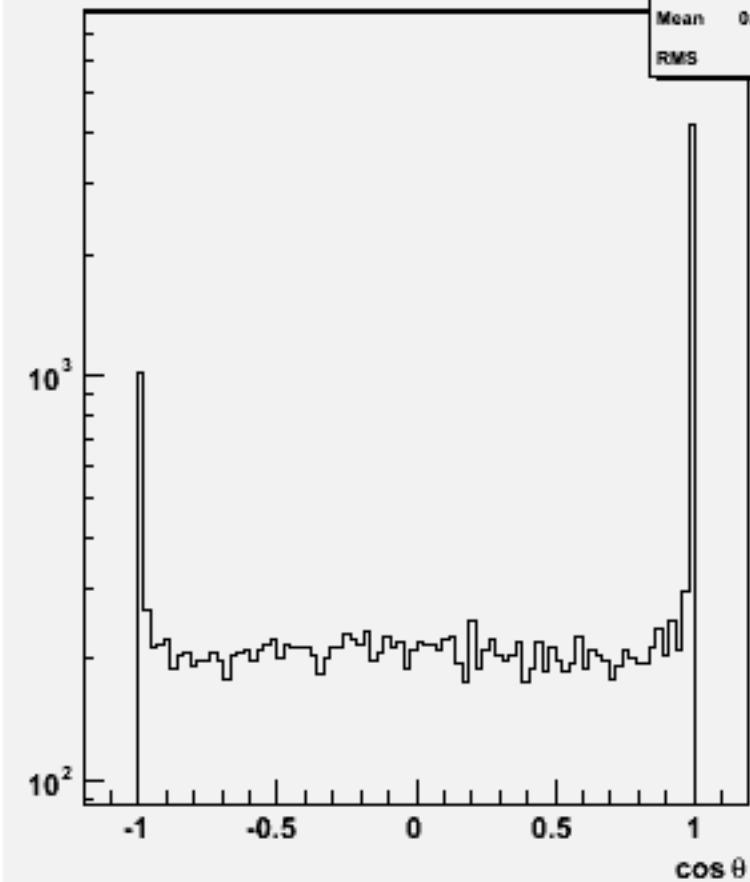
Jet cos \theta (All jets)w102160 n1n1e2e2e3e3_o
