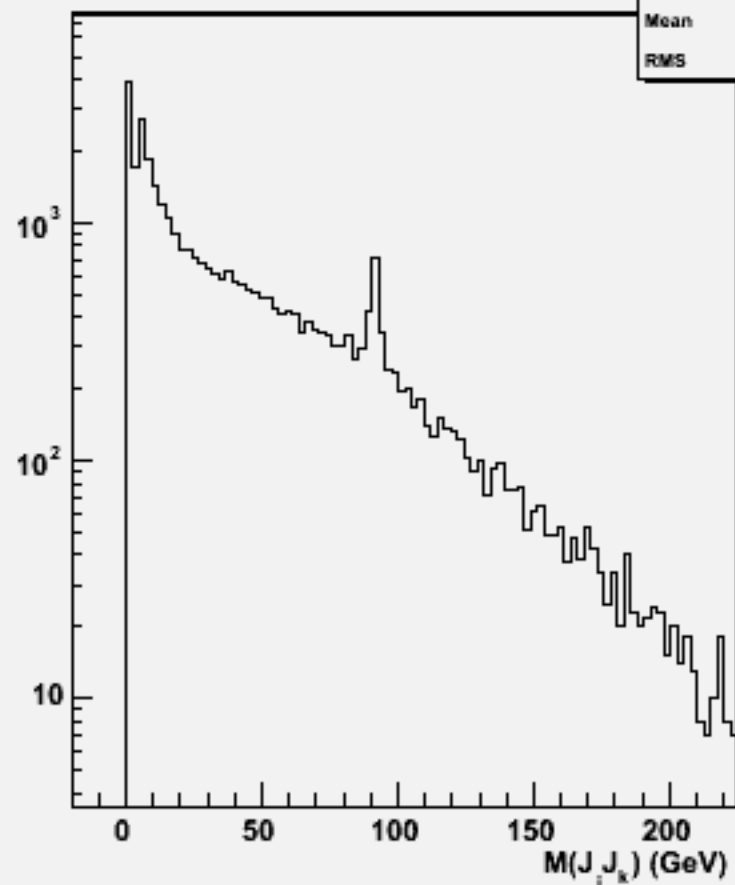
2jets mass(All comb)w102160 n1n1e2e2e3e3_o
