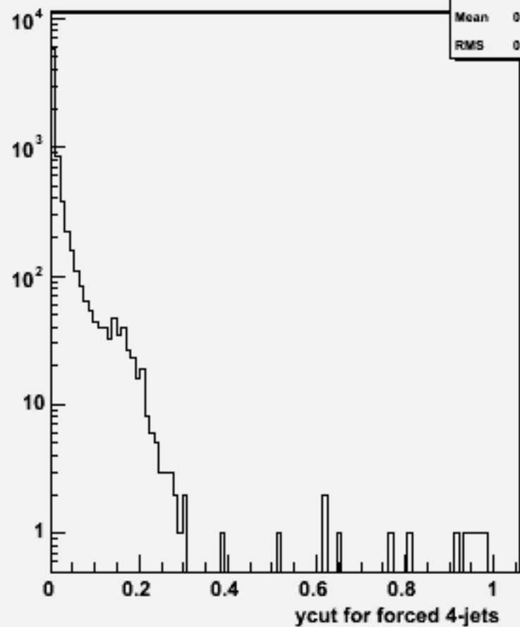
Ycut for 4-jets :w102157 n1n1e2e2e2e2_o
