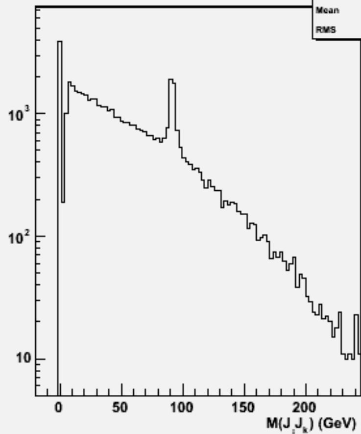
2jets mass(All comb)w102157 n1n1e2e2e2e2_o
