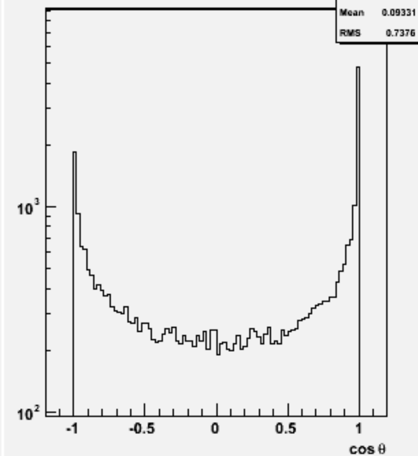
Jet cos \theta (All jets)w102157 n1n1e2e2e2e2_o
