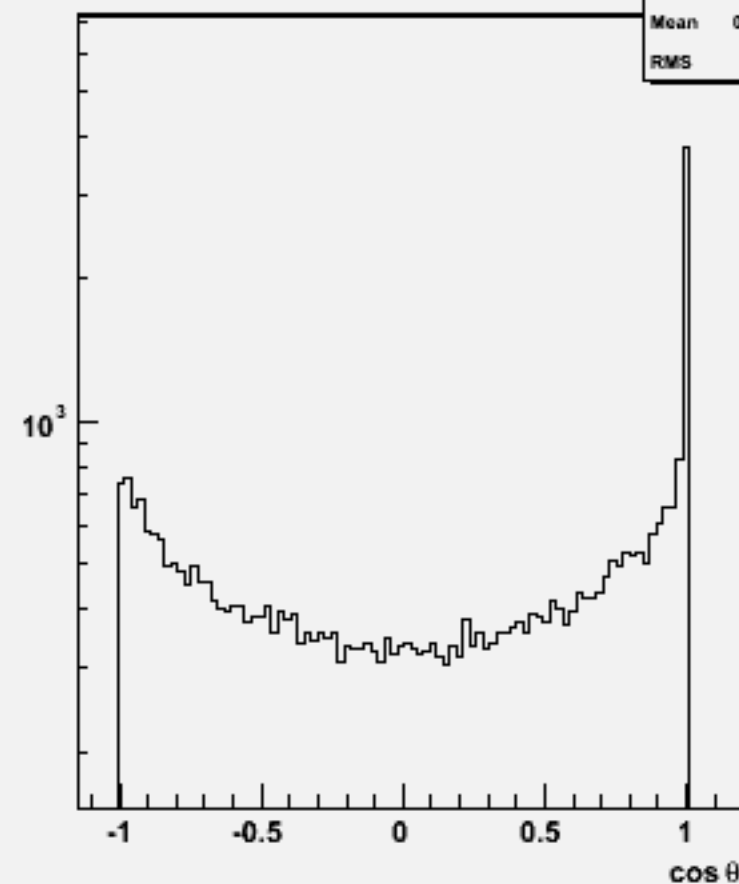
Jet cos \theta (All jets)w102153 cccbb_o
