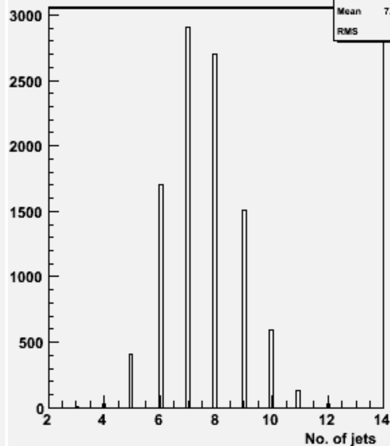
No. jets (ycut=0.001) : w102153 cccbb_o
