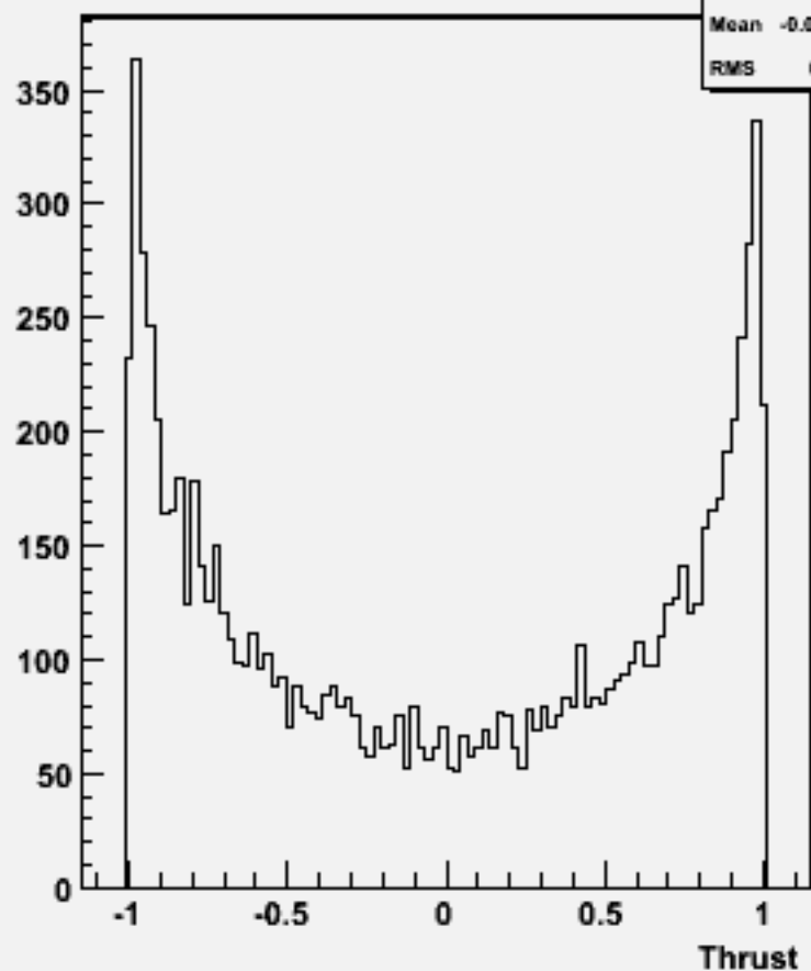
cos \Theta (thrust) w102153 cccbb_o
