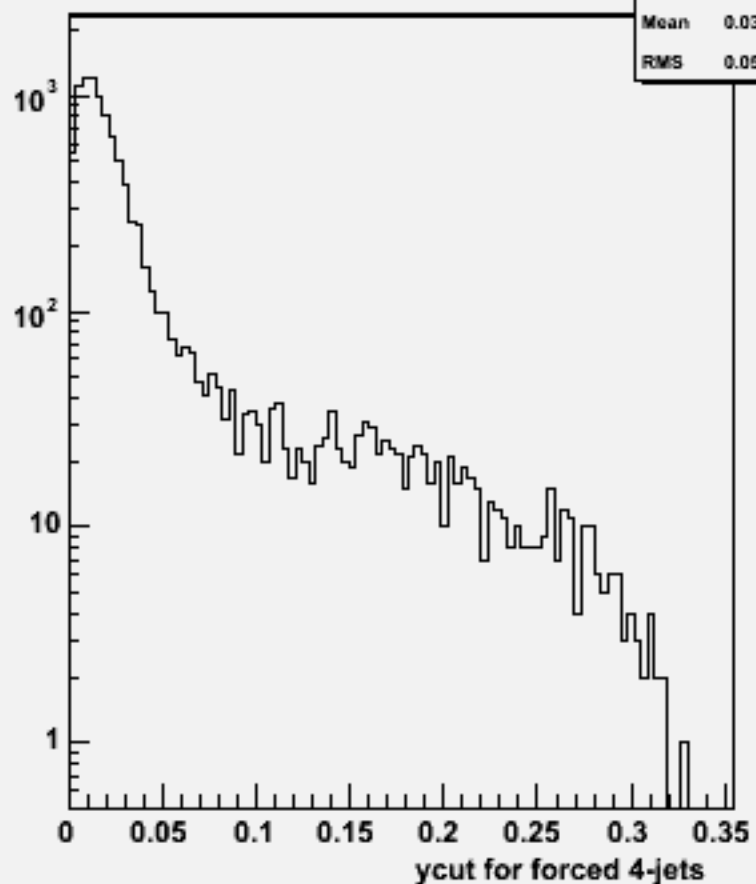
Ycut for 4-jets :w102153 cccbb_o
