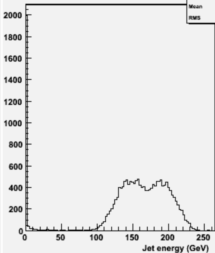
energy for 2-jets :w102153 cccbb_o
