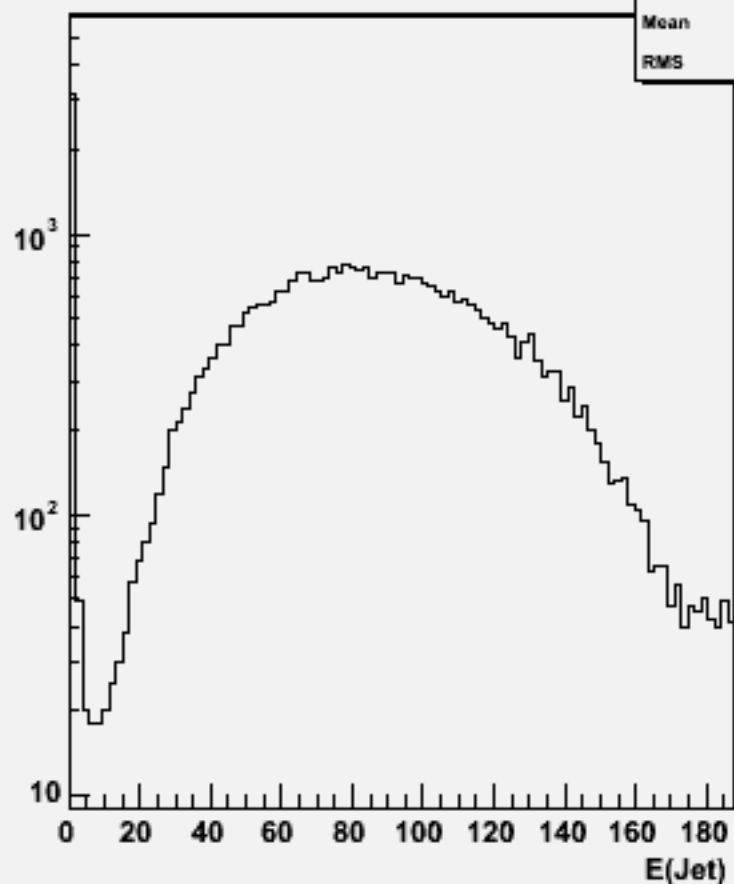
Jet energies(All jets)w102153 cccbb_o
