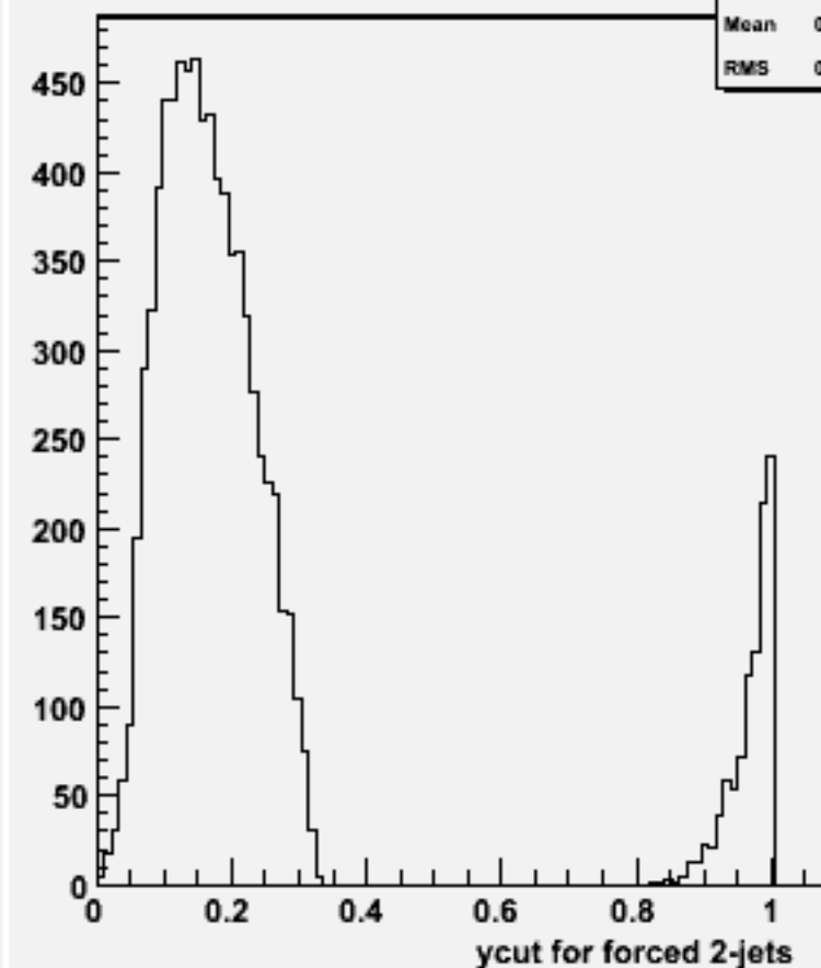
Ycut for 2-jets :w102153 cccbb_o
