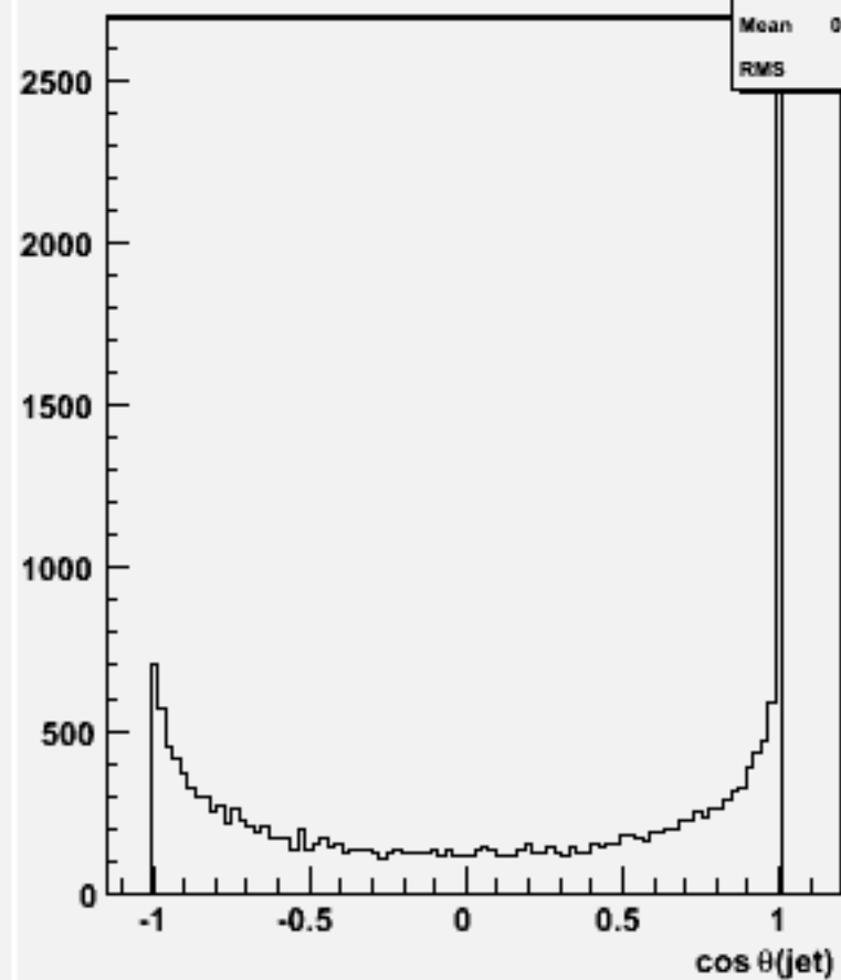
cos \theta for 2-jets :w102153 cccbb_o
