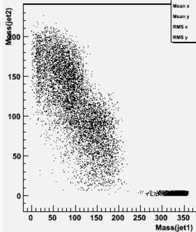
Jet mass for forced 2-jets : w102153 cccbb_o
