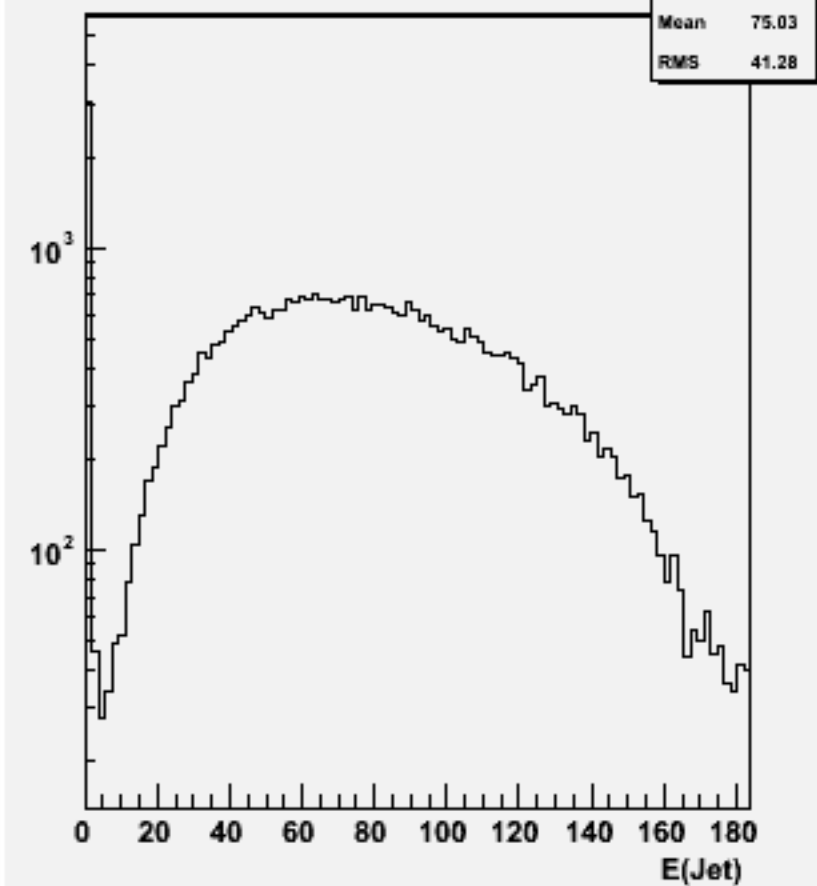
Jet energies(All jets)w102144 cccce3e3_o
