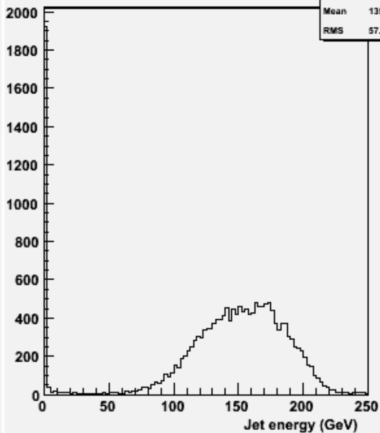
energy for 2-jets :w102144 cccce3e3_o
