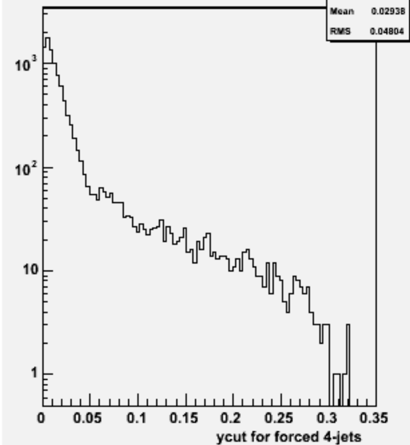
Ycut for 4-jets :w102144 cccce3e3_o
