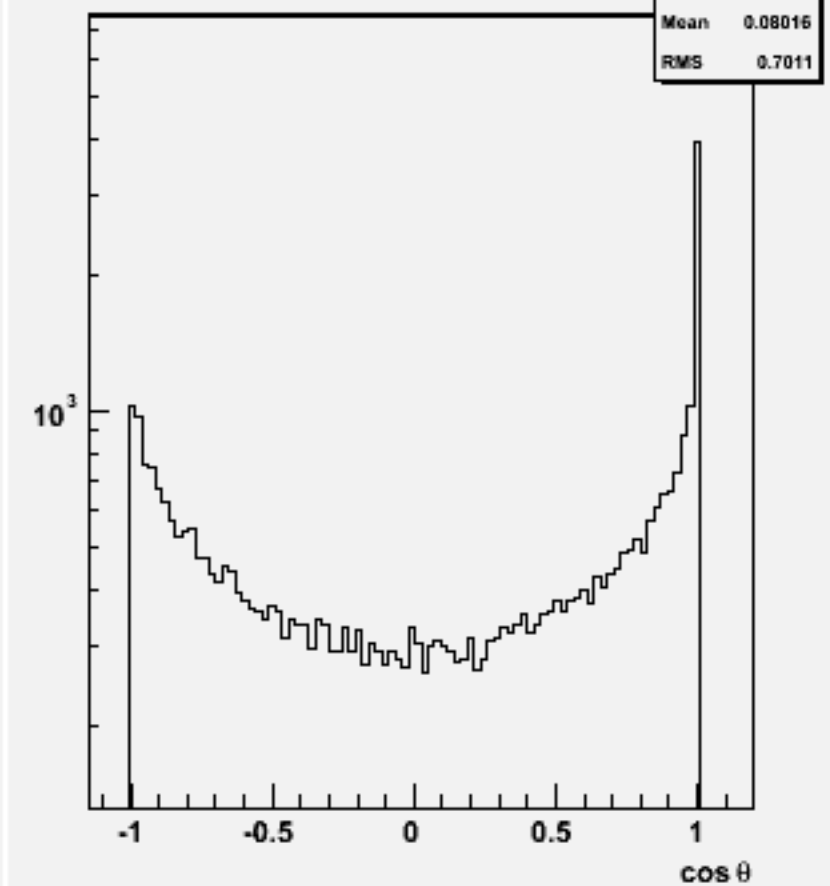
Jet cosθ (All jets)w102144 cccce3e3_o
