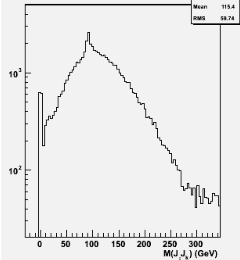
2jets mass(All comb)w102144 cccce3e3_o
