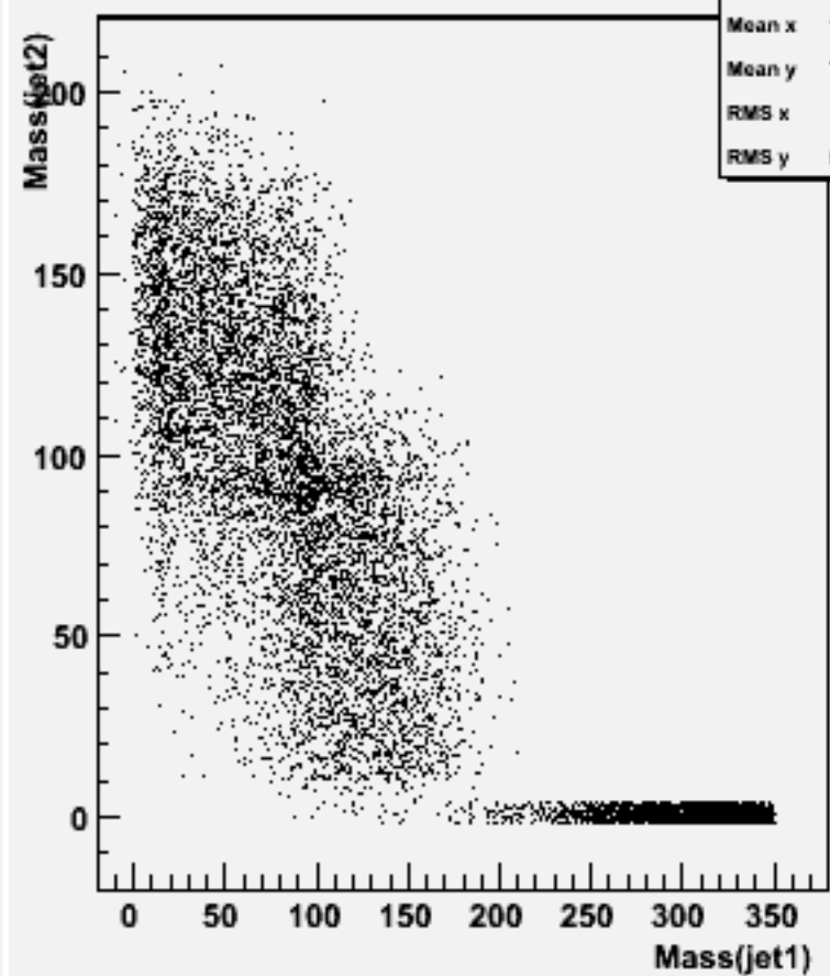
Jet mass for forced 2-jets : w102144 cccce3e3_o
