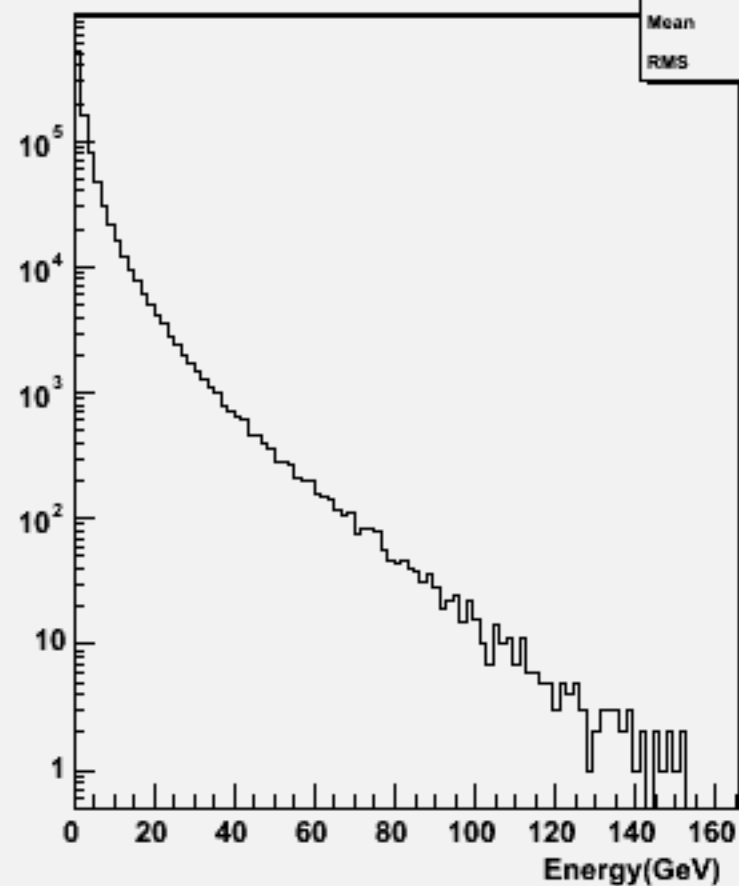
Particle Energy : w102144 cccce3e3_o
