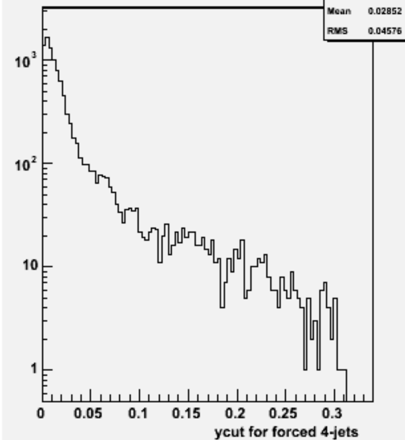
Ycut for 4-jets :w102141 cccce2e2_o
