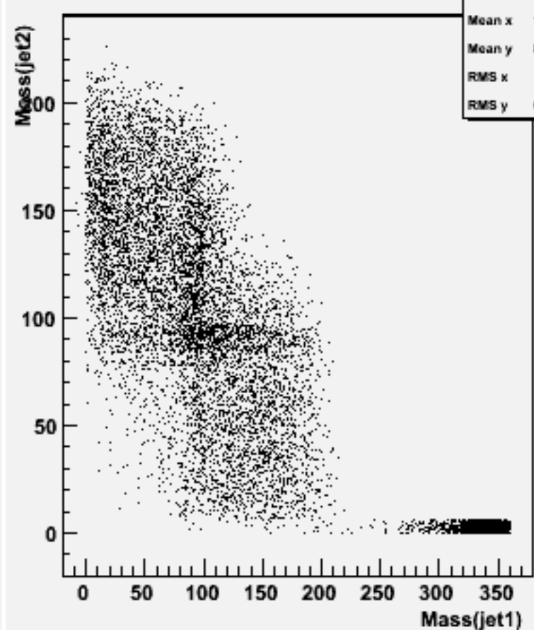
Jet mass for forced 2-jets : w102141 cccce2e2_o
