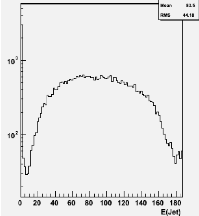
Jet energies(All jets)w102141 cccce2e2_o
