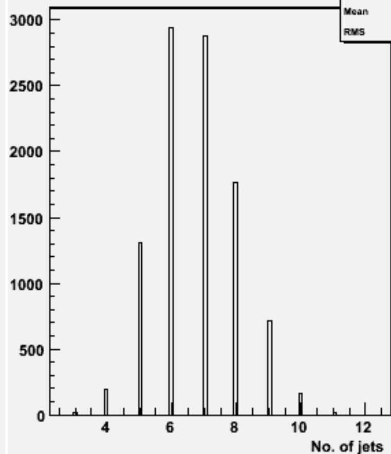
No. jets (ycut=0.001) : w102141 cccce2e2_o
