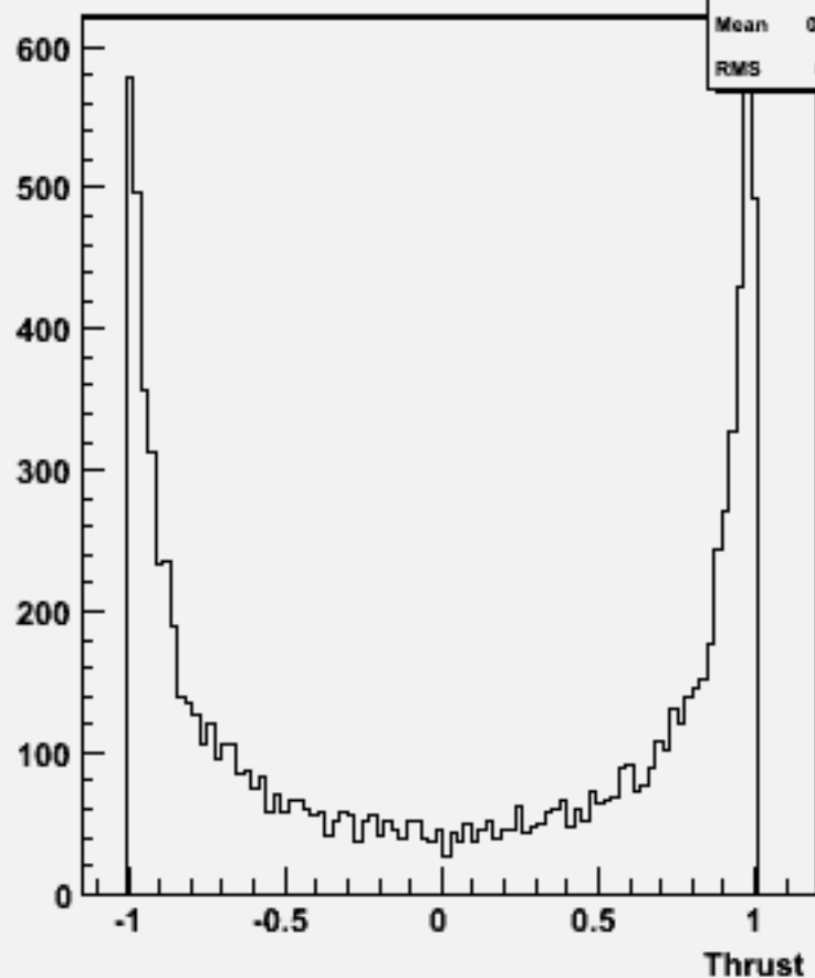
cos \Theta (thrust) w102141 cccce2e2_o
