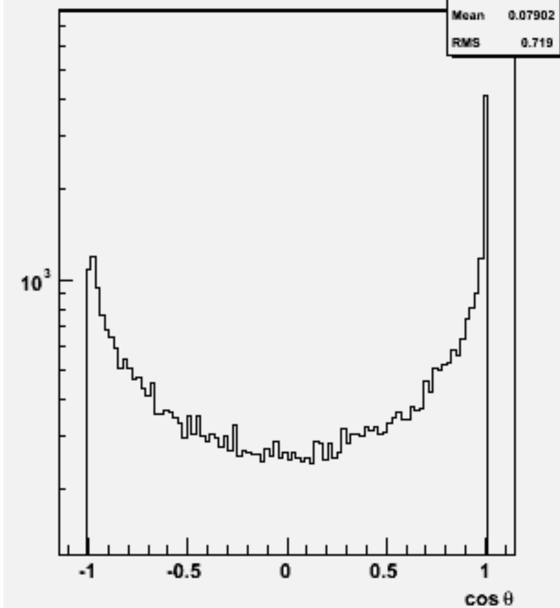
Jet cosθ (All jets)w102141 cccce2e2_o
