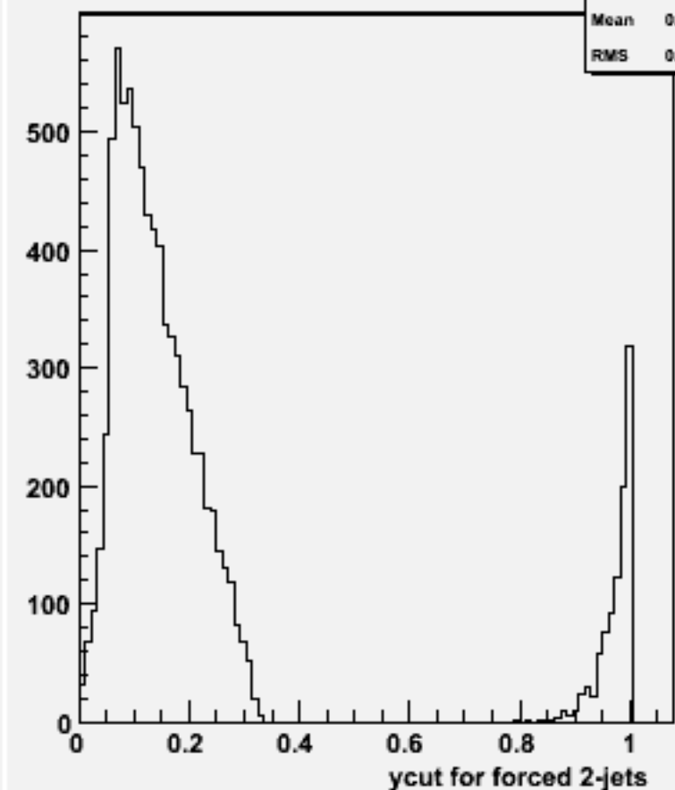
Ycut for 2-jets :w102141 cccce2e2_o
