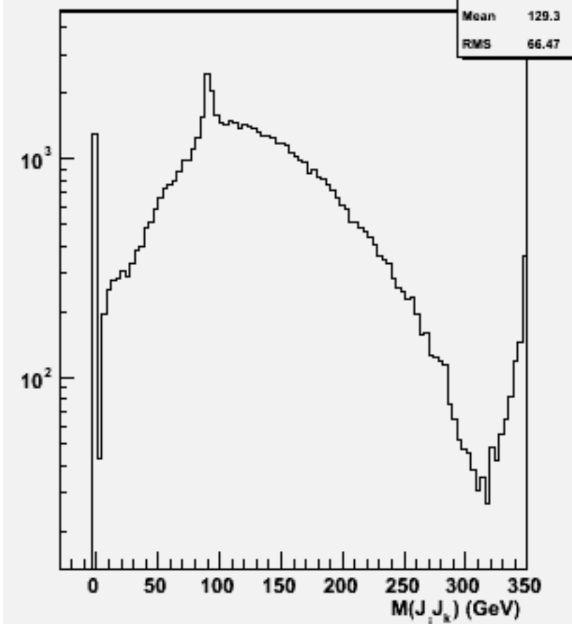
2jets mass(All comb)w102141 cccce2e2_o
