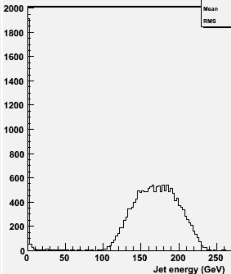
energy for 2-jets :w102141 cccce2e2_o
