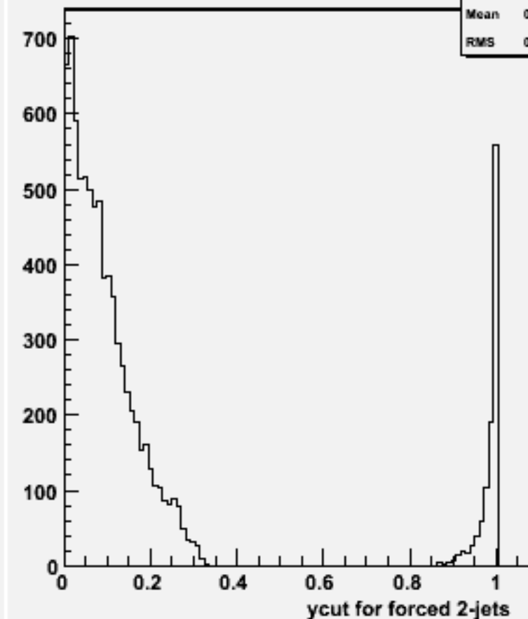
Ycut for 2-jets :w102138 cccce1e1_o
