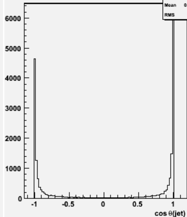
cos \theta for 2-jets :w102138 cccce1e1_o
