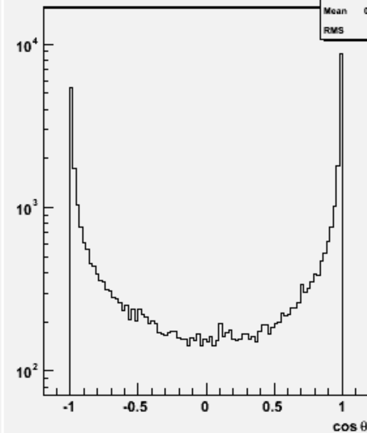
Jet cosθ (All jets)w102138 cccce1e1_o
