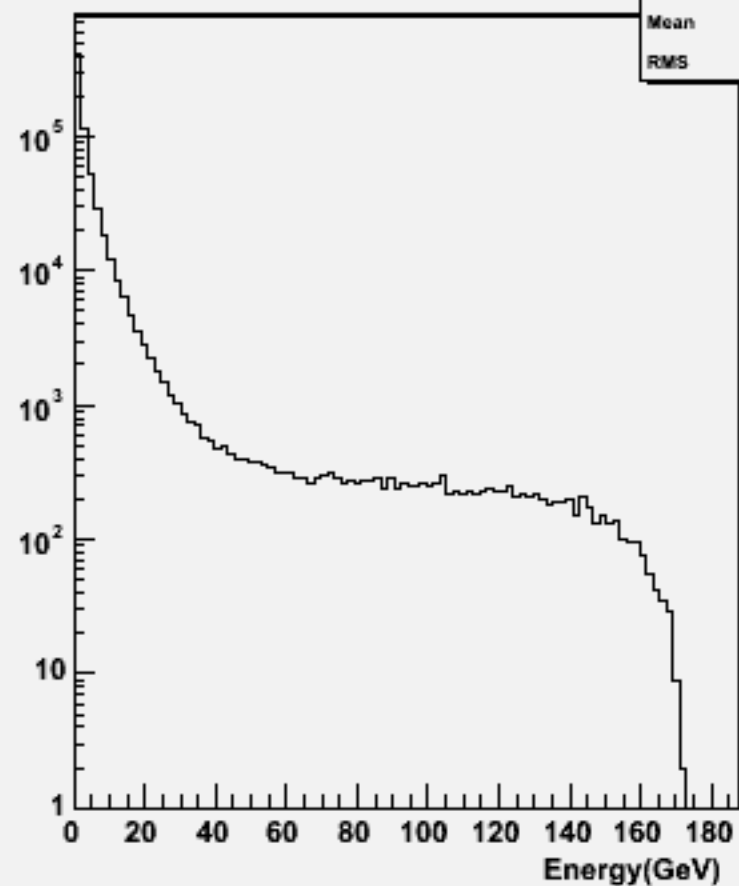
Particle Energy : w102138 cccce1e1_o
