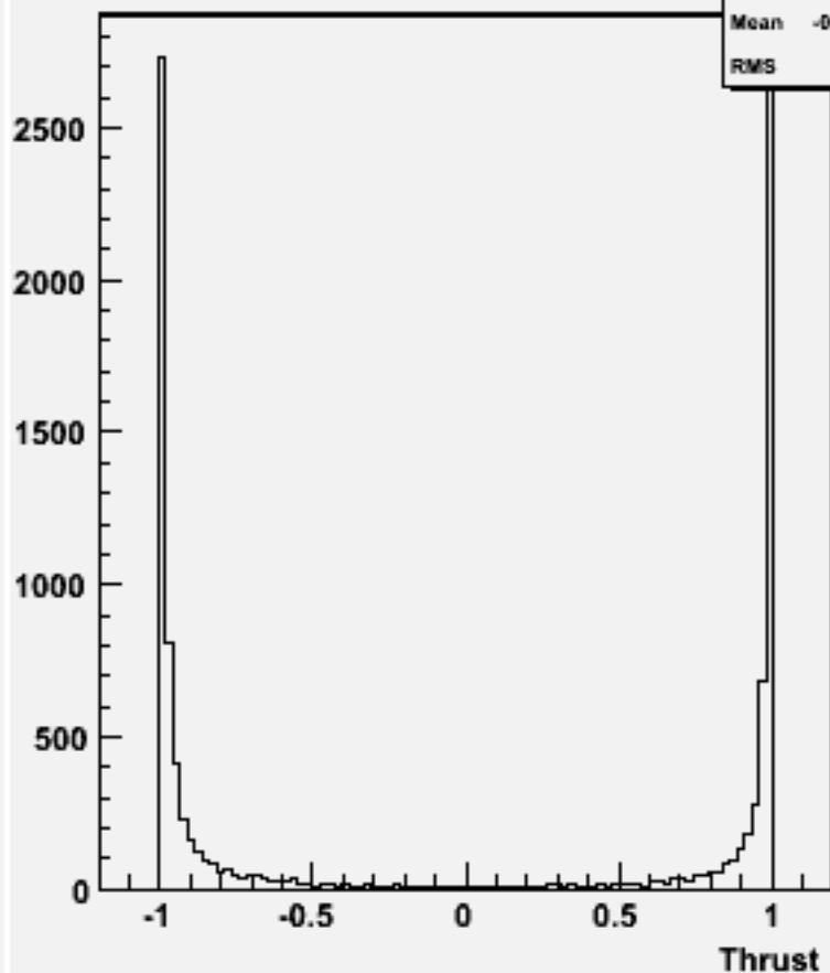
cos \Theta (thrust) w102138 cccce1e1_o
