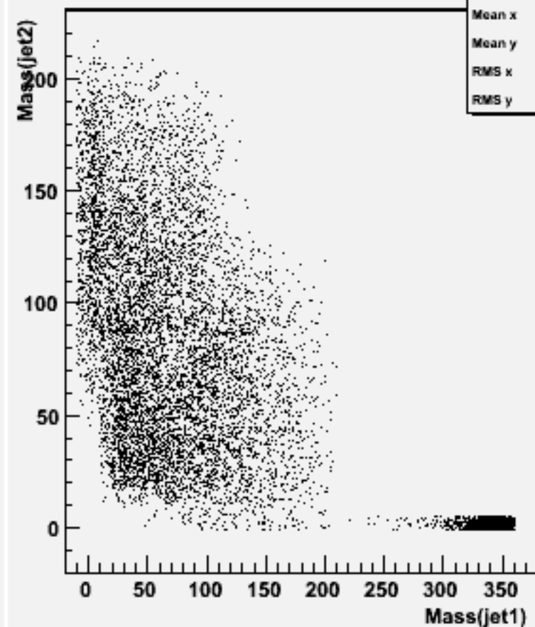
Jet mass for forced 2-jets : w102138 cccce1e1_o
