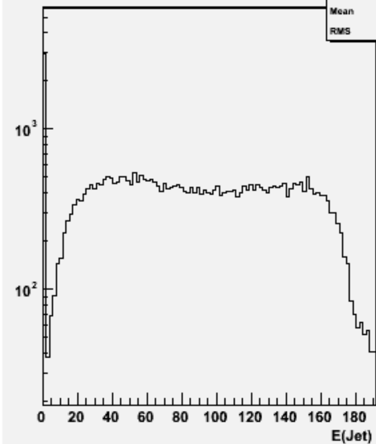
Jet energies(All jets)w102138 cccce1e1_o
