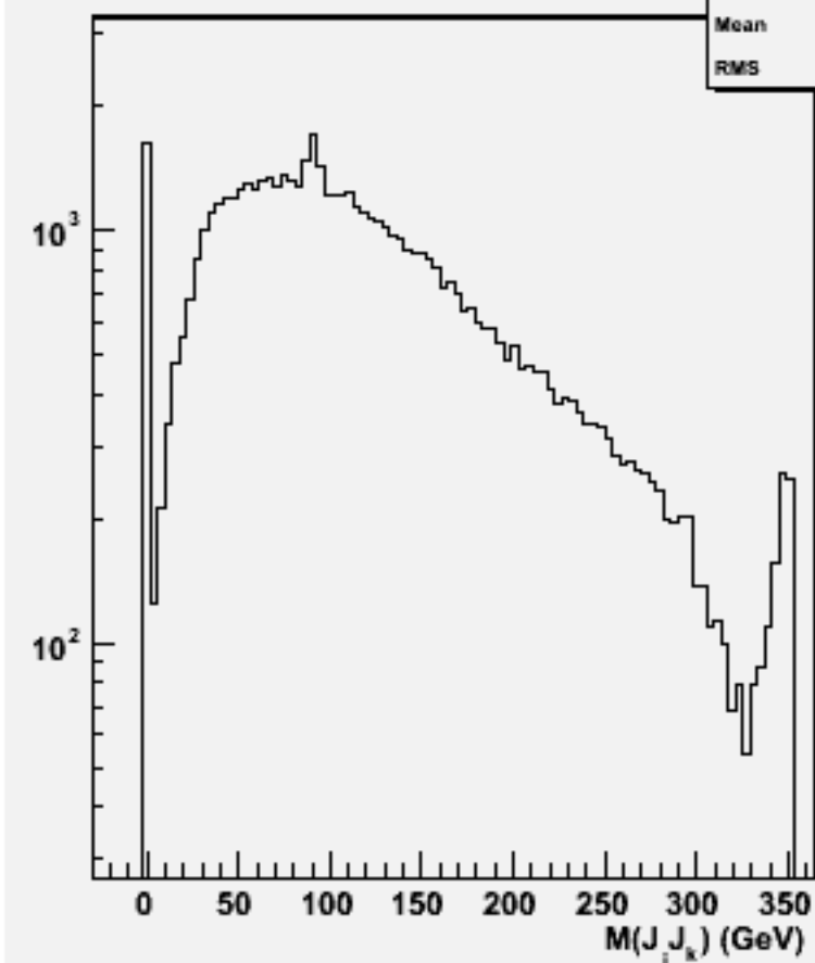
2jets mass(All comb)w102138 cccce1e1_o
