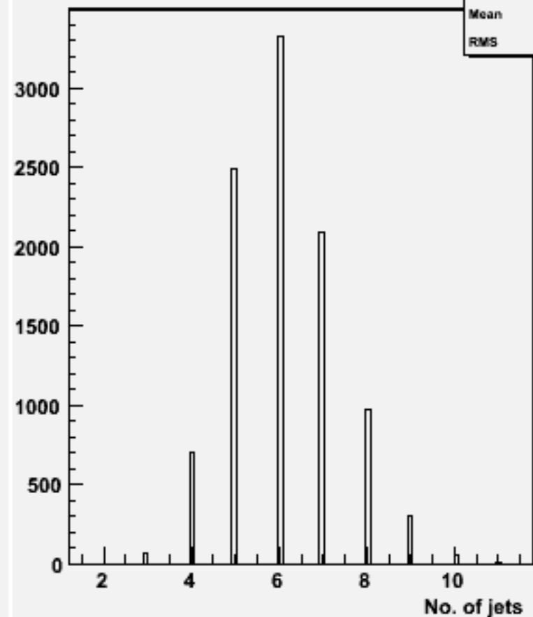
No. jets (ycut=0.001) : w102138 cccce1e1_o
