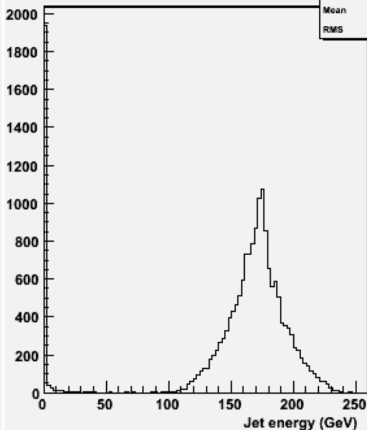
energy for 2-jets :w102138 cccce1e1_o
