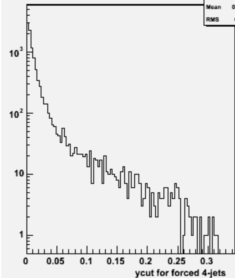
Ycut for 4-jets :w102138 cccce1e1_o
