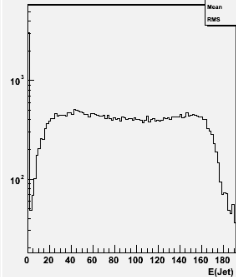
Jet energies(All jets)w102135 cccce1e1_o
