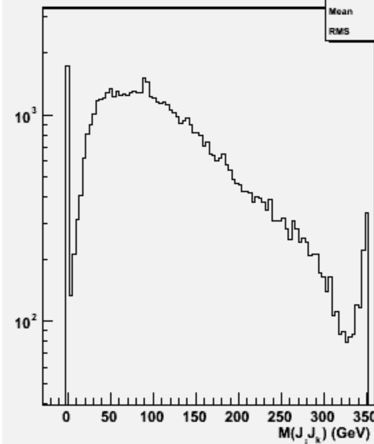
2jets mass(All comb)w102135 cccce1e1_o
