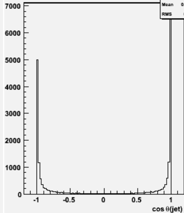
cos \theta for 2-jets :w102135 cccce1e1_o
