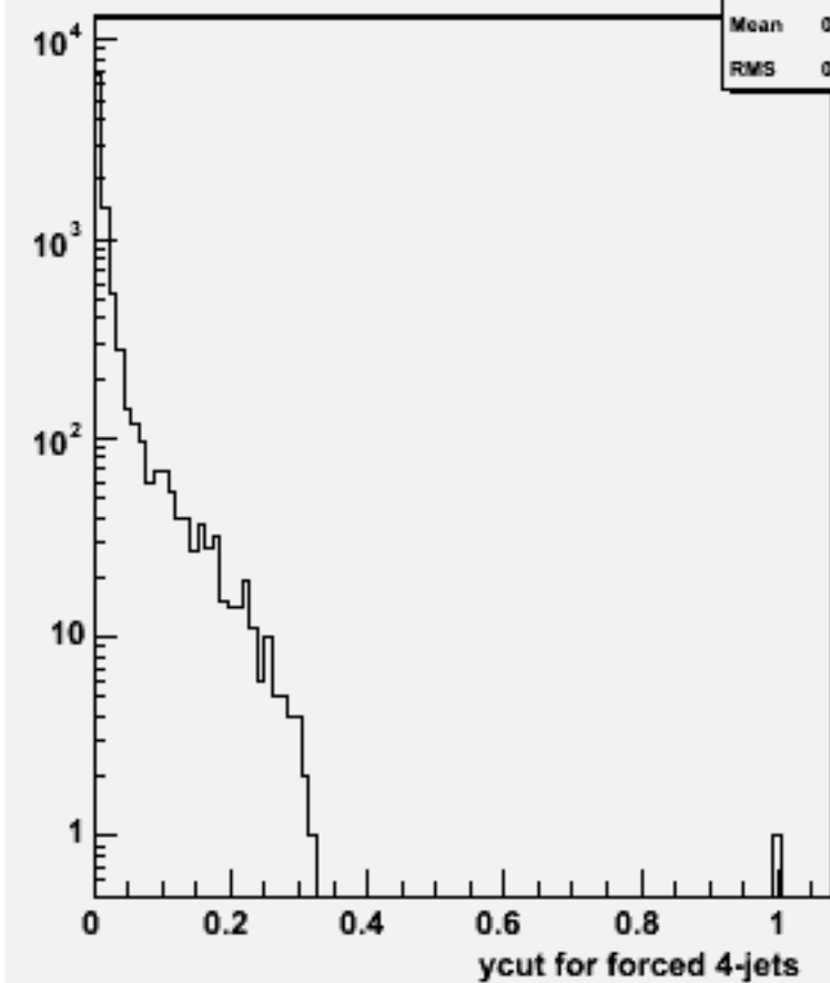
Ycut for 4-jets :w102135 cccce1e1_o
