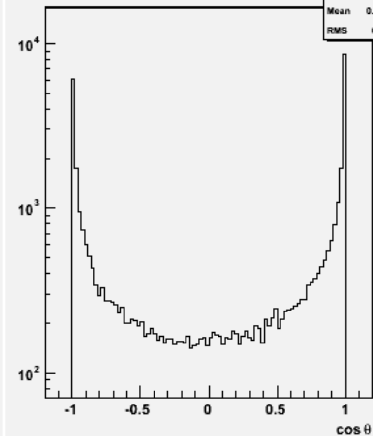
Jet cosθ (All jets)w102135 cccce1e1_o
