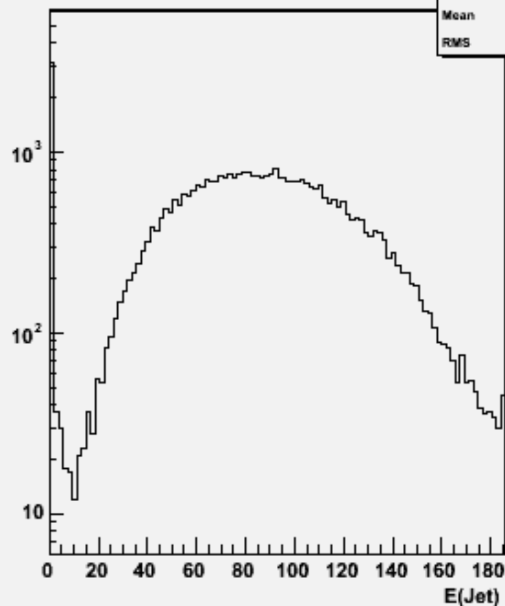
Jet energies(All jets)w102132 uuccbb_o
