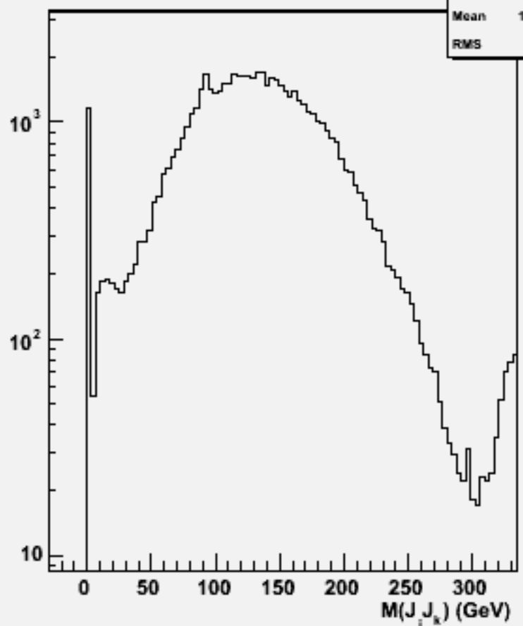
2jets mass(All comb)w102132 uuccbb_o
