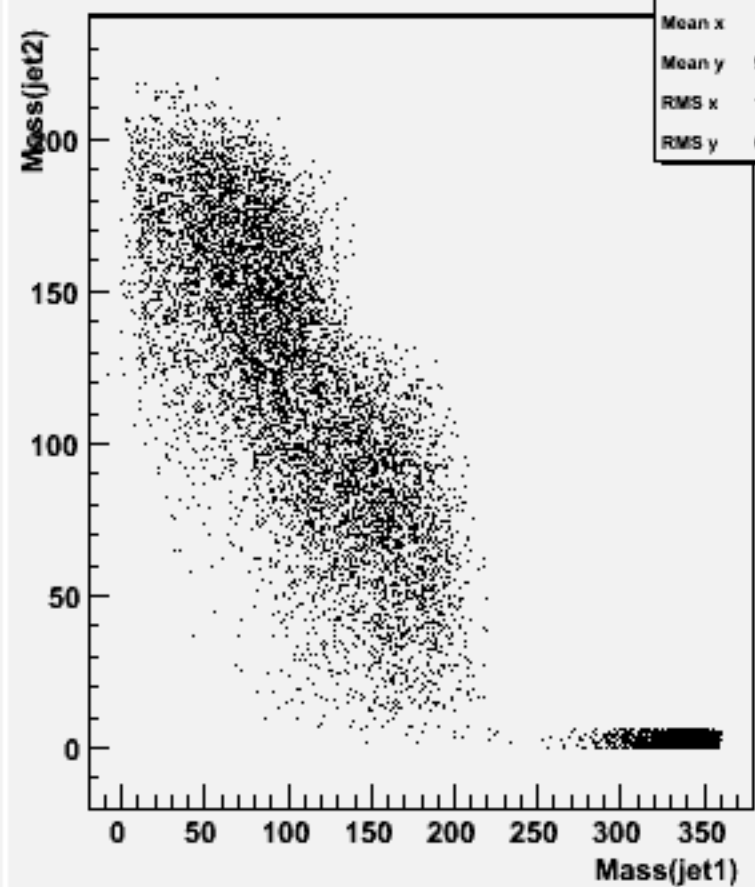
Jet mass for forced 2-jets : w102132 uuccbb_o
