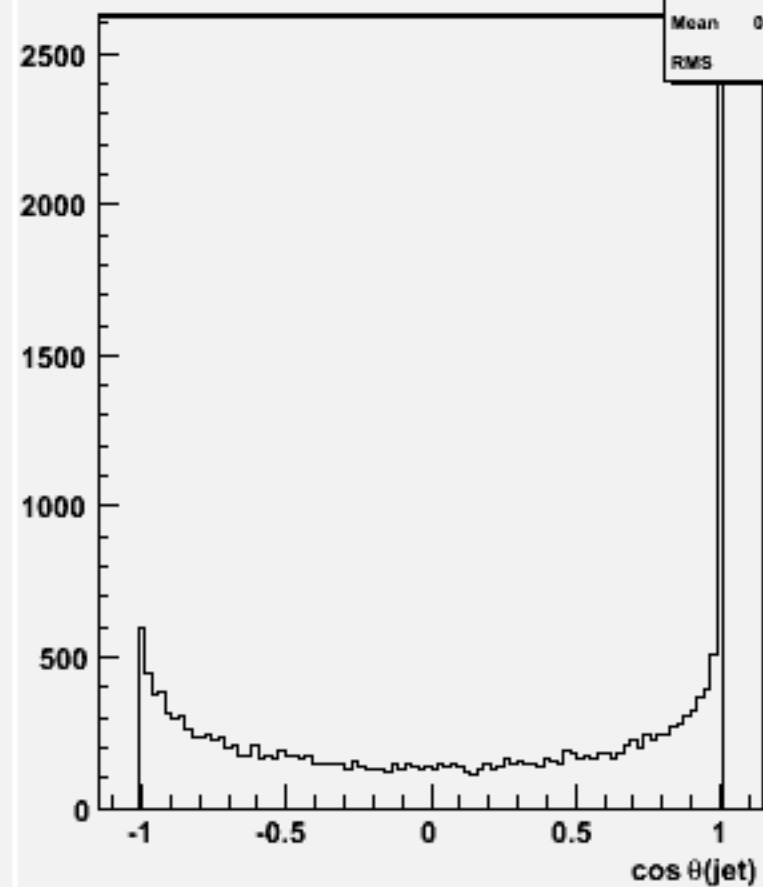
cos \theta for 2-jets :w102132 uuccbb_o
