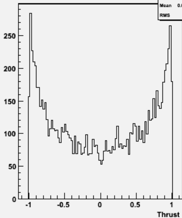
cos \Theta (thrust) w102132 uuccbb_o
