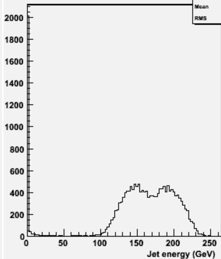
energy for 2-jets :w102132 uuccbb_o
