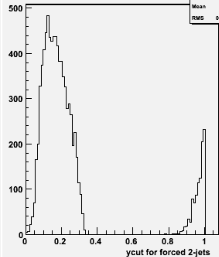
Ycut for 2-jets :w102132 uuccbb_o
