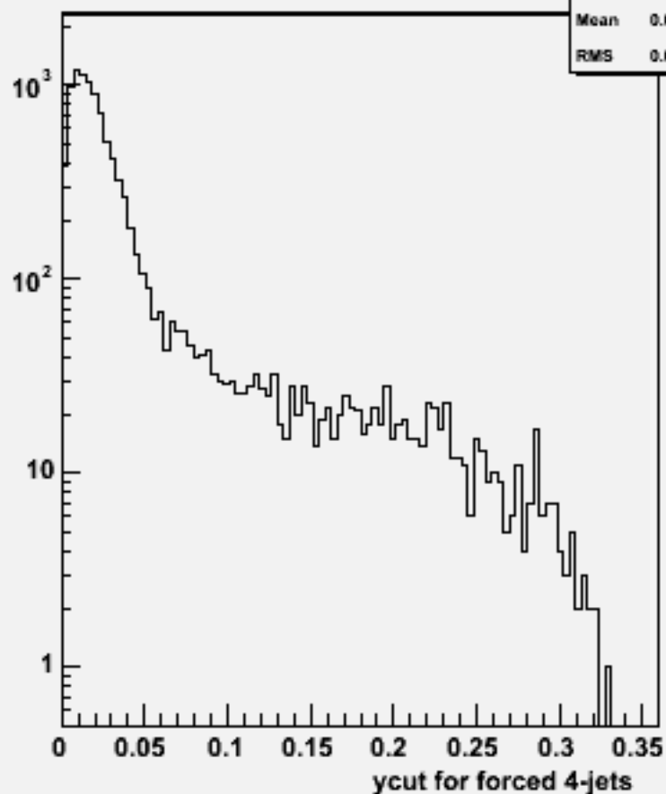
Ycut for 4-jets :w102132 uuccbb_o
