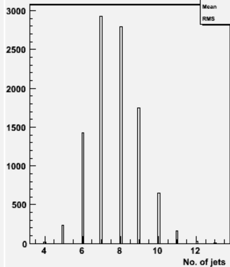
No. jets (ycut=0.001) : w102132 uuccbb_o
