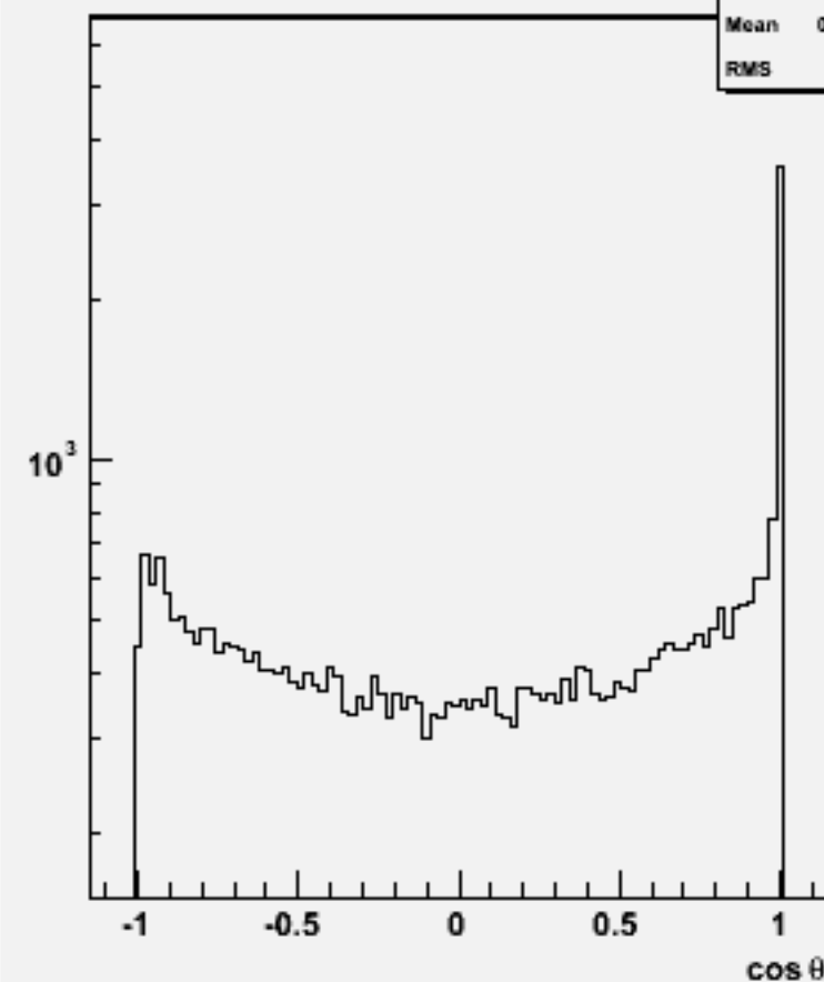
Jet cos \theta (All jets)w102132 uuccbb_o
