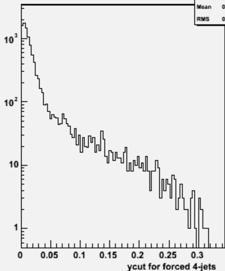
Ycut for 4-jets :w102129 uucce3e3_o
