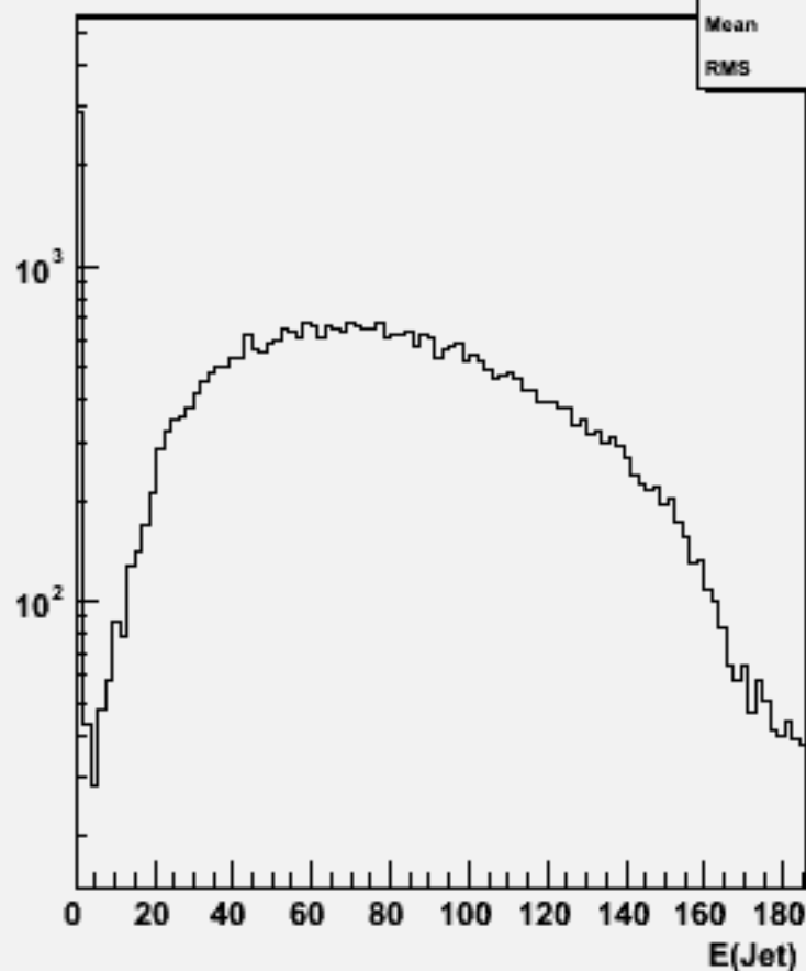
Jet energies(All jets)w102129 uucce3e3_o
