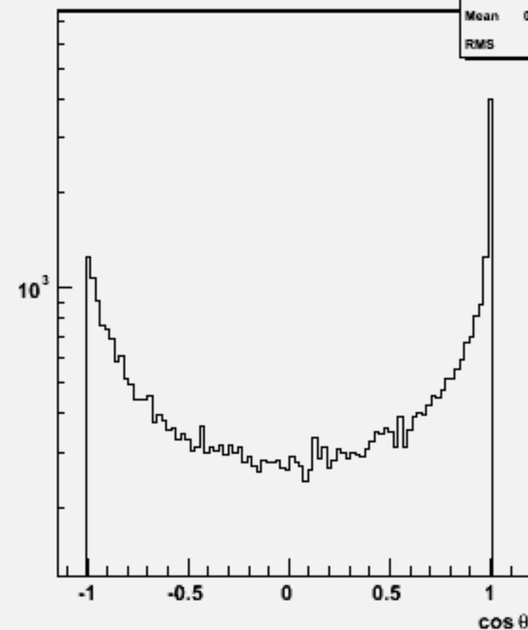
Jet cosθ (All jets)w102129 uucce3e3_o
