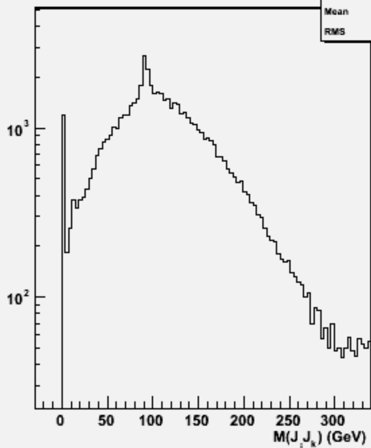
2jets mass(All comb)w102129 uucce3e3_o
