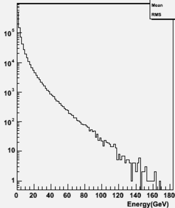
Particle Energy : w102129 uucce3e3_o
