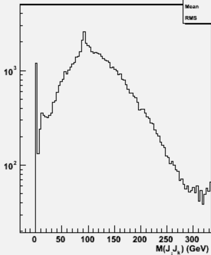
2jets mass(All comb)w102128 uucce3e3_o
