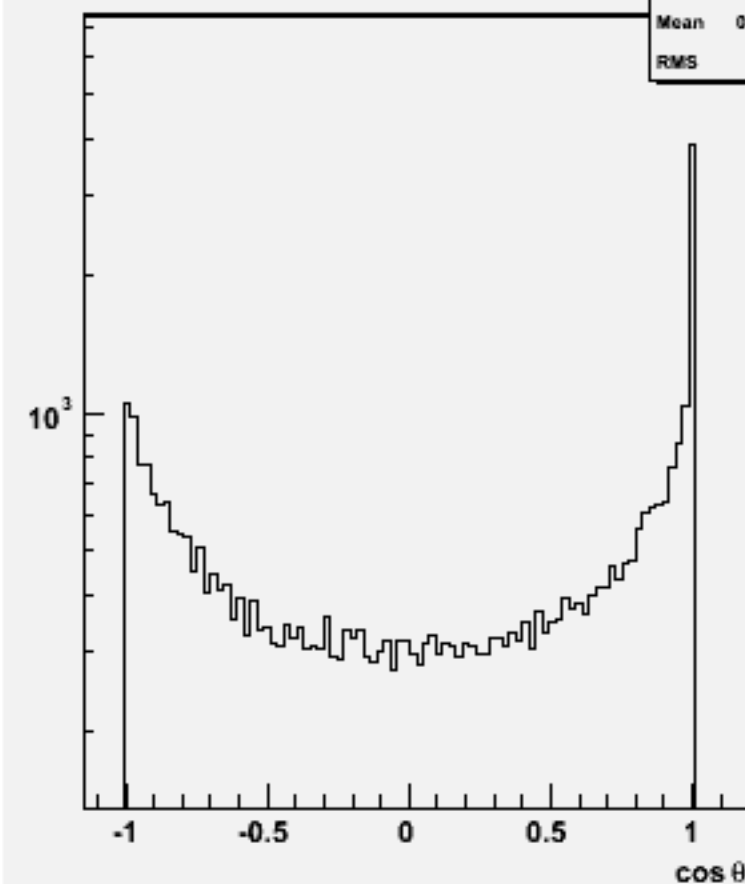
Jet cosθ (All jets)w102128 uucce3e3_o
