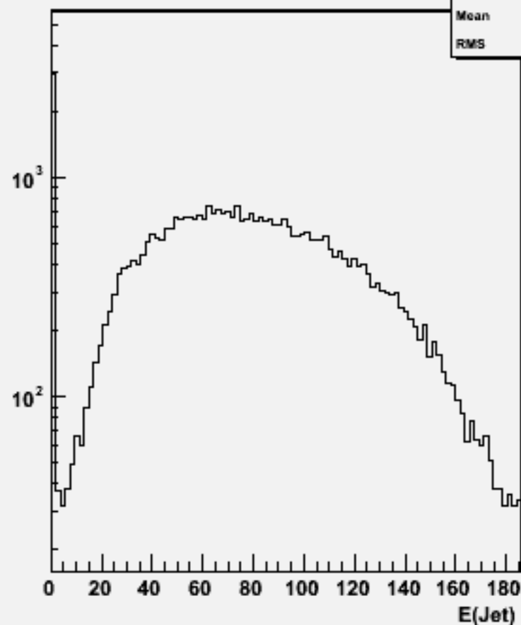
Jet energies(All jets)w102128 uucce3e3_o
