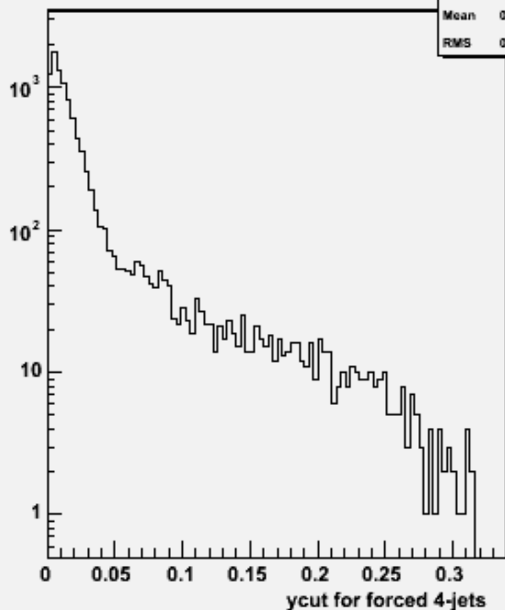
Ycut for 4-jets :w102128 uucce3e3_o
