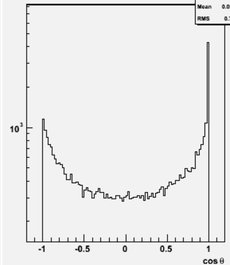
Jet cosθ (All jets)w102124 uucce2e2_o
