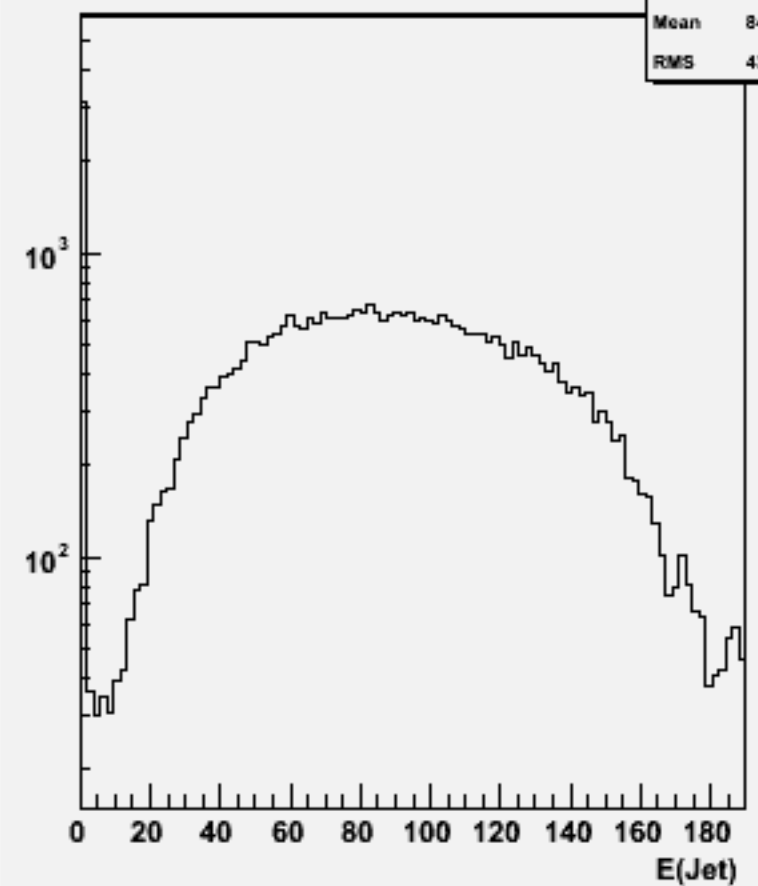
Jet energies(All jets)w102124 uucce2e2_o
