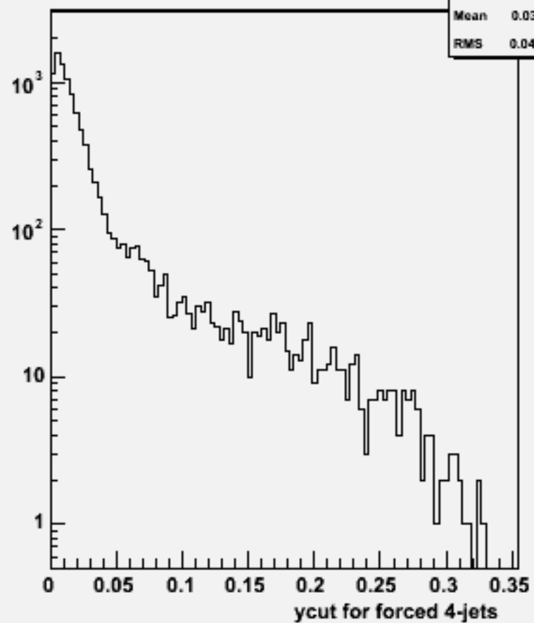
Ycut for 4-jets :w102124 uucce2e2_o
