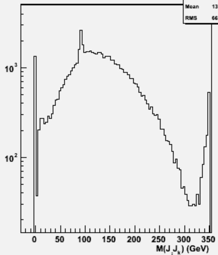
2jets mass(All comb)w102124 uucce2e2_o
