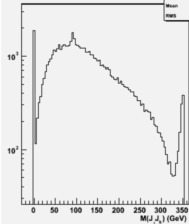
2jets mass(All comb)w102122 uucce1e1_o
