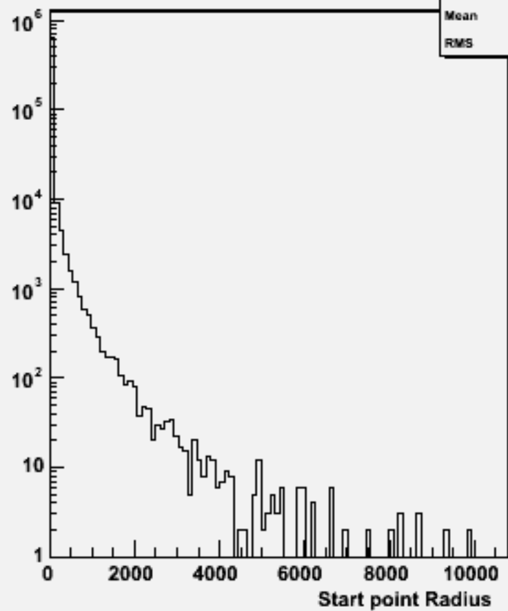
Start point R : w102122 uucce1e1_o
