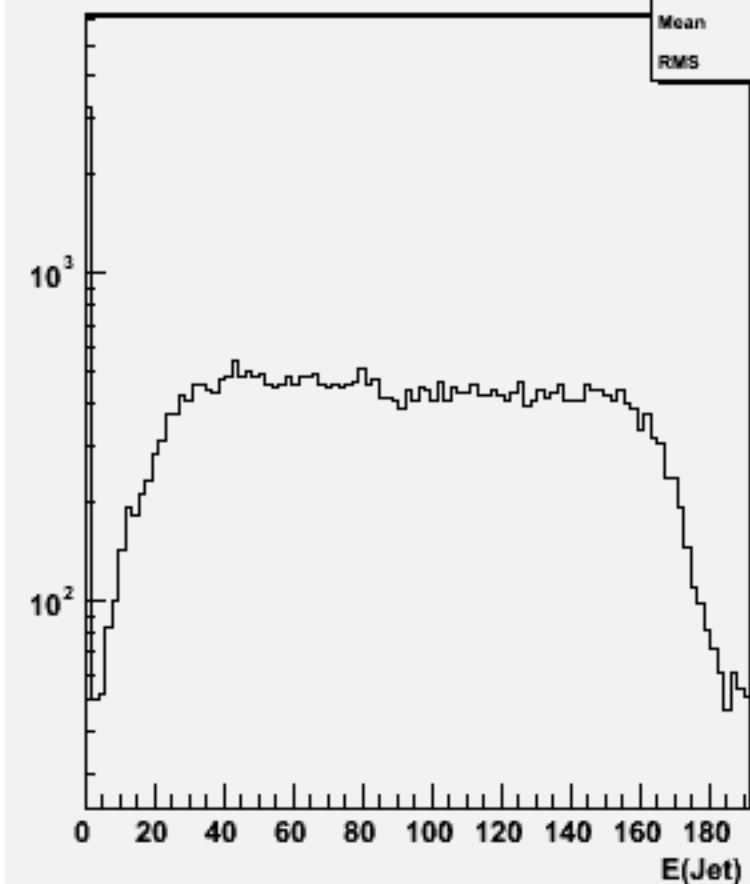
Jet energies(All jets)w102122 uucce1e1_o
