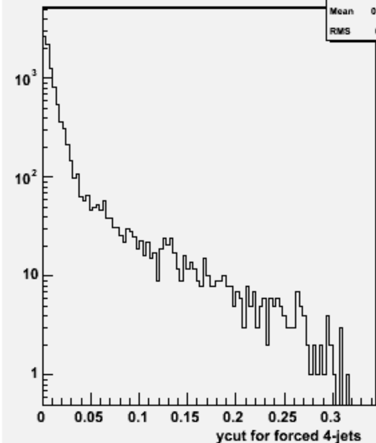
Ycut for 4-jets :w102122 uucce1e1_o
