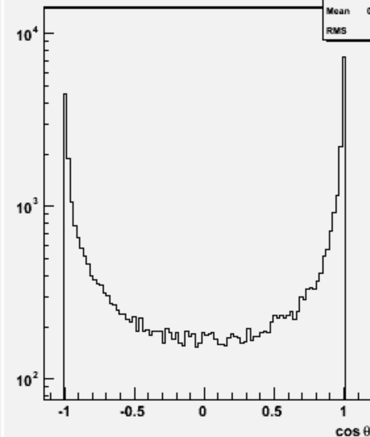
Jet cosθ (All jets)w102122 uucce1e1_o
