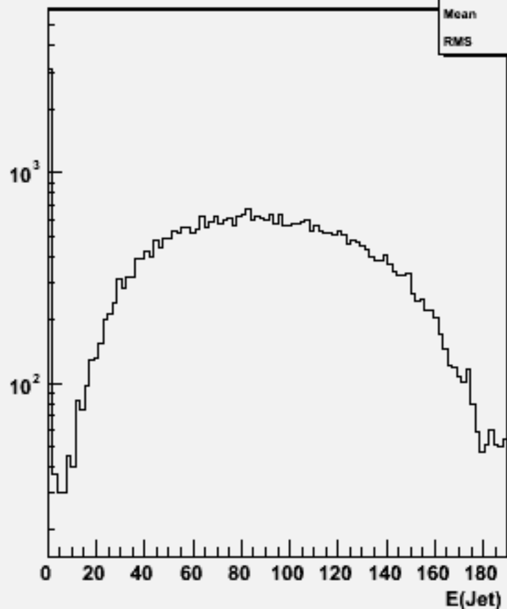
Jet energies(All jets)w102120 uucce1e1_o
