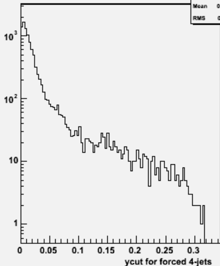
Ycut for 4-jets :w102120 uucce1e1_o
