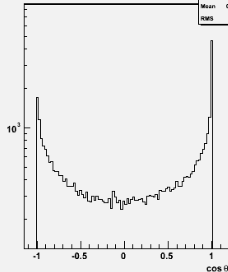
Jet cosθ (All jets)w102120 uucce1e1_o
