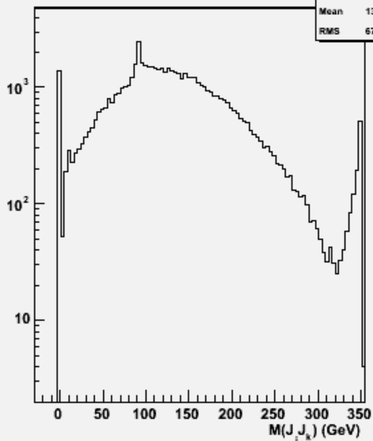
2jets mass(All comb)w102120 uucce1e1_o
