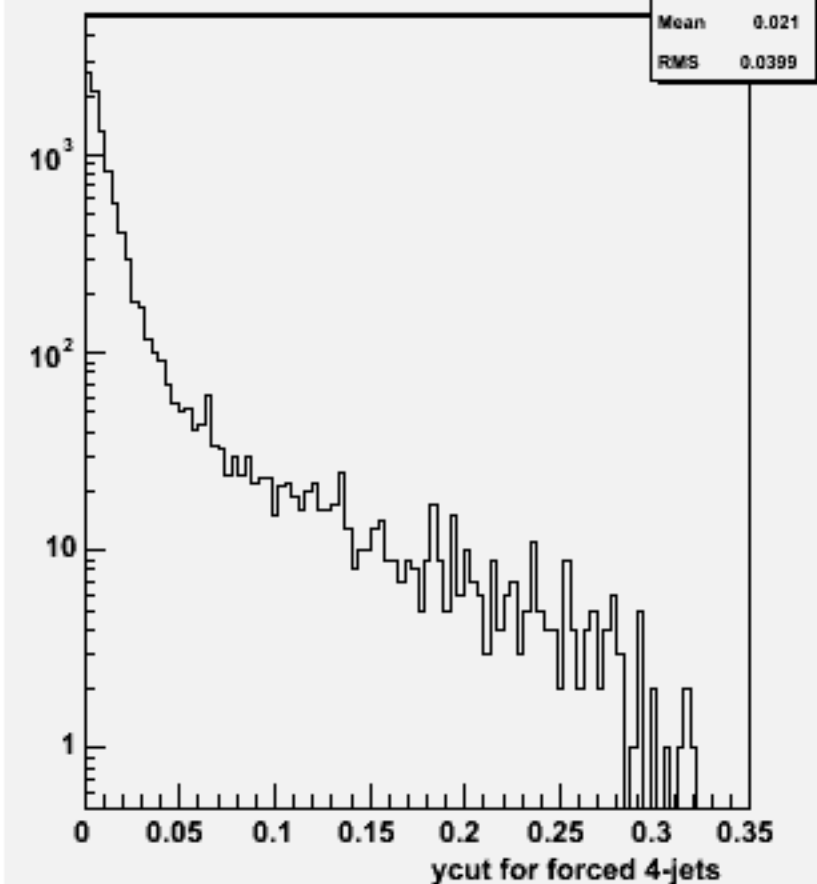
Ycut for 4-jets :w102119 uucce1e1_o
