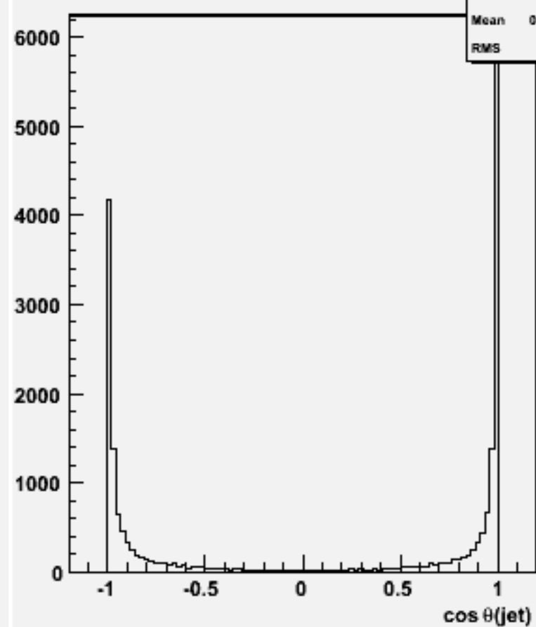
cos \theta for 2-jets :w102119 uucce1e1_o
