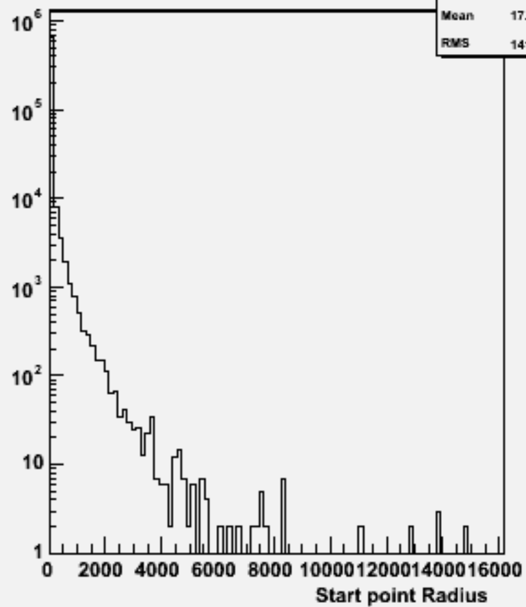
Start point R : w102119 uucce1e1_o
