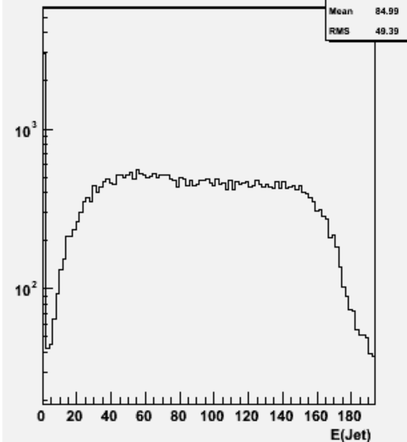
Jet energies(All jets)w102119 uucce1e1_o
