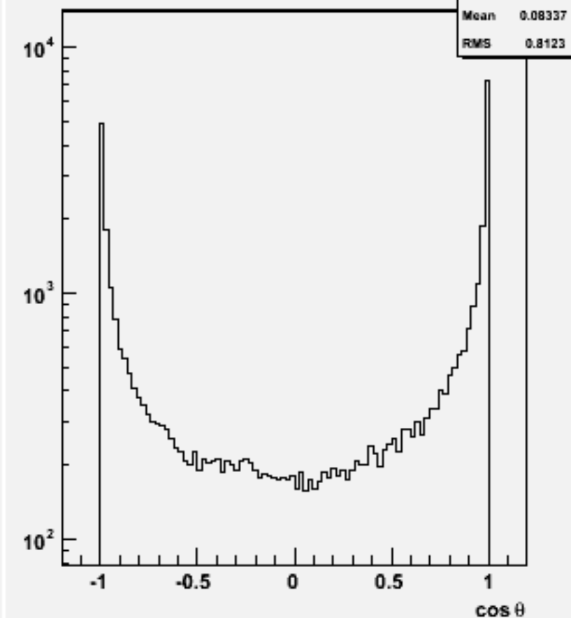
Jet cosθ (All jets)w102119 uucce1e1_o
