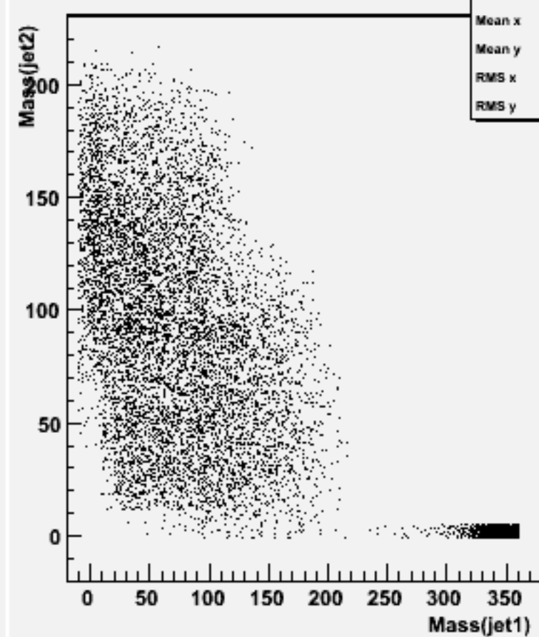
Jet mass for forced 2-jets : w102119 uucce1e1_o
