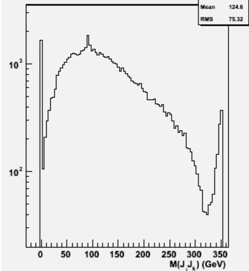
2jets mass(All comb)w102119 uucce1e1_o
