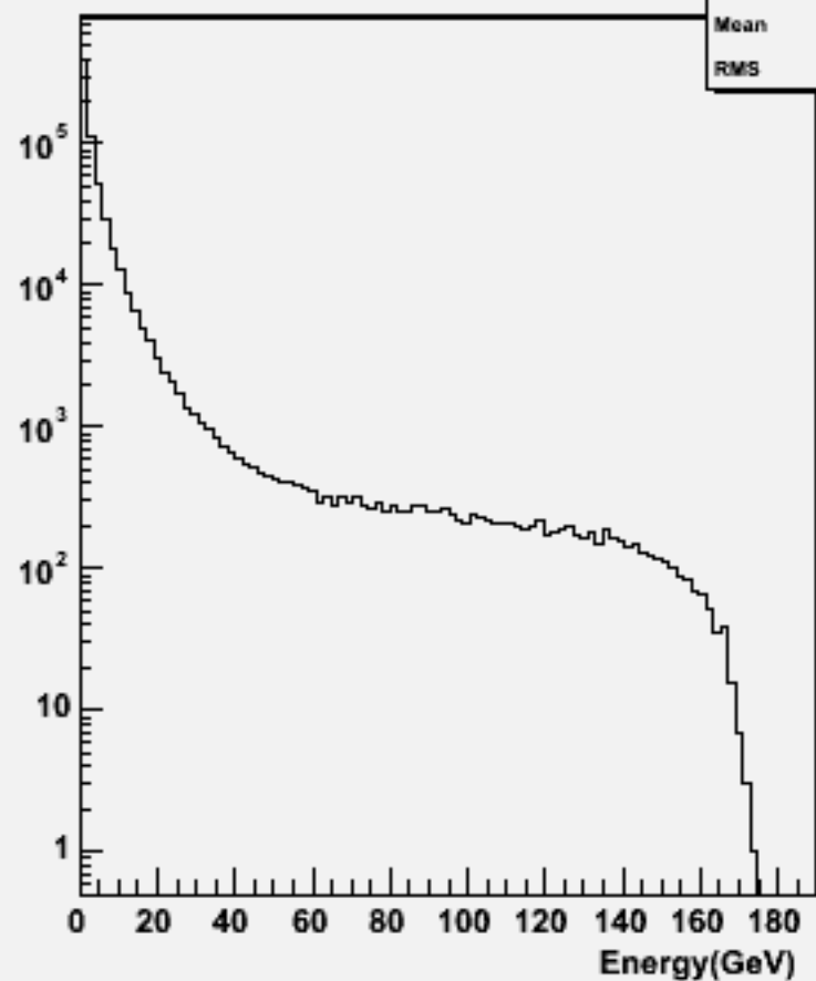
Start point R : w102119 uucce1e1_o
