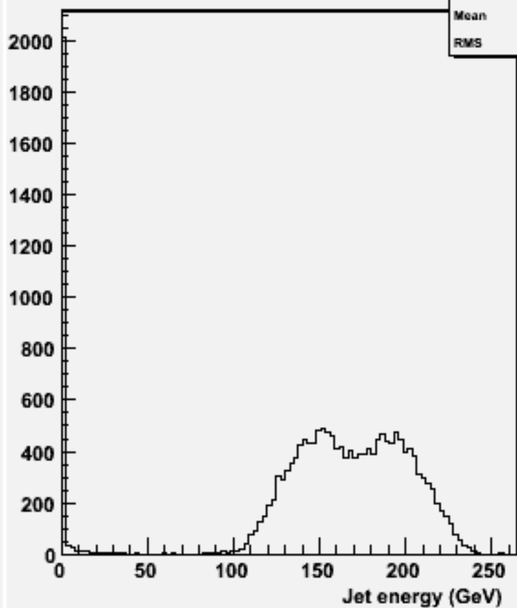
energy for 2-jets :w102117 uuuubb_o
