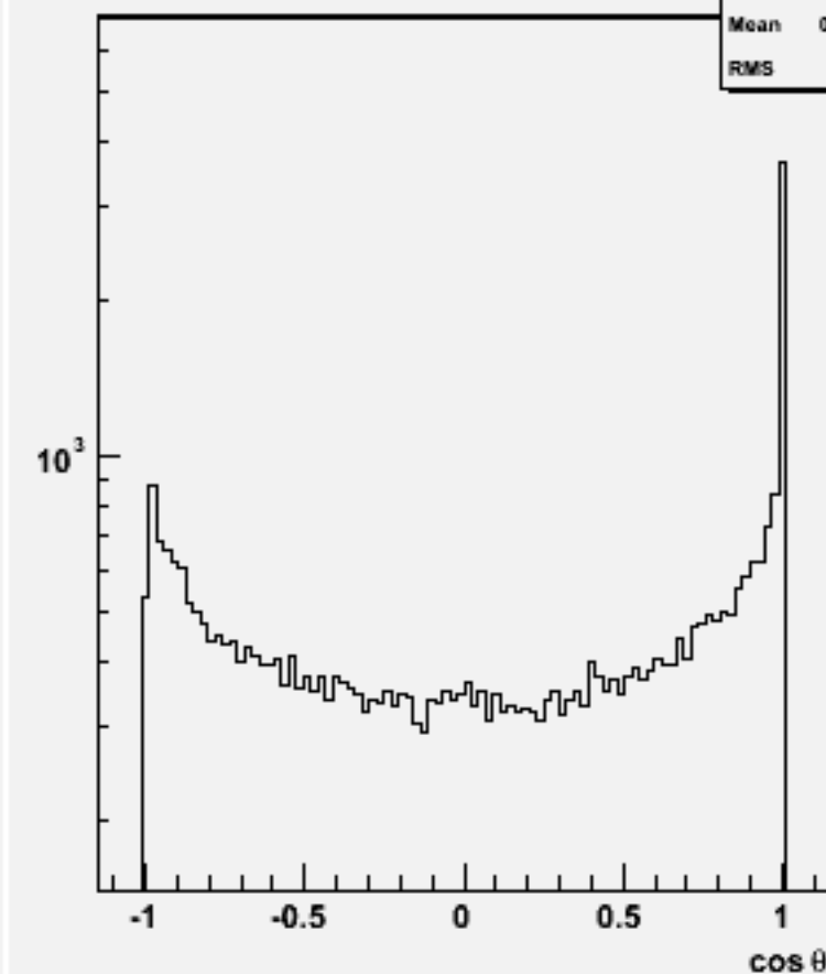
Jet cos \theta (All jets)w102117 uuuubb_o
