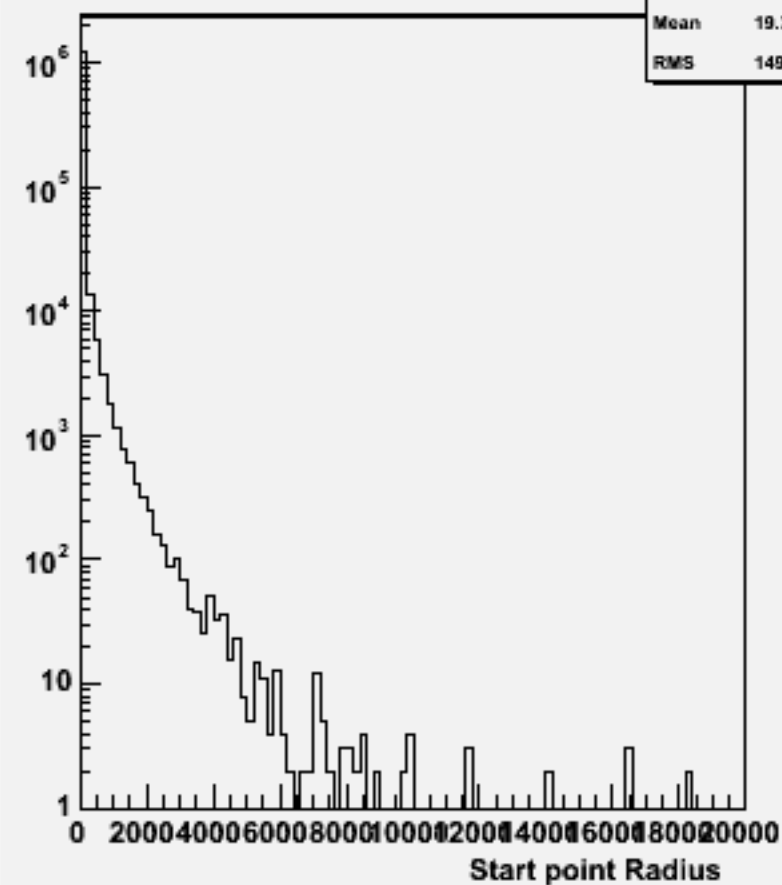
Start point R : w102117 uuuubb_o
