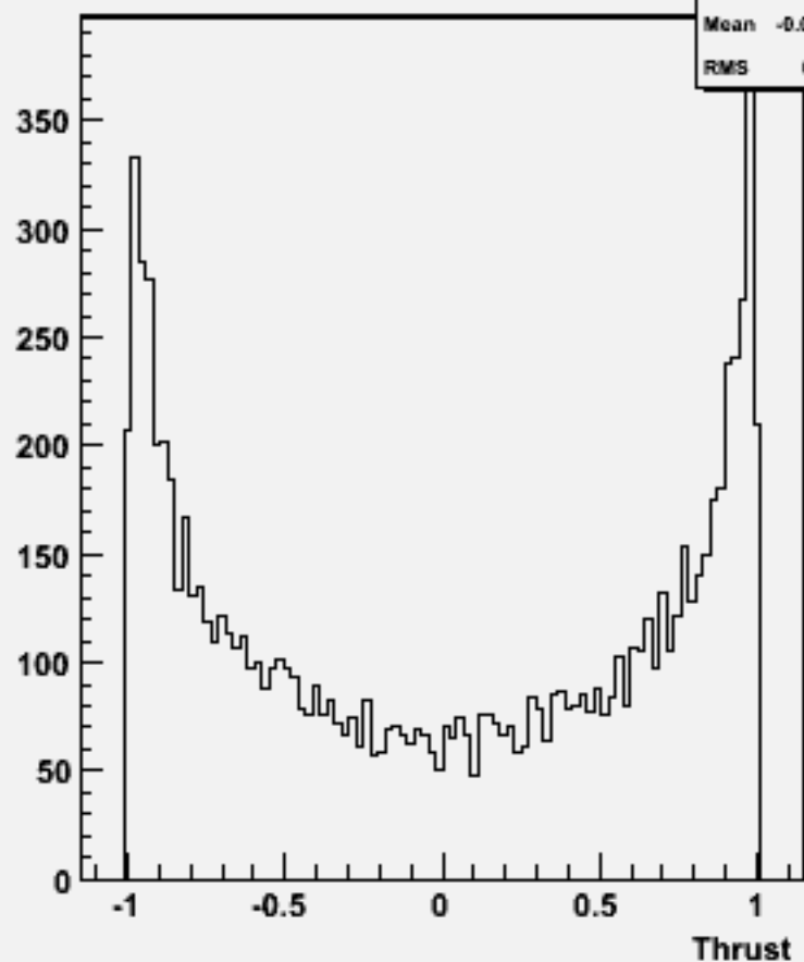
cos \Theta (thrust) w102117 uuuubb_o
