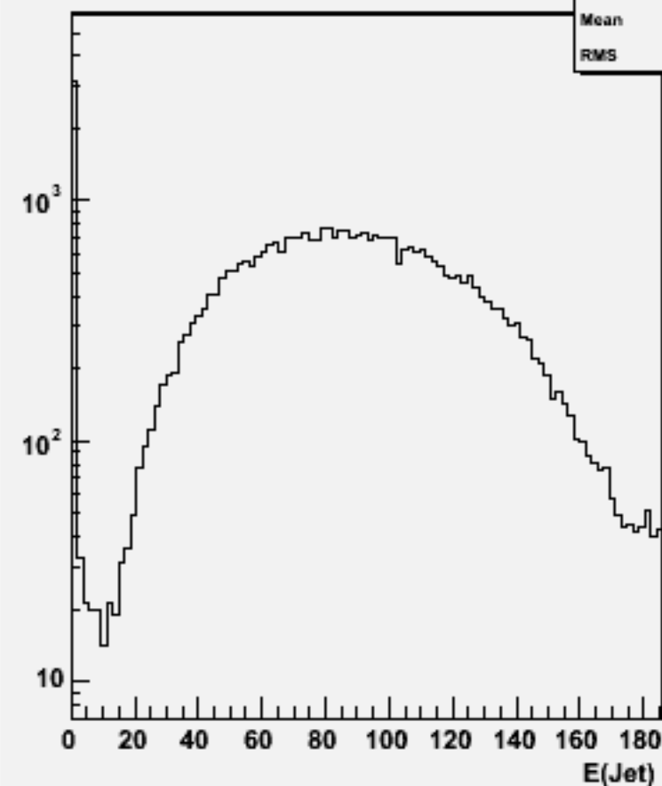
Jet energies(All jets)w102117 uuuubb_o
