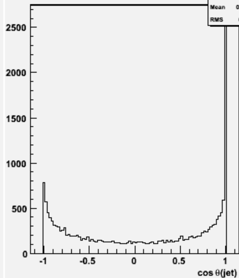
cos \Theta for 2-jets :w102117 uuuubb_o
