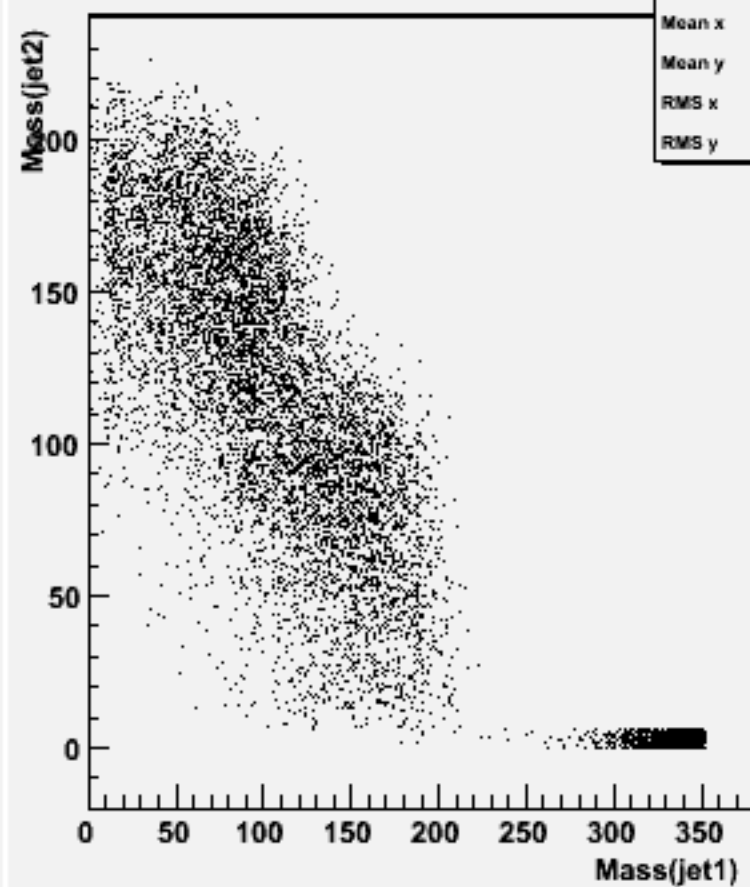
Jet mass for forced 2-jets : w102117 uuuubb_o
