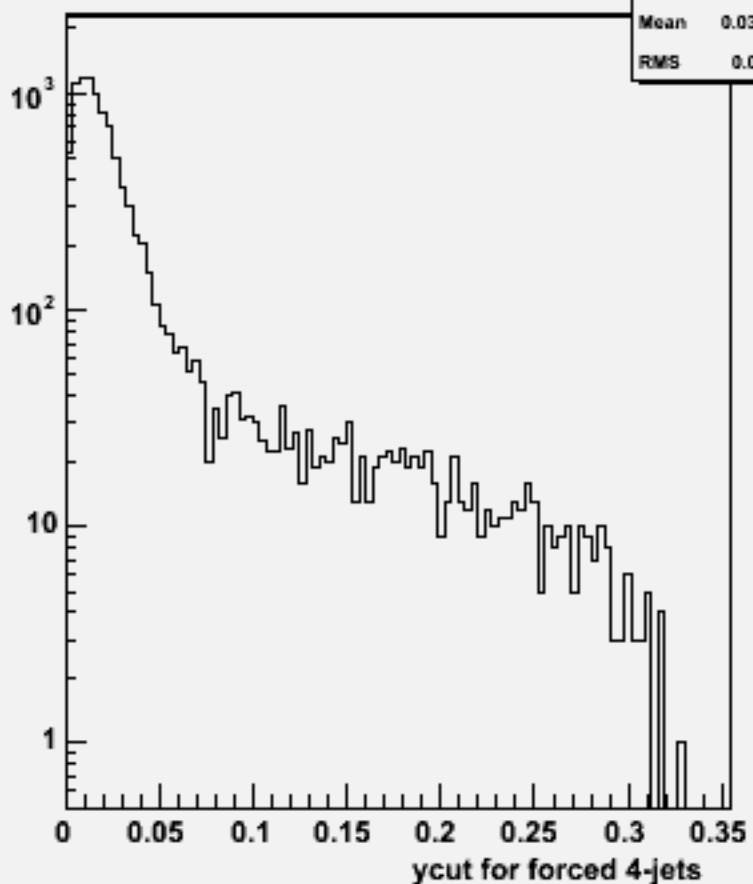
Ycut for 4-jets :w102117 uuuubb_o
