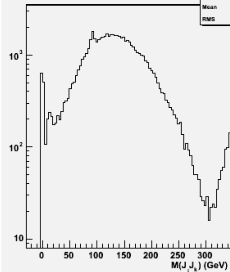
2jets mass(All comb)w102117 uuuubb_o
