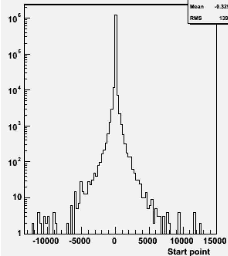
Start point Z : w102117 uuuubb_o
