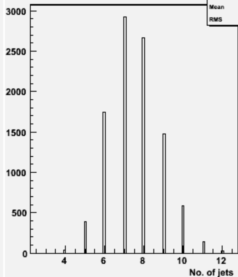
No. jets (ycut=0.001) : w102117 uuuubb_o
