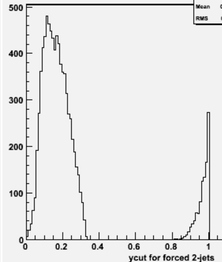
Ycut for 2-jets :w102117 uuuubb_o
