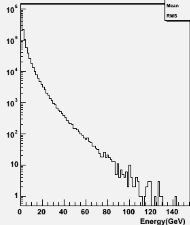
Start point R : w102117 uuuubb_o
