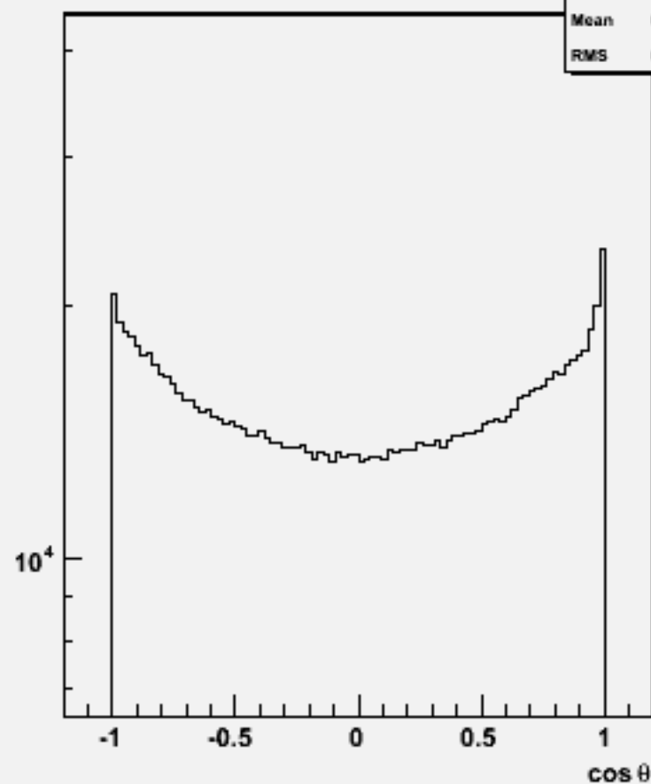
Particle cos \theta : w102116 uuuubb_o
