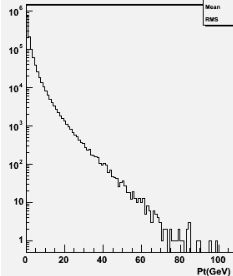
Start point Z : w102116 uuuubb_o
