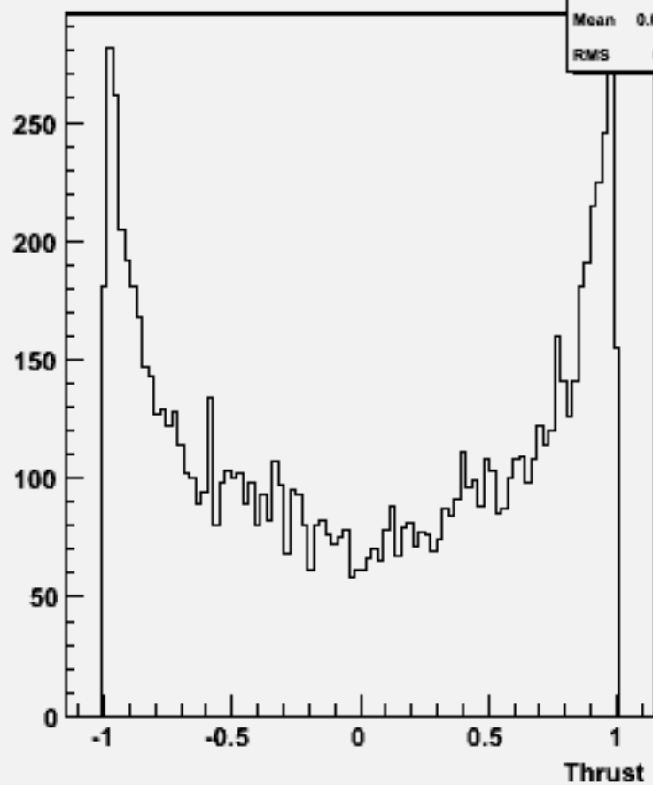
cos \Theta (thrust) w102116 uuubbb_o
