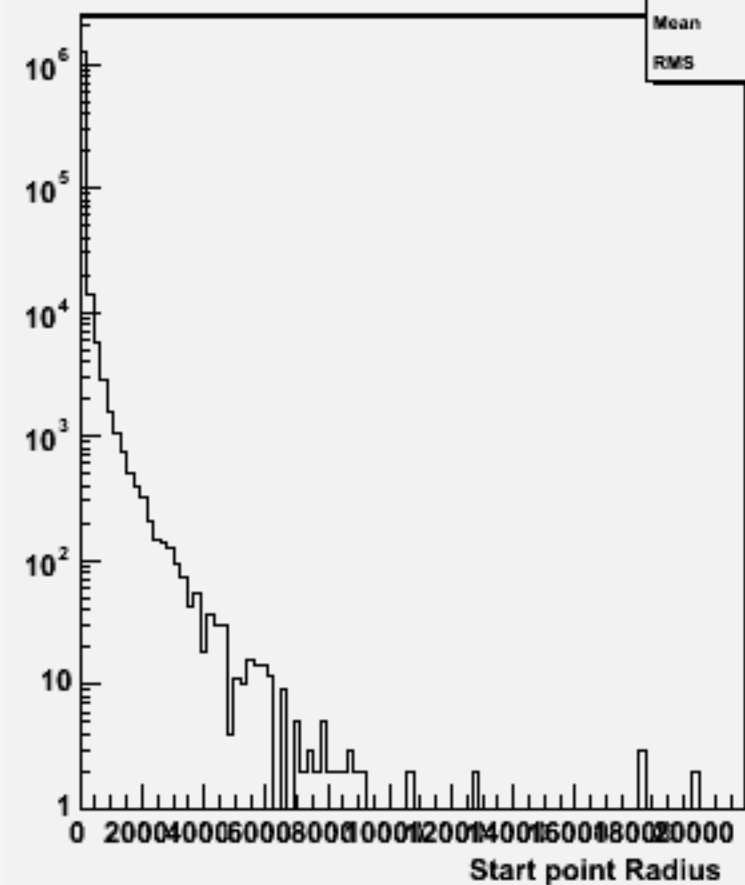
Start point R : w102116 uuuubb_o
