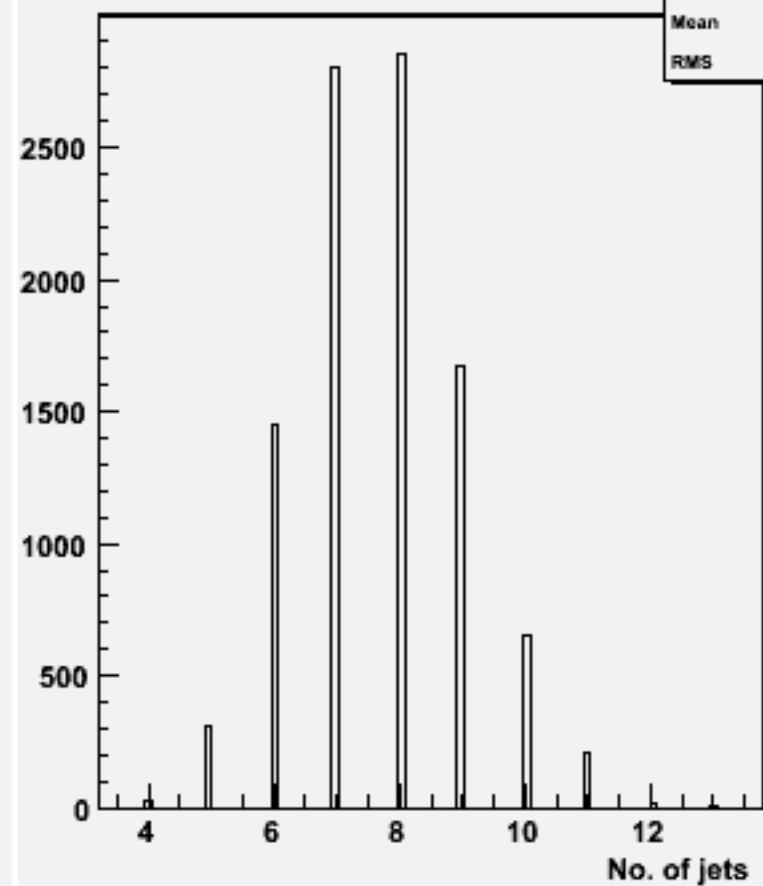
No. jets (ycut=0.001) : w102116 uuubbb_o
