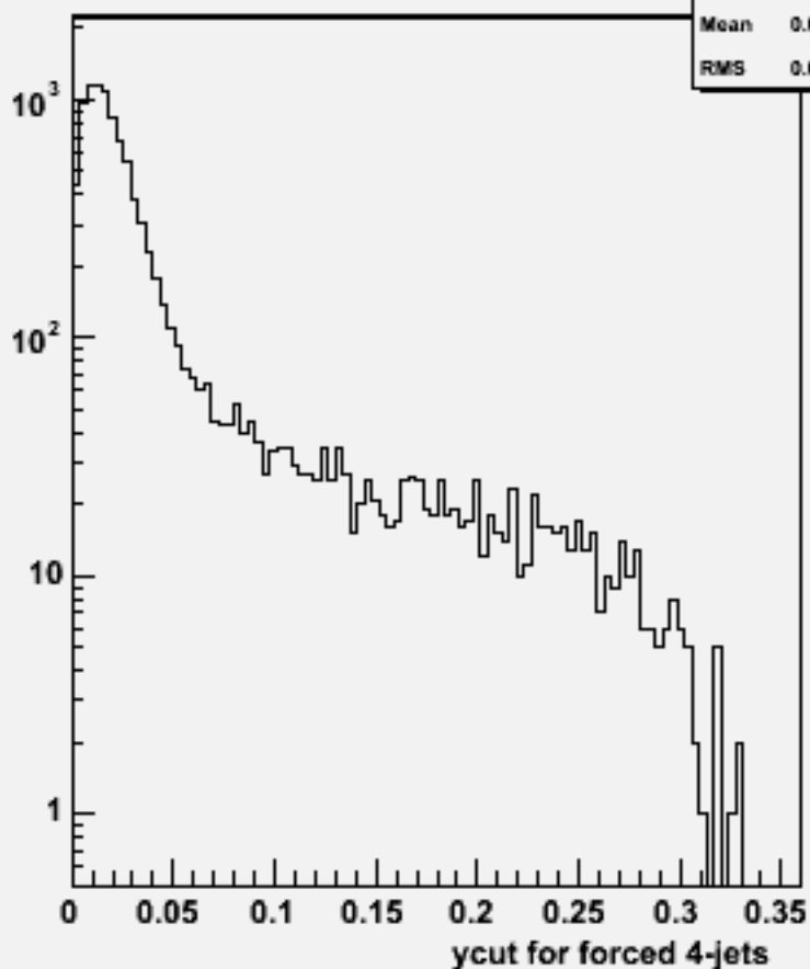
Ycut for 4-jets :w102116 uuuubb_o
