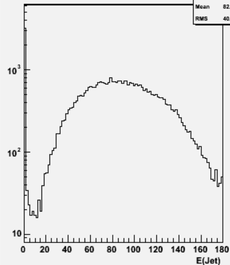
Jet energies(All jets)w102116 uuuubb_o
