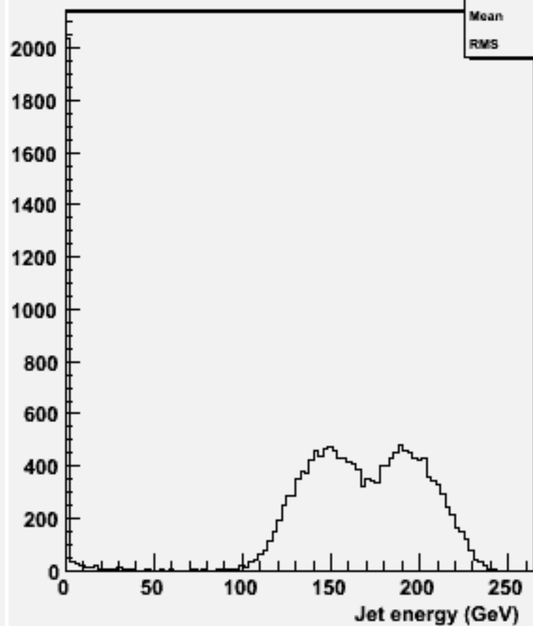
energy for 2-jets :w102116 uuubbb_o
