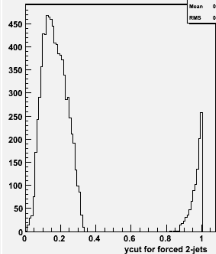
Ycut for 2-jets :w102116 uuubbb_o
