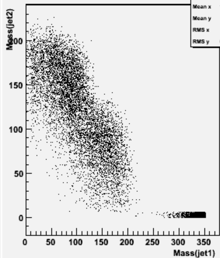
Jet mass for forced 2-jets : w102116 uuubbb_o
