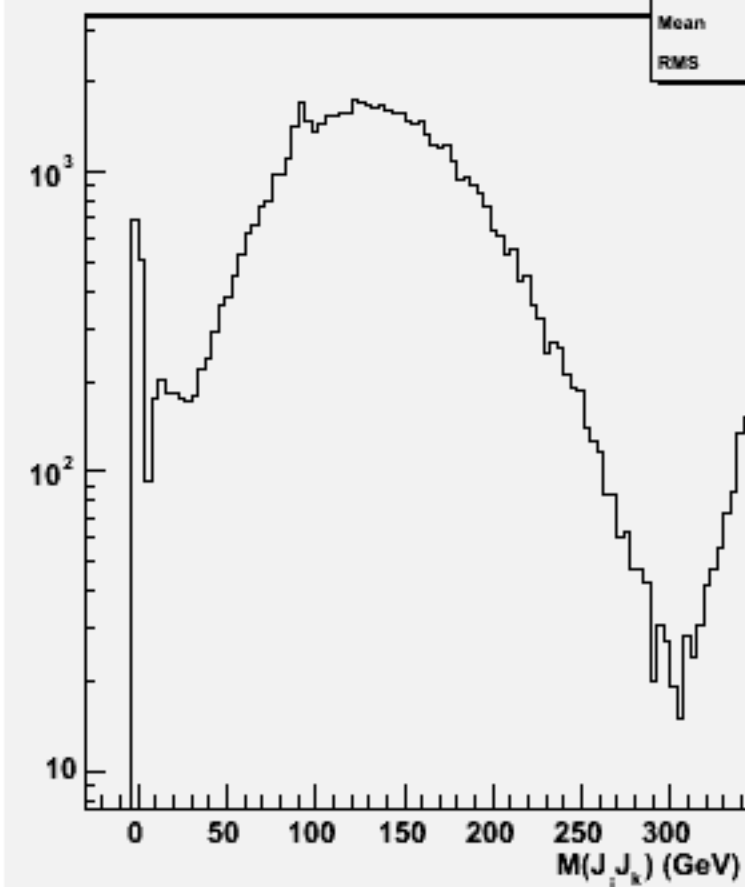
2jets mass(All comb)w102116 uuuubb_o
