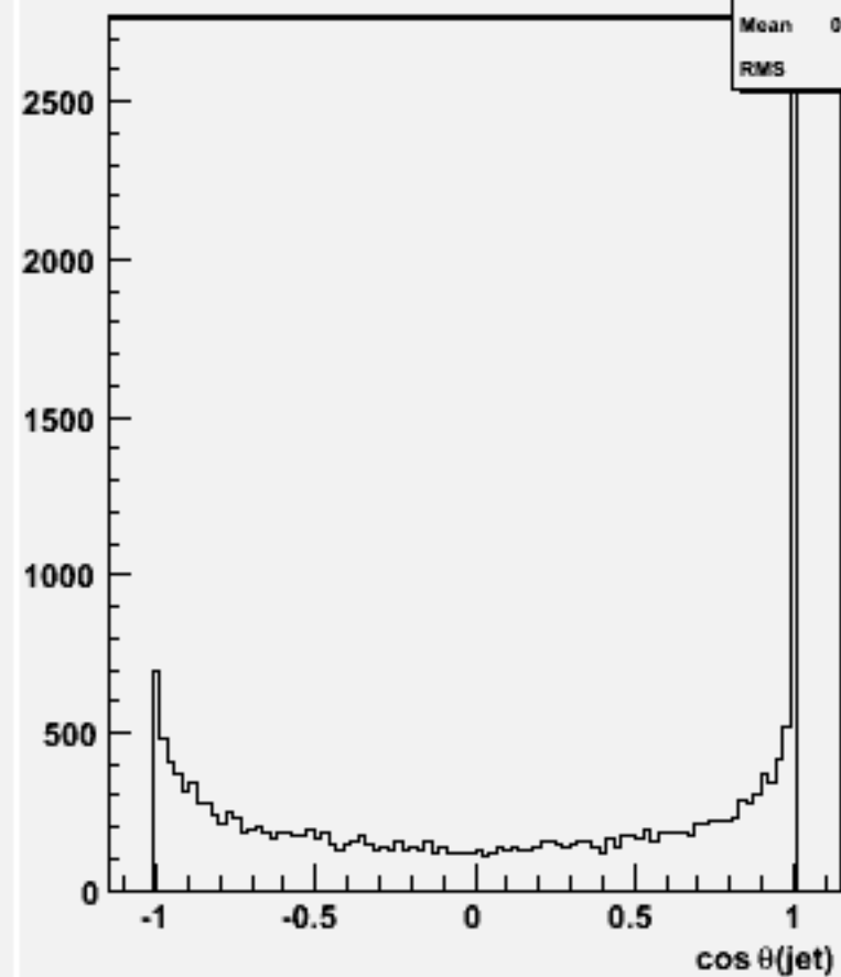
cos \theta for 2-jets :w102116 uuubbb_o
