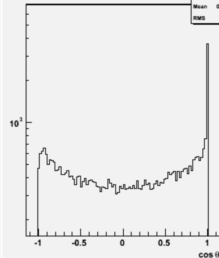
Jet cos \theta (All jets)w102116 uuuubb_o
