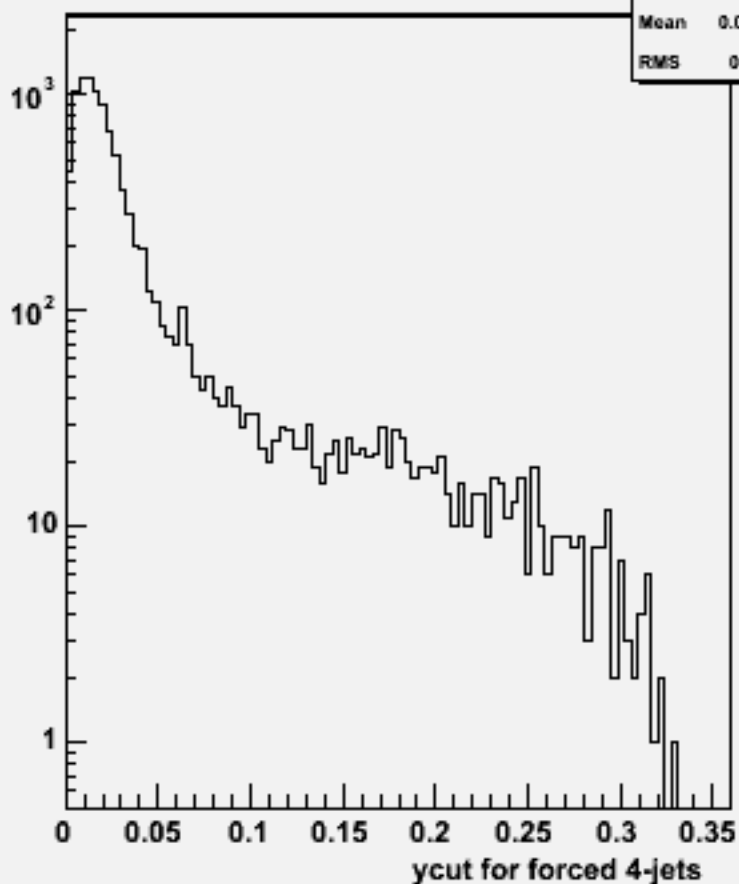
Ycut for 4-jets :w102113 uuuuss_o
