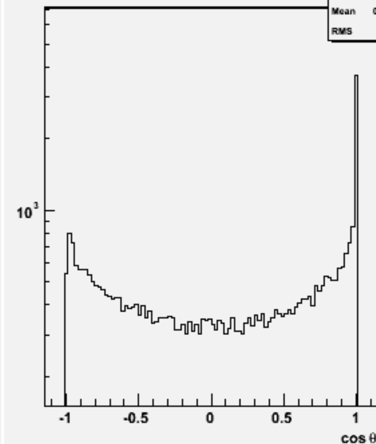
Jet cos \theta (All jets)w102113 uuuuss_o
