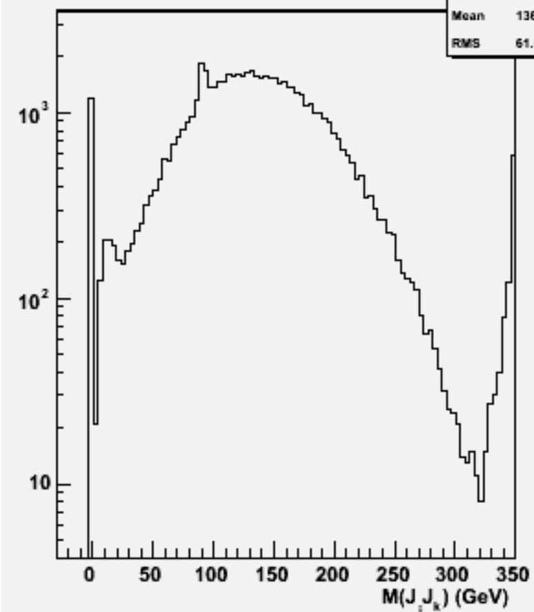
2jets mass(All comb)w102113 uuuuss_o
