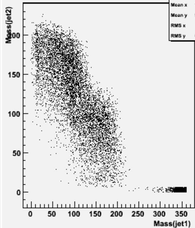
Jet mass for forced 2-jets : w102113 uuuuss_o
