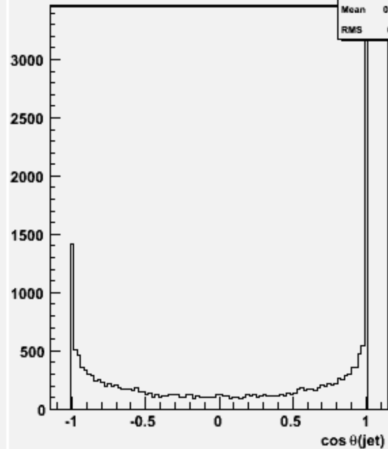
cos \theta for 2-jets :w102113 uuuuss_o
