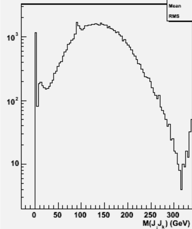
2jets mass(All comb)w102112 uuuuss_o
