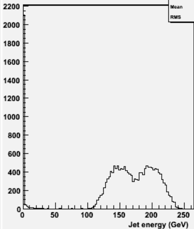
energy for 2-jets :w102112 uuuuss_o
