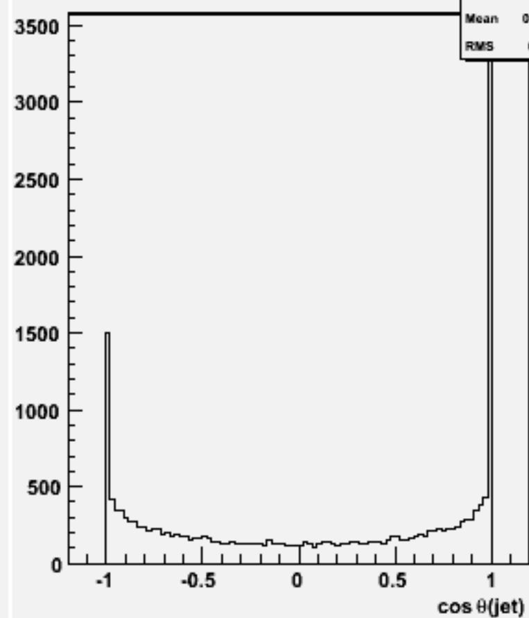
cos \theta for 2-jets :w102112 uuuuss_o
