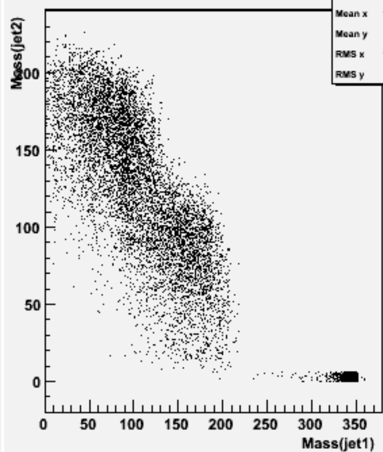
Jet mass for forced 2-jets : w102112 uuuuss_o
