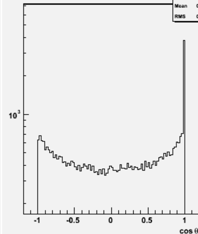
Jet cos \theta (All jets)w102112 uuuuss_o
