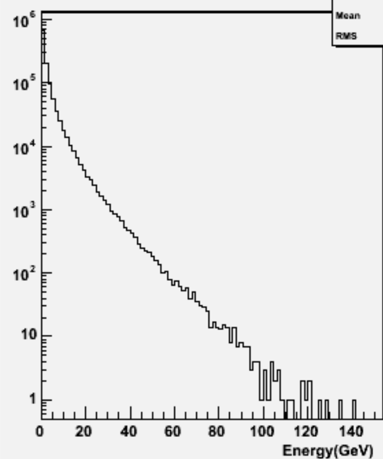
Particle Energy : w102112 uuuuss_o
