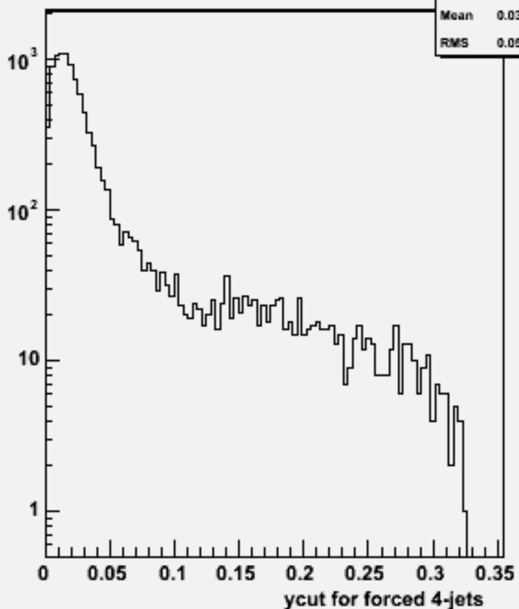
Ycut for 4-jets :w102112 uuuuss_o
