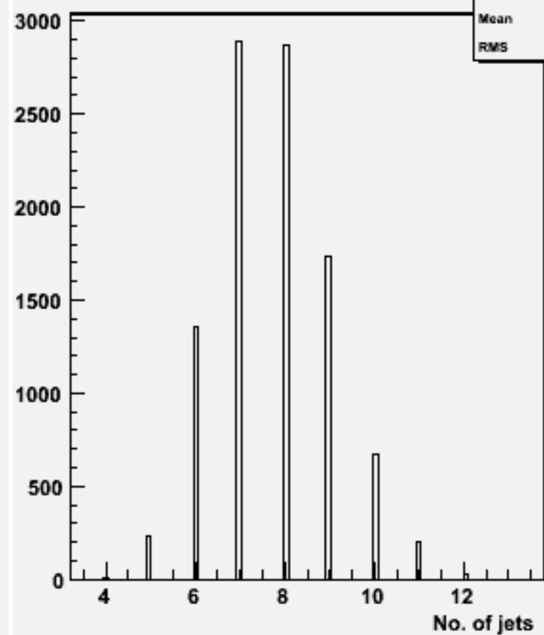
No. jets (ycut=0.001) : w102112 uuuuss_o
