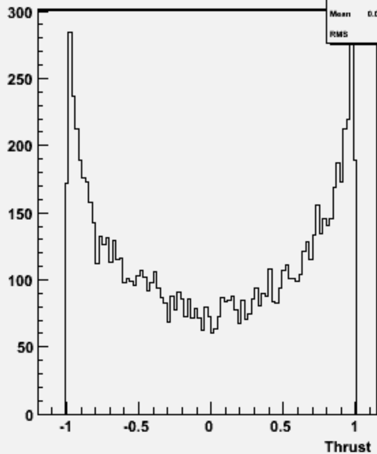
cos \Theta (thrust) w102112 uuuuss_o
