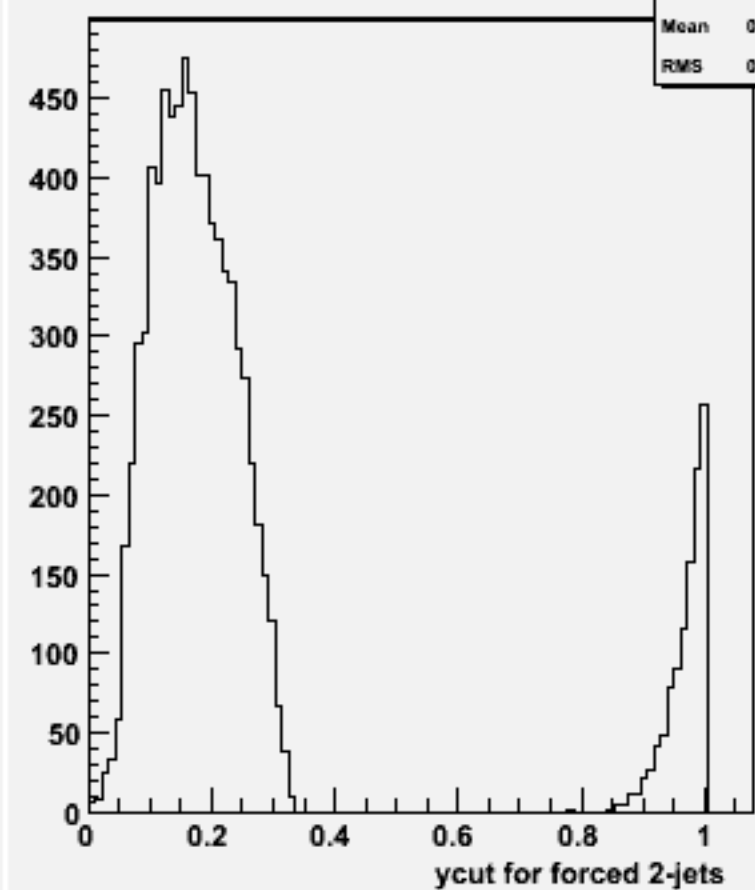
Ycut for 2-jets :w102112 uuuuss_o
