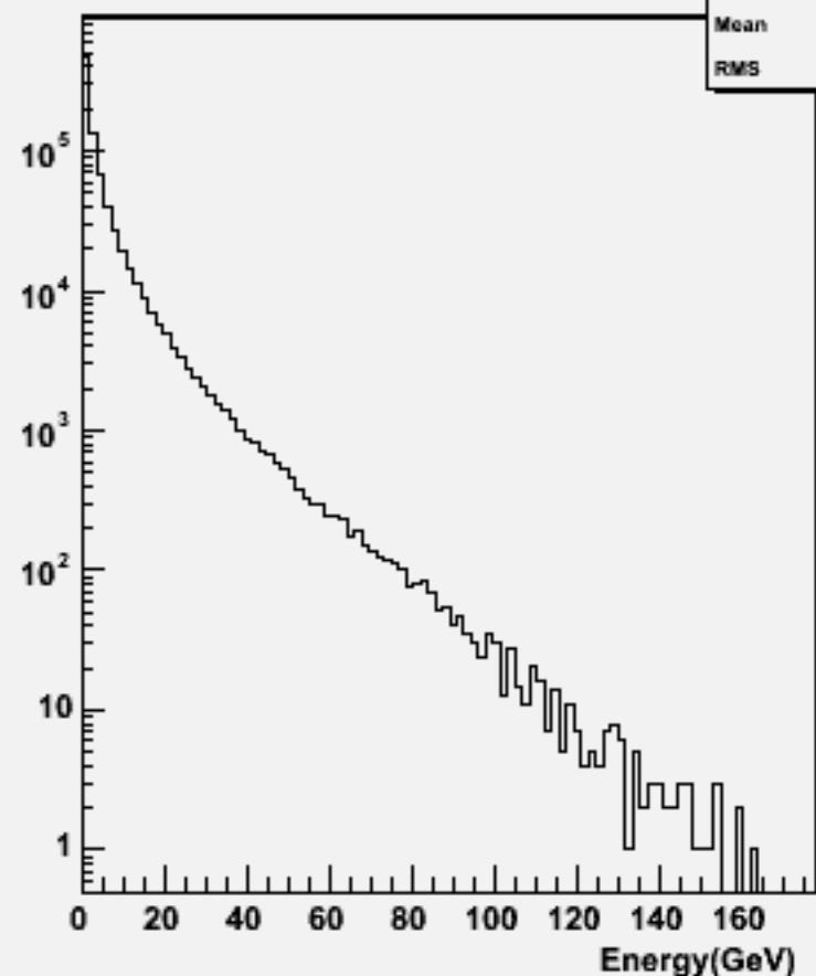
Particle Energy : w102109 uuuue3e3_o
