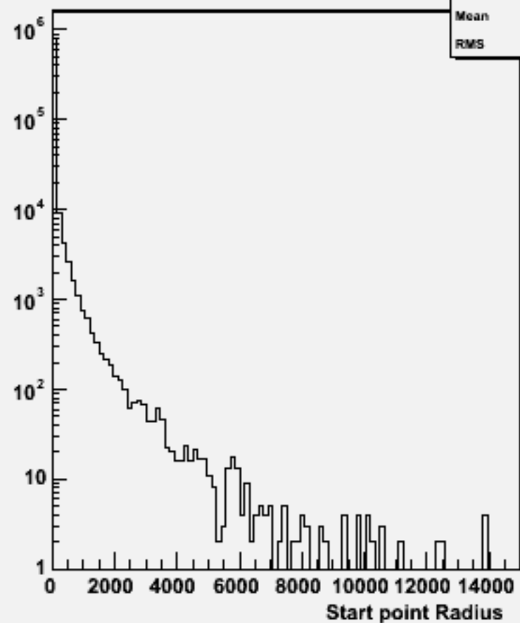
Start point R : w102109 uuuue3e3_o
