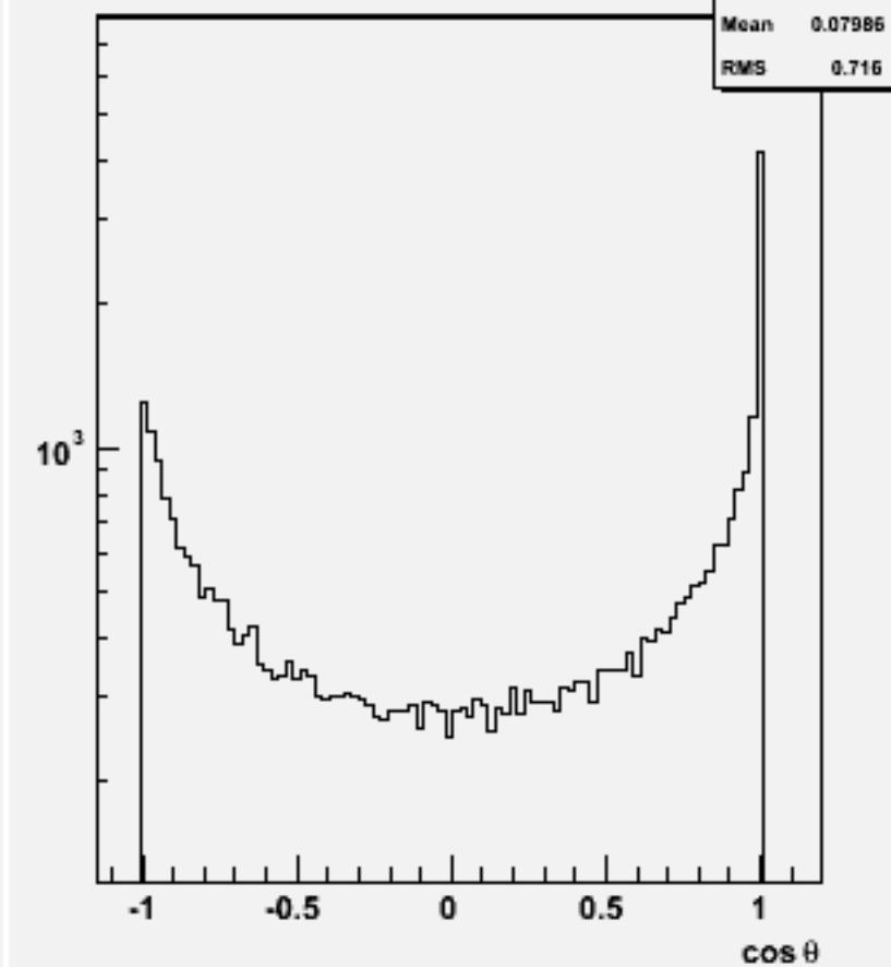
Jet cos \theta (All jets)w102109 uuuue3e3_o
