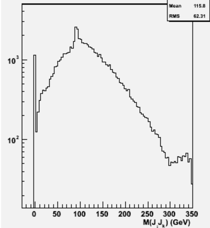
2jets mass(All comb)w102109 uuuue3e3_o
