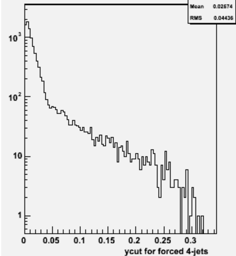
Ycut for 4-jets :w102109 uuuue3e3_o
