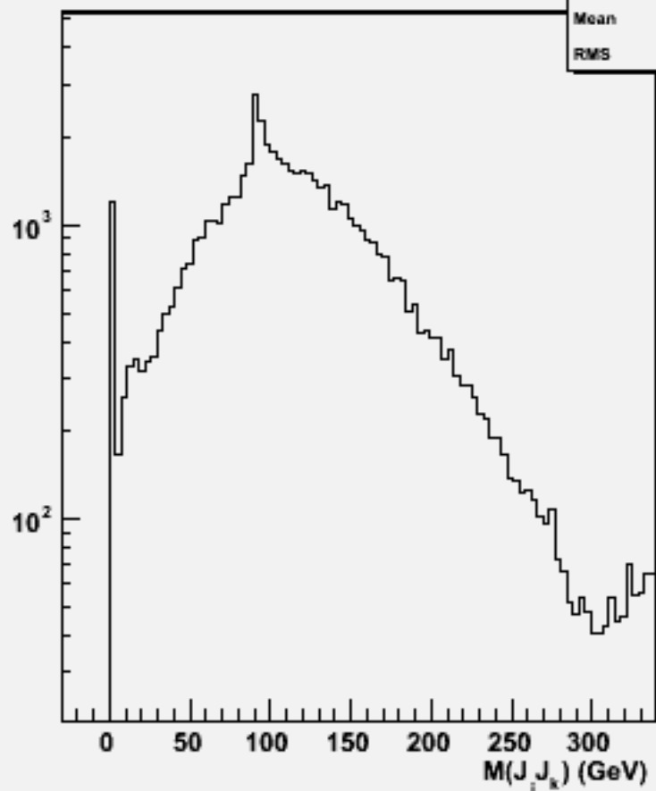
2jets mass(All comb)w102108 uuuue3e3_o
