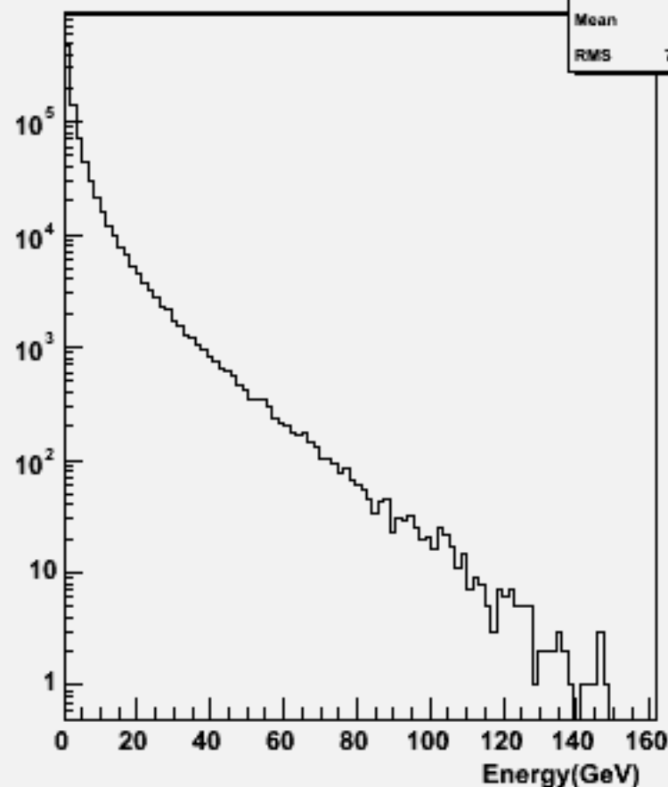
Particle Energy : w102108 uuuue3e3_o
