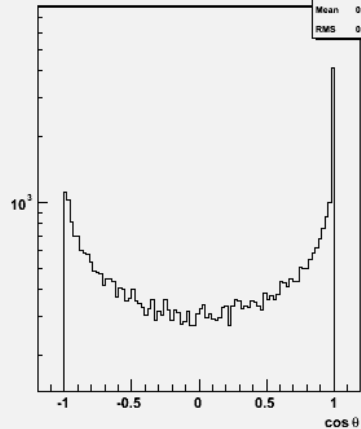
Jet cosθ (All jets)w102108 uuuue3e3_o
