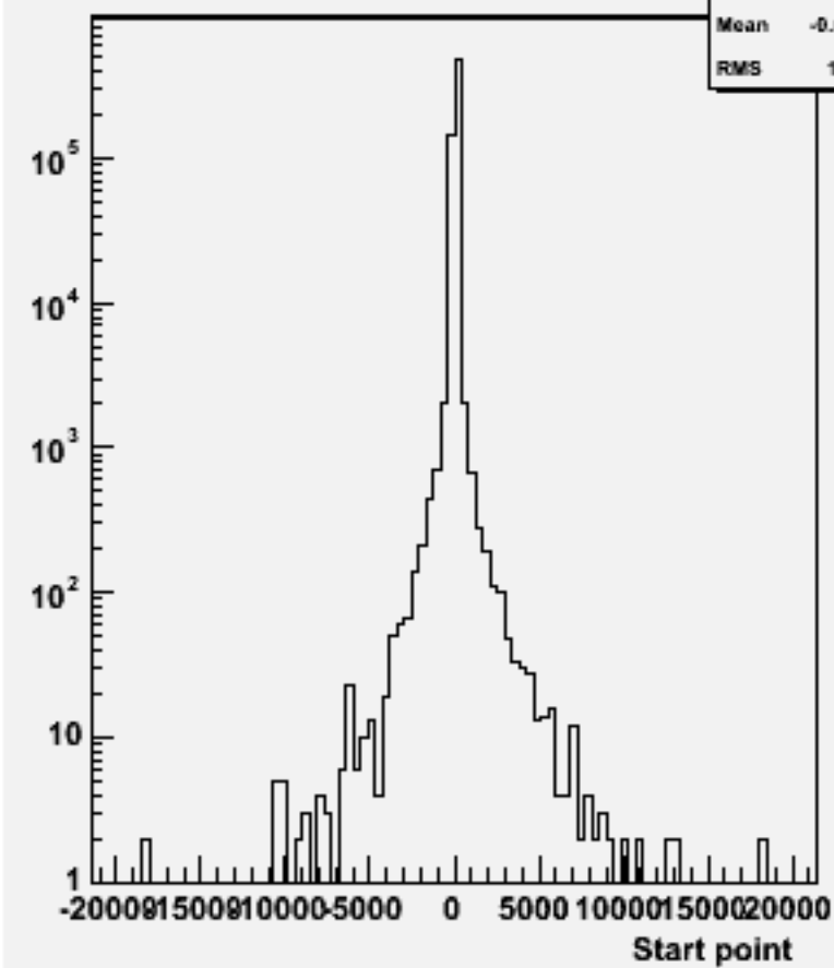
Start point Z : w102102 uuuue1e1_o
