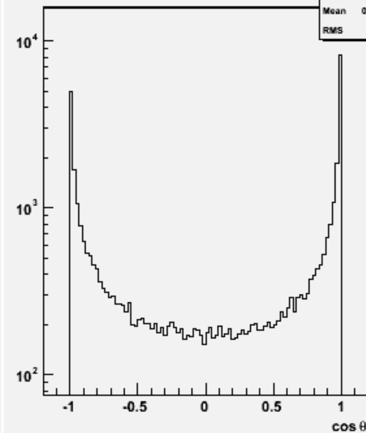
Jet cos \theta (All jets)w102102 uuuue1e1_o
