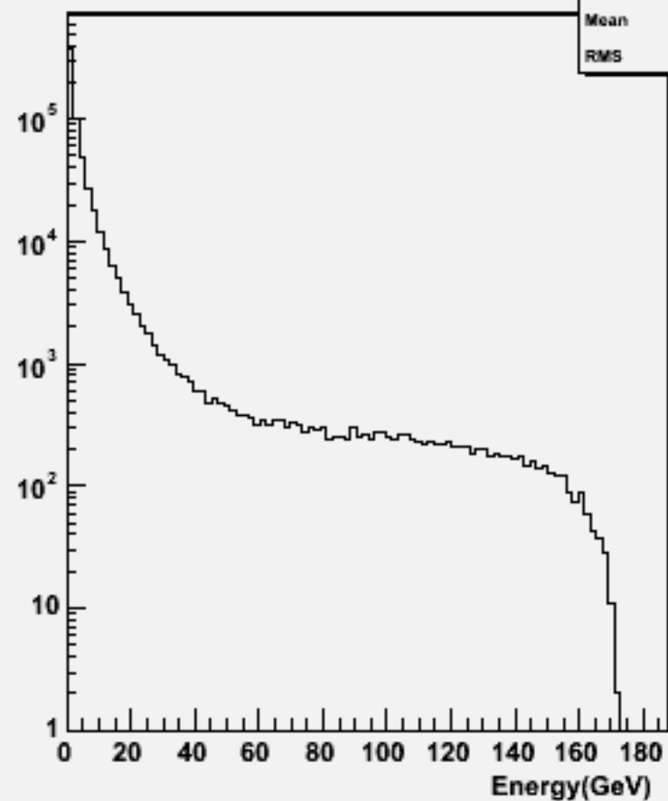
Particle Energy : w102102 uuuue1e1_o
