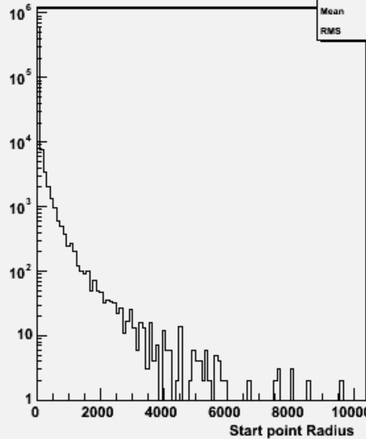
Start point R : w102102 uuuue1e1_o
