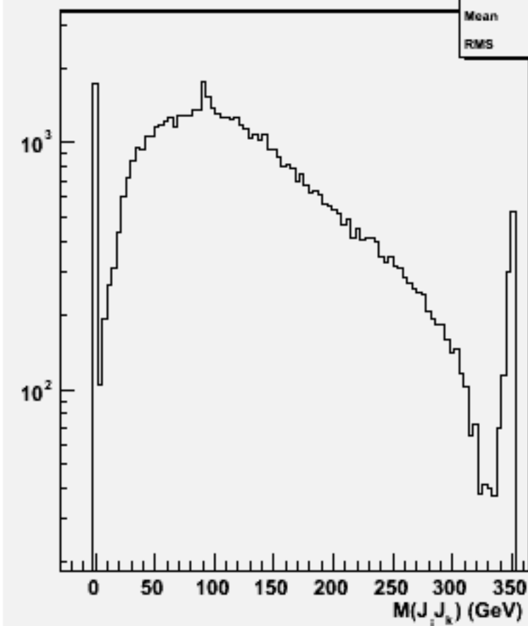
2jets mass(All comb)w102102 uuuue1e1_o
