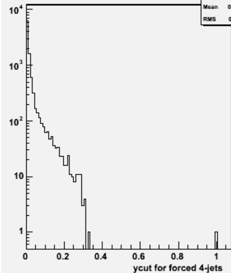
Ycut for 4-jets :w102102 uuuue1e1_o
