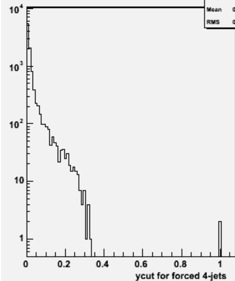
Ycut for 4-jets :w102101 uuuue1e1_o
