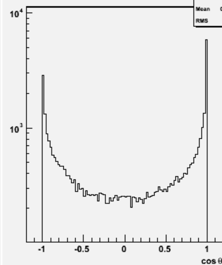
Jet cos \theta (All jets)w102101 uuuue1e1_o
