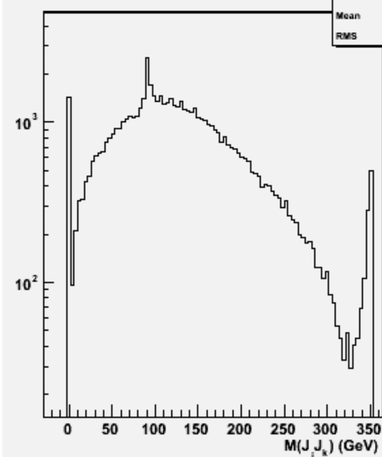
2jets mass(All comb)w102101 uuuue1e1_o
