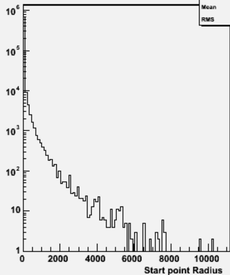
Start point R : w102101 uuuue1e1_o
