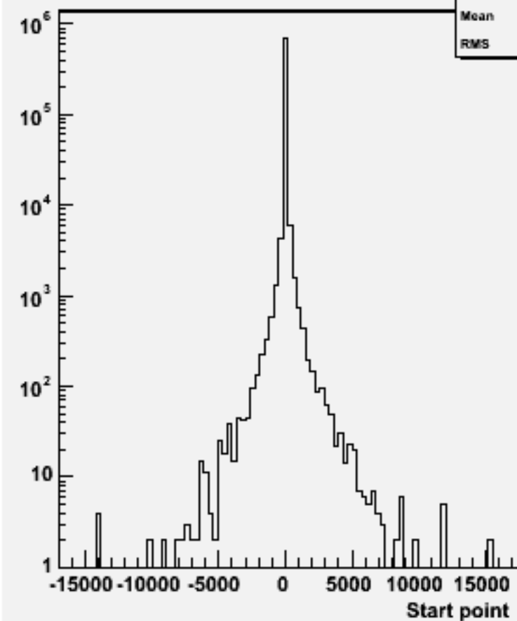
Start point Z : w102101 uuuue1e1_o
