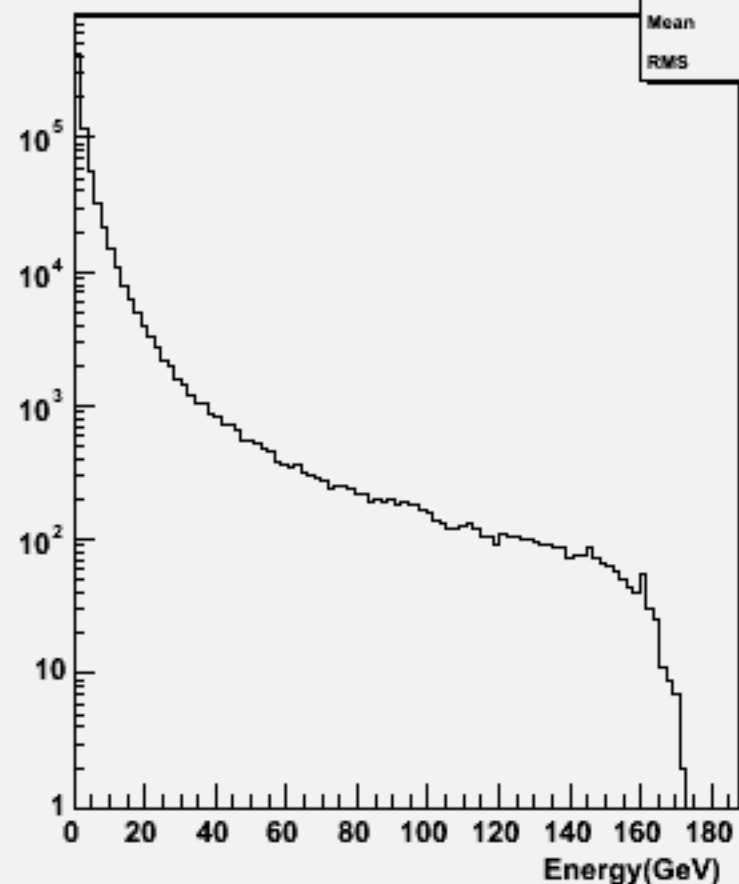
Particle Energy : w102101 uuuue1e1_o
