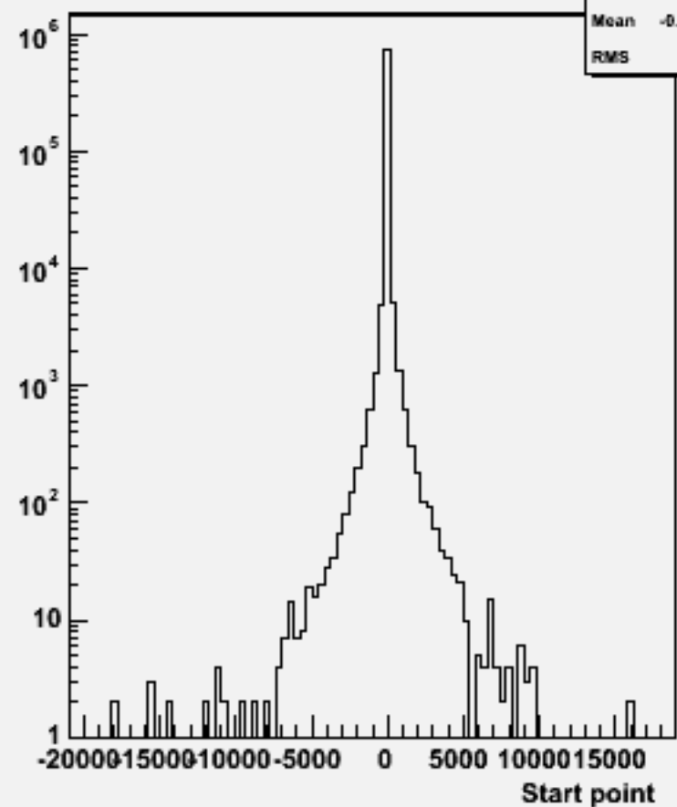
Start point Z : w102100 uuuue1e1_o
