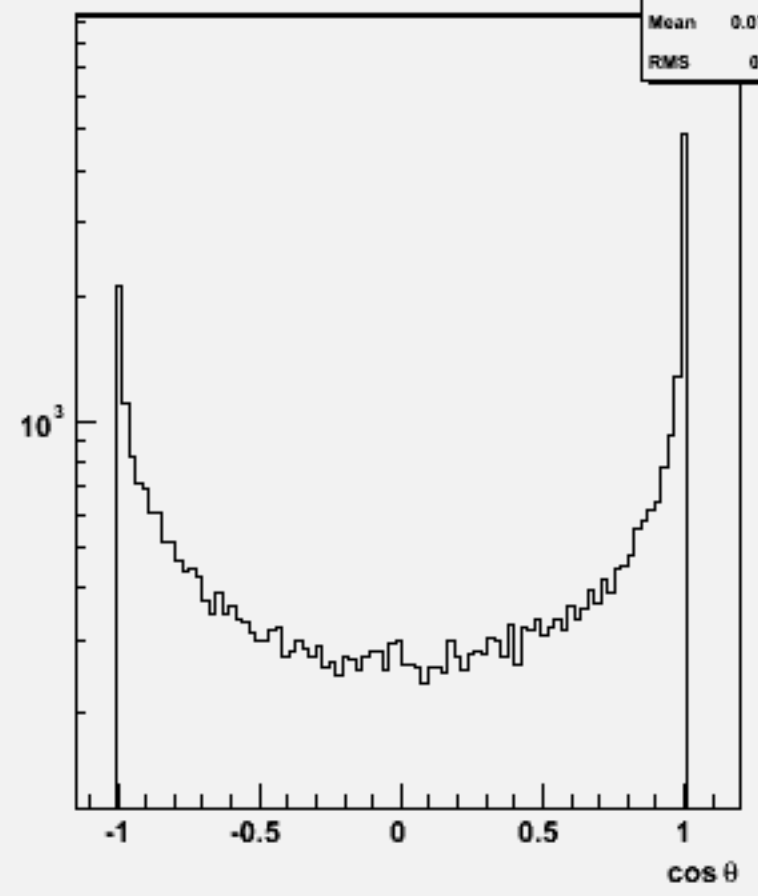
Jet cosθ (All jets)w102100 uuuue1e1_o
