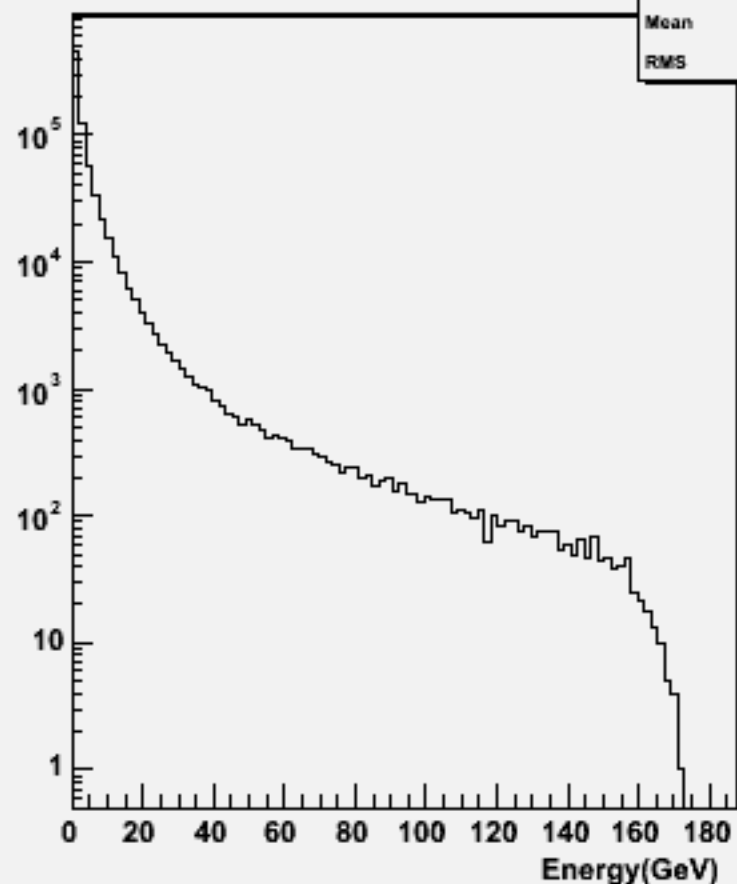
Particle Energy : w102100 uuuue1e1_o
