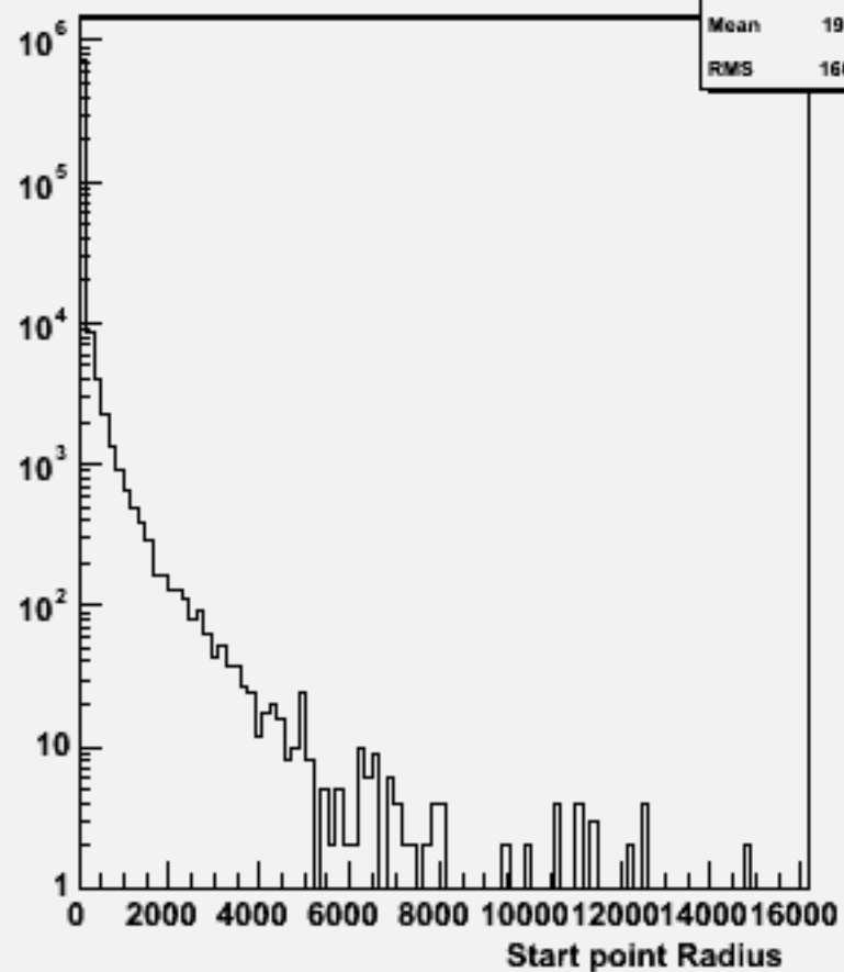
Start point R : w102100 uuuue1e1_o
