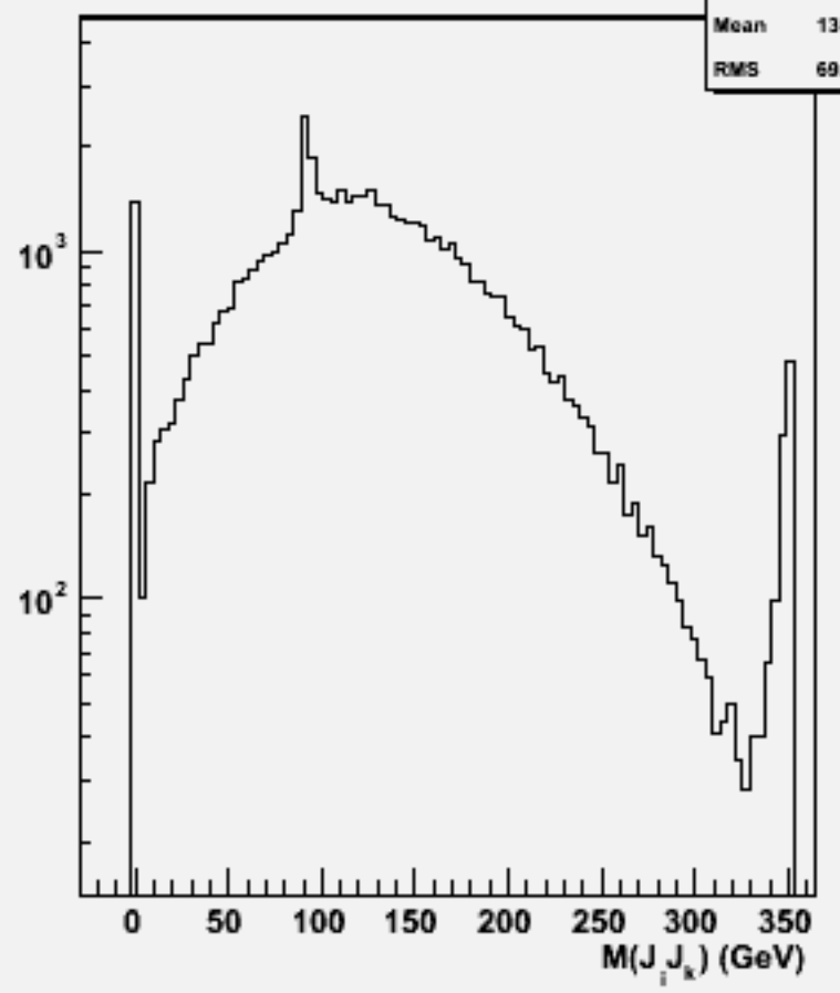
2jets mass(All comb)w102100 uuuue1e1_o
