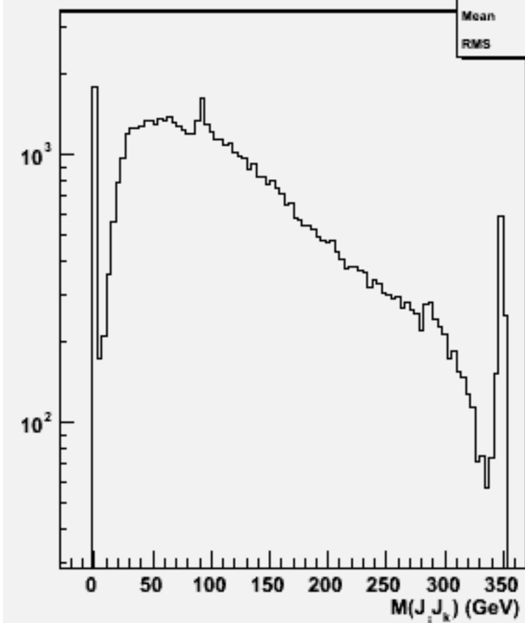
2jets mass(All comb)w102099 uuuue1e1_o
