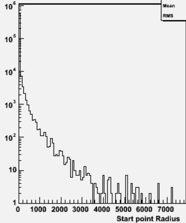
Start point R : w102099 uuuue1e1_o
