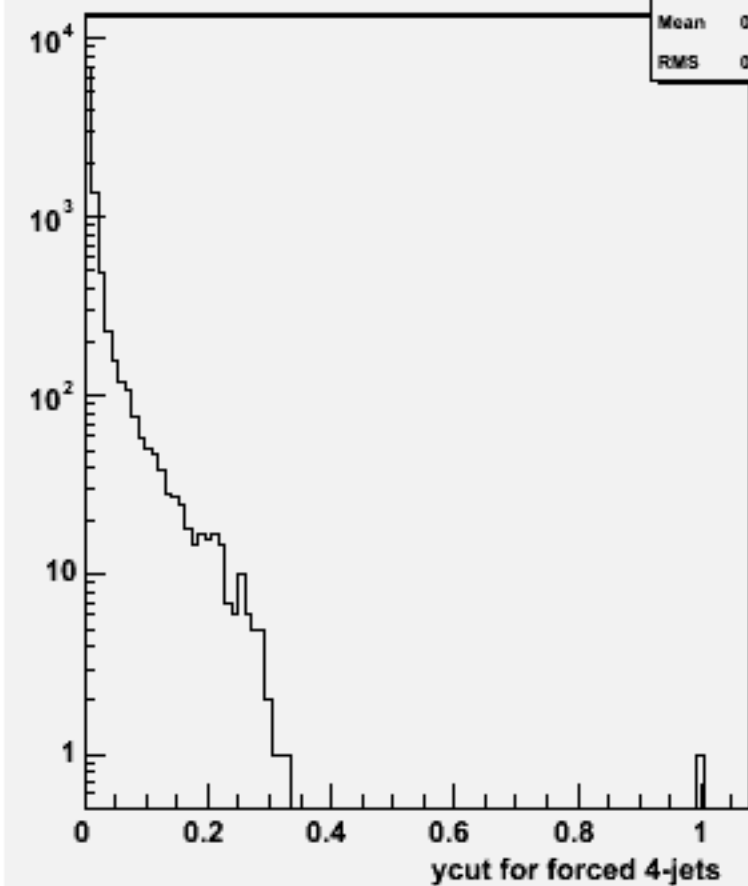
Ycut for 4-jets :w102099 uuuue1e1_o
