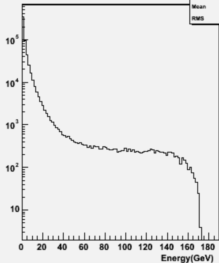
Particle Energy : w102099 uuuue1e1_o
