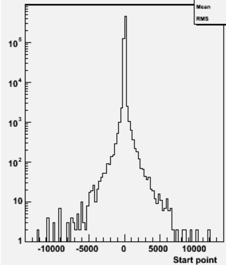
Start point Z : w102099 uuuue1e1_o
