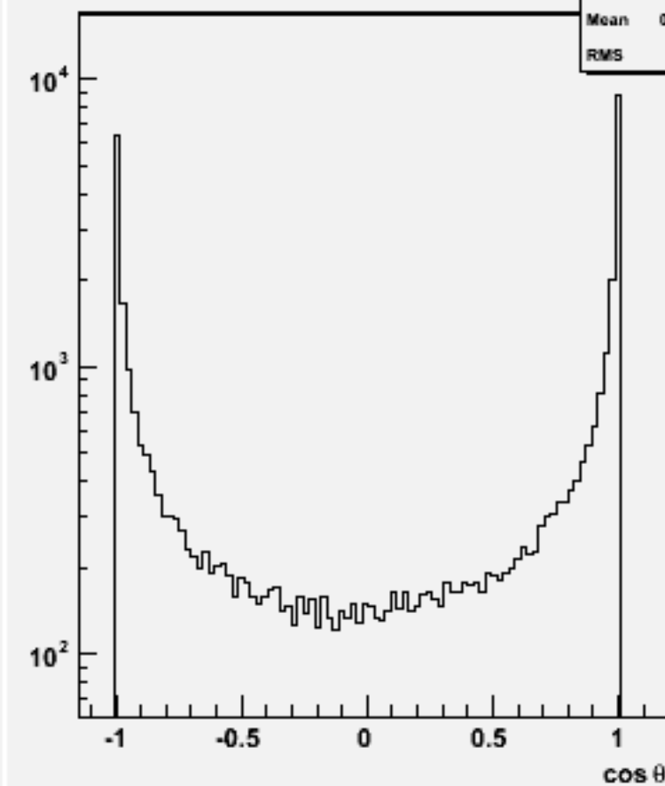
Jet cosθ (All jets)w102099 uuuue1e1_o
