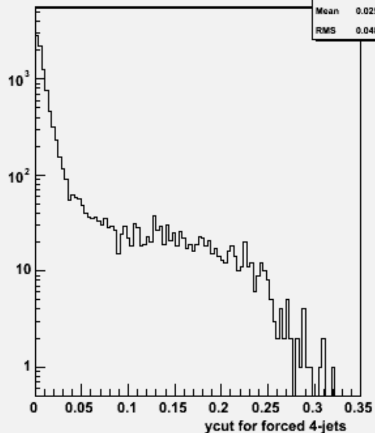
Ycut for 4-jets :w102097 n3n3ccbb_o
