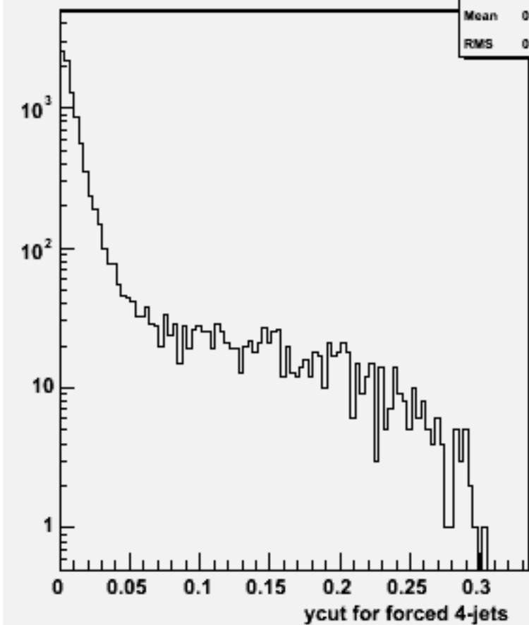
Ycut for 4-jets :w102096 n3n3ccbb_o
