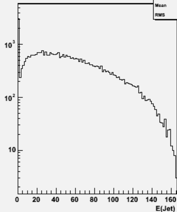
Jet energies(All jets)w102089 n3n3cce2e2_o
