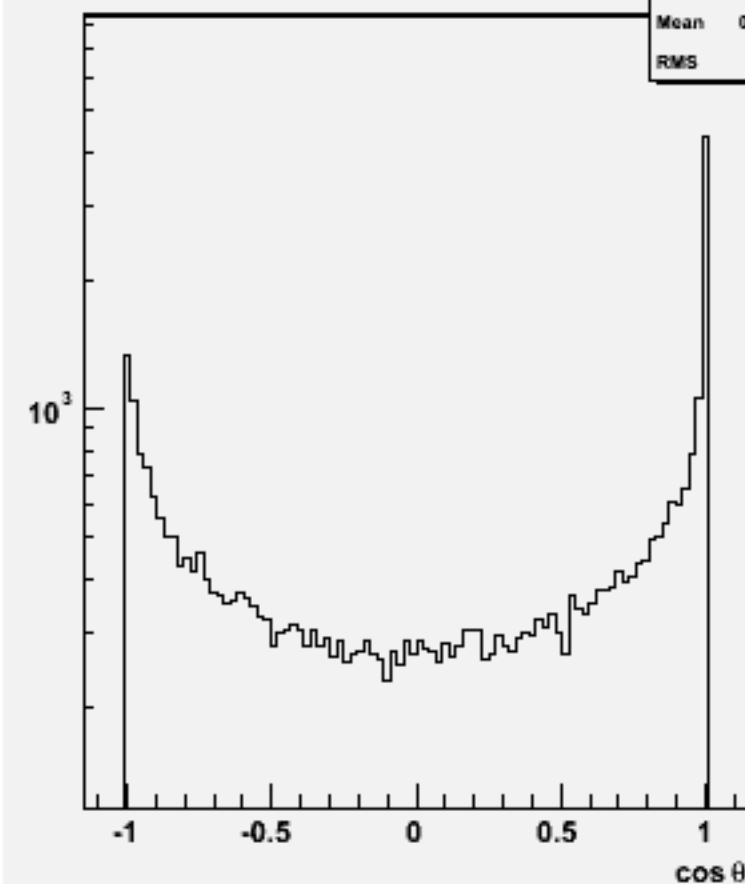
Jet cos \theta (All jets)w102089 n3n3cce2e2_o
