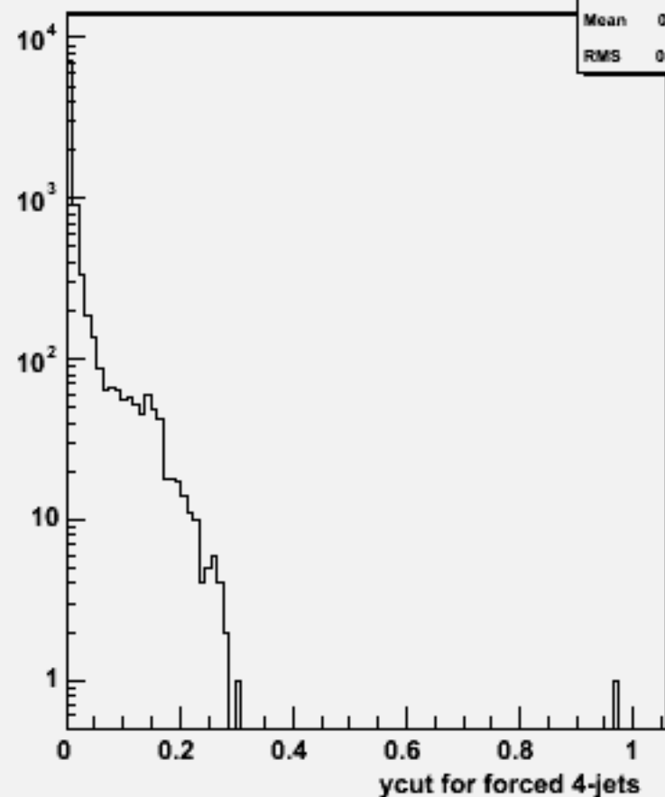
Ycut for 4-jets :w102089 n3n3cce2e2_o
