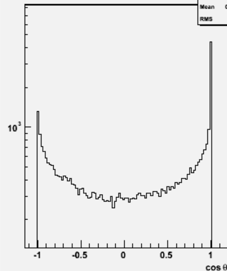
Jet cos \theta (All jets)w102088 n3n3cce2e2_o
