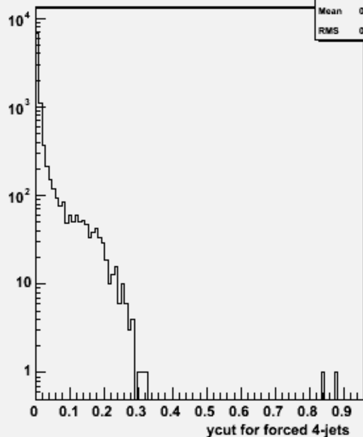
Ycut for 4-jets :w102088 n3n3cce2e2_o
