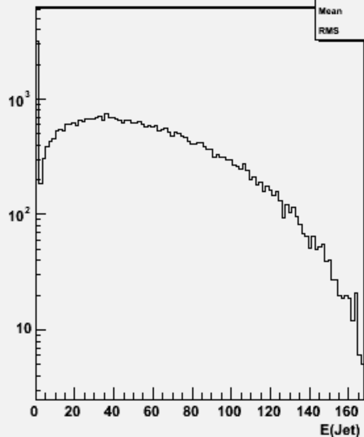
Jet energies(All jets)w102088 n3n3cce2e2_o
